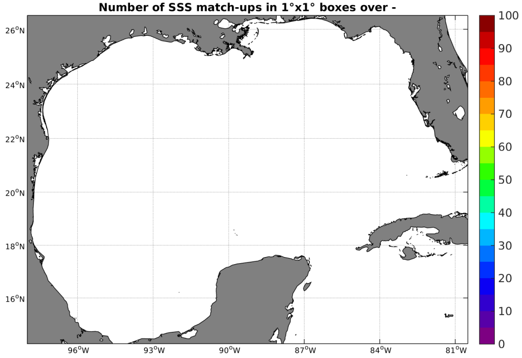
Figure 4: Number of SSS match-ups between TSG-LEGOS-DM SSS and the AQUARIUS-L2-JPL-V4 SSS product for the Gulf of Mexico Pi-MEP region over 1°x1° boxes and for the full satellite product period.
