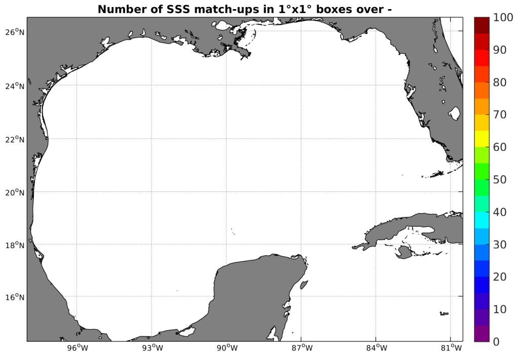
Figure 4: Number of SSS match-ups between TSG-GOSUD-Sailing-ship SSS and the AQUARIUS-L2-JPL-V4 SSS product for the Gulf of Mexico Pi-MEP region over 1^\circ \times 1^\circ boxes and for the full satellite product period.
