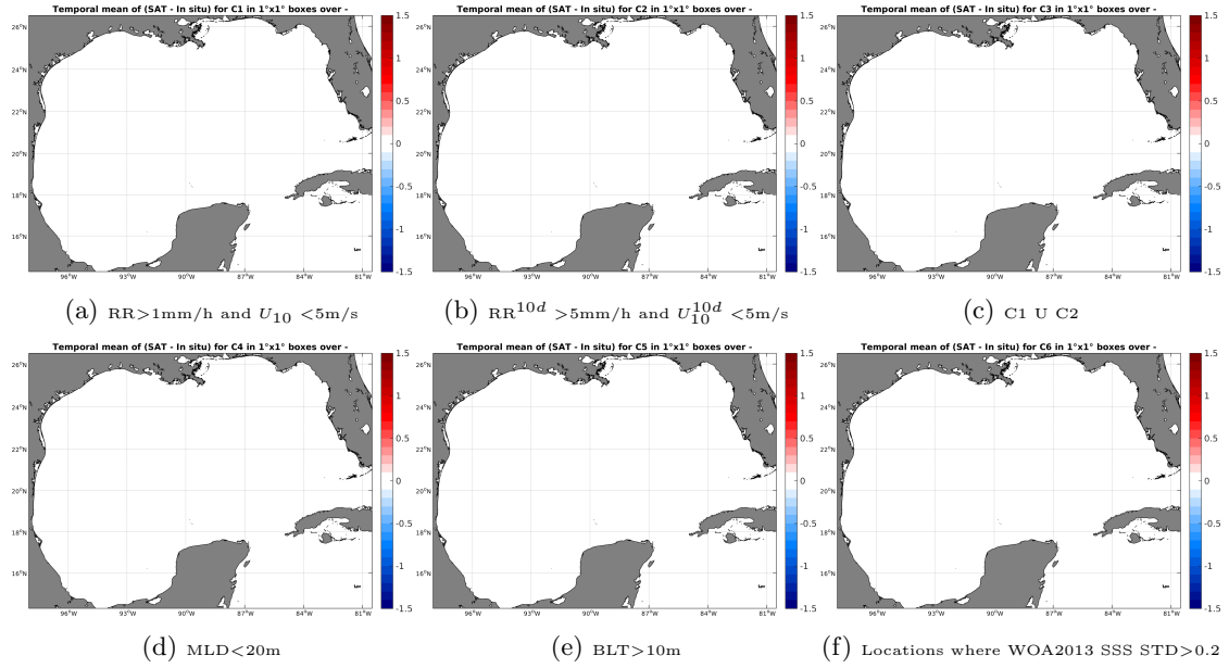
Figure 12: Temporal mean gridded over spatial boxes of size 1^\circ \times 1^\circ of \Delta SSS (AQUARIUS-L2-JPL-V4 - Sea mammals) for 6 different subdatasets corresponding to: RR > 1\text{mm/h} and U_{10} < 5\text{m/s} (a), RR^{10d} > 5\text{mm/h} and U_{10}^{10d} < 5\text{m/s} (b), C1 \cup C2 (c), MLD < 20\text{m} (d), BLT > 10\text{m} (e), Locations where WOA2013 SSS STD > 0.2 (f).
