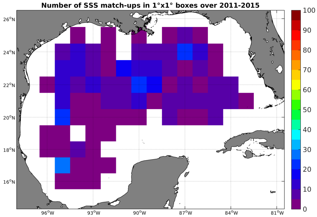
Figure 4: Number of SSS match-ups between Argo SSS and the AQUARIUS-L2-JPL-V4 SSS product for the Gulf of Mexico Pi-MEP region over 1^\circ \times 1^\circ boxes and for the full satellite product period.
