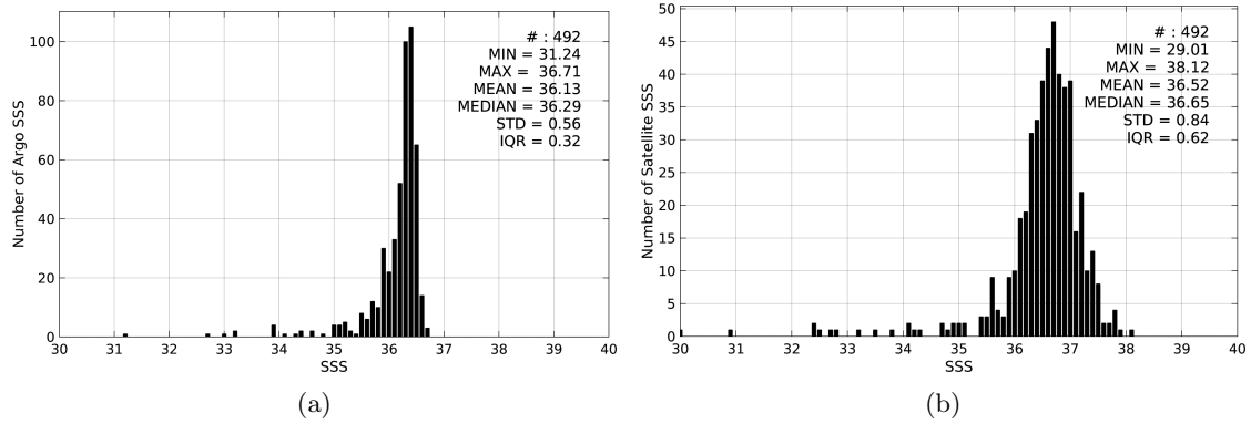
Figure 2: Histograms of SSS from Argo (a) and AQUARIUS-L2-JPL-V4 (b) considering all match-up pairs per bins of 0.1 over the Gulf of Mexico Pi-MEP region and for the full satellite product period.
