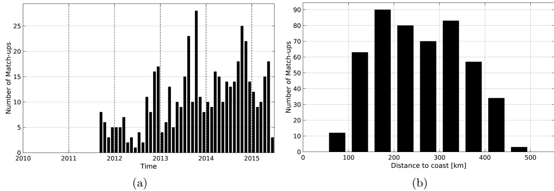
Figure 1: Number of match-ups between Argo and AQUARIUS-L2-JPL-V4 SSS as a function of time (a) and as function of the distance to coast (b) over the Gulf of Mexico Pi-MEP region and for the full satellite product period.
