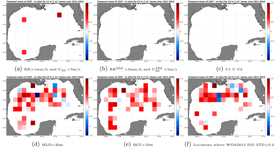
Figure 12: Temporal mean gridded over spatial boxes of size 1^\circ \times 1^\circ of \Delta\text{SSS} (AQUARIUS-L2-JPL-V4 - Argo) for 6 different subdatasets corresponding to: \text{RR} > 1\text{mm/h} and U_{10} < 5\text{m/s} (a), \text{RR}^{10d} > 5\text{mm/h} and U_{10}^{10d} < 5\text{m/s} (b), C1 U C2 (c), \text{MLD} < 20\text{m} (d), \text{BLT} > 10\text{m} (e), Locations where WOA2013 SSS STD > 0.2 (f).
