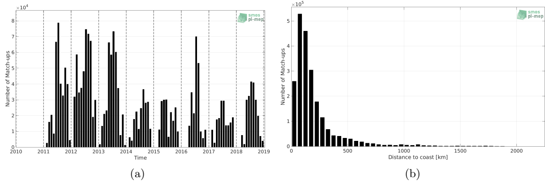
Figure 1: Number of match-ups between TSG (SAMOS) and SMOS and SMAP SSS L4 OI v1 - 7 Days (LOPS) SSS as a function of time (a) and as function of the distance to coast (b) over the Gulf Stream Pi-MEP region and for the full satellite product period.
