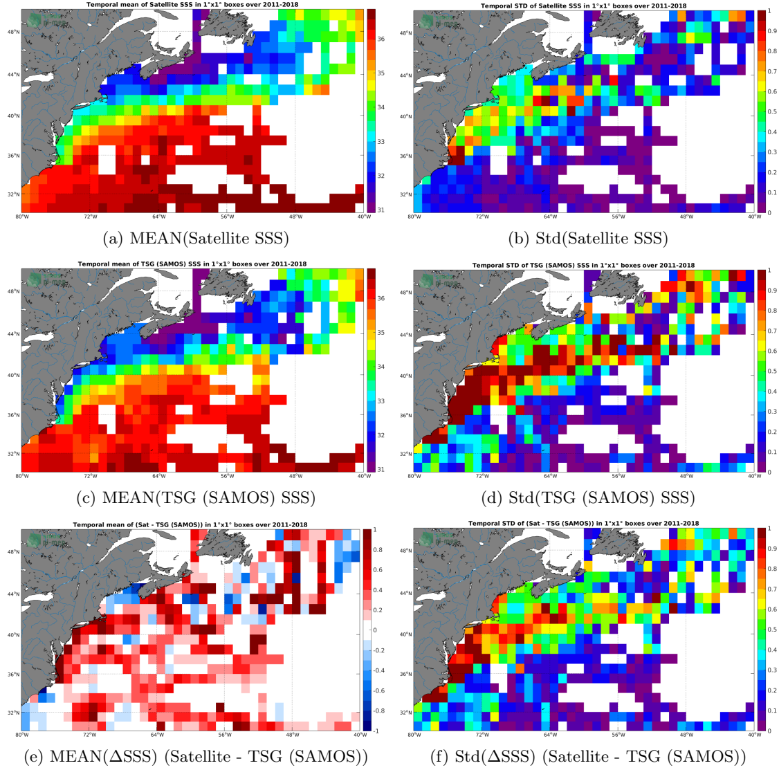
Figure 6: Temporal mean (left) and Std (right) of SSS from SMOS and SMAP SSS L4 OI v1 - 7 Days (LOPS) (top), TSG (SAMOS) (middle), and of \Delta SSS (Satellite - TSG (SAMOS)). Only match-up pairs are used to generate these maps.
