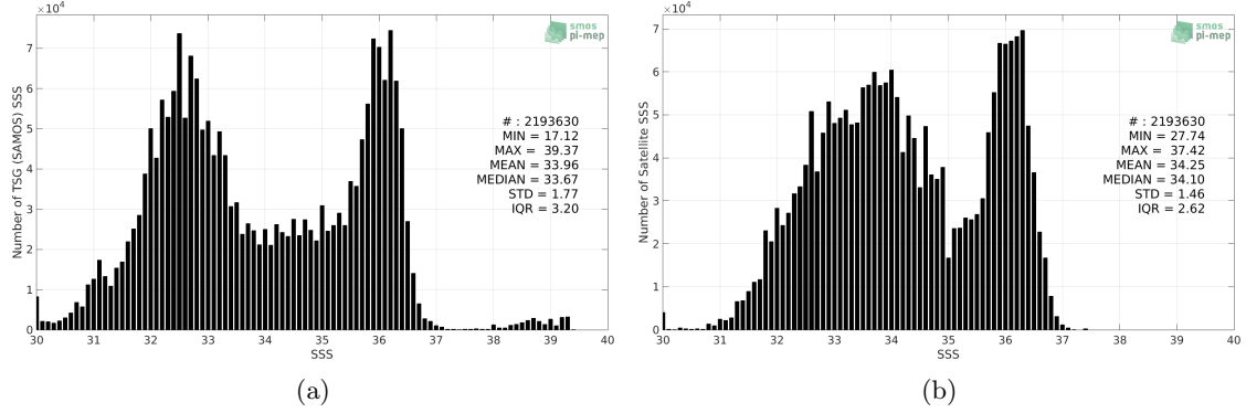
Figure 2: Histograms of SSS from TSG (SAMOS) (a) and SMOS and SMAP SSS L4 OI v1 - 7 Days (LOPS) (b) considering all match-up pairs per bins of 0.1 over the Gulf Stream Pi-MEP region and for the full satellite product period.
