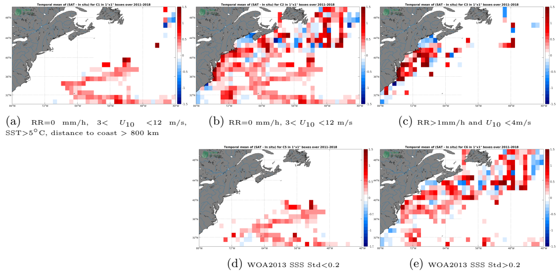
Figure 12: Temporal mean gridded over spatial boxes of size 1^\circ \times 1^\circ of \Delta SSS (SMOS and SMAP SSS L4 OI v1 - 7 Days (LOPS) - TSG (SAMOS)) for 5 different subdatasets corresponding to: RR=0 mm/h, 3 < U_{10} < 12 m/s, SST > 5^\circ C , distance to coast > 800 km (a), RR=0 mm/h, 3 < U_{10} < 12 m/s (b), RR > 1 mm/h and U_{10} < 4 m/s (c), WOA2013 SSS Std < 0.2 (d), WOA2013 SSS Std > 0.2 (e).
