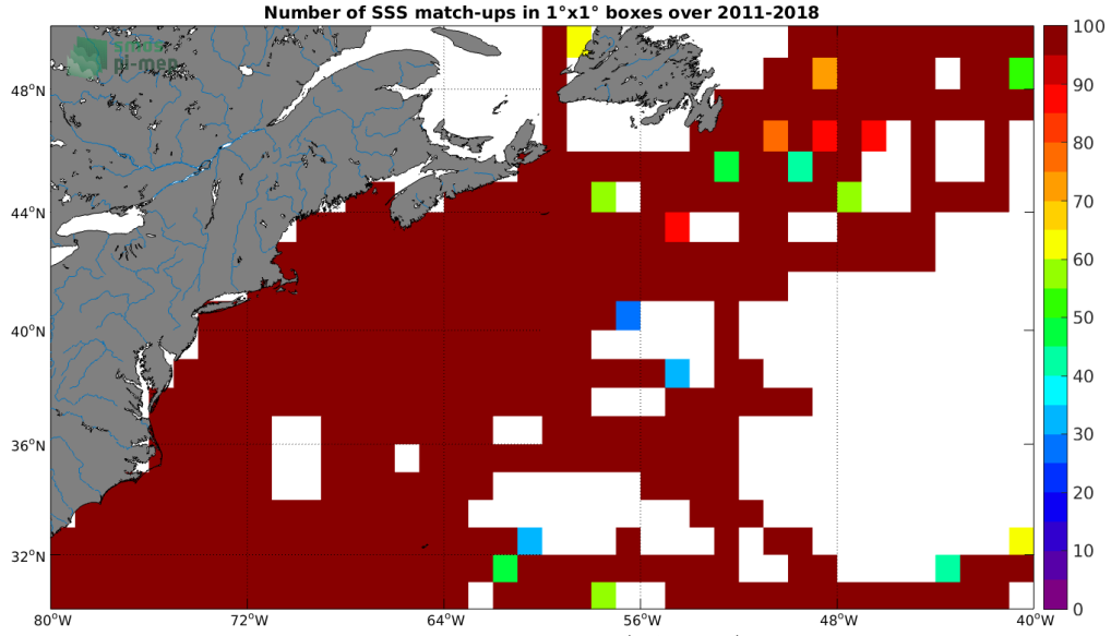
Figure 4: Number of SSS match-ups between TSG (SAMOS) SSS and the SMOS and SMAP SSS L4 OI v1 - 7 Days (LOPS) SSS product for the Gulf Stream Pi-MEP region over 1^\circ \times 1^\circ boxes and for the full satellite product period.
