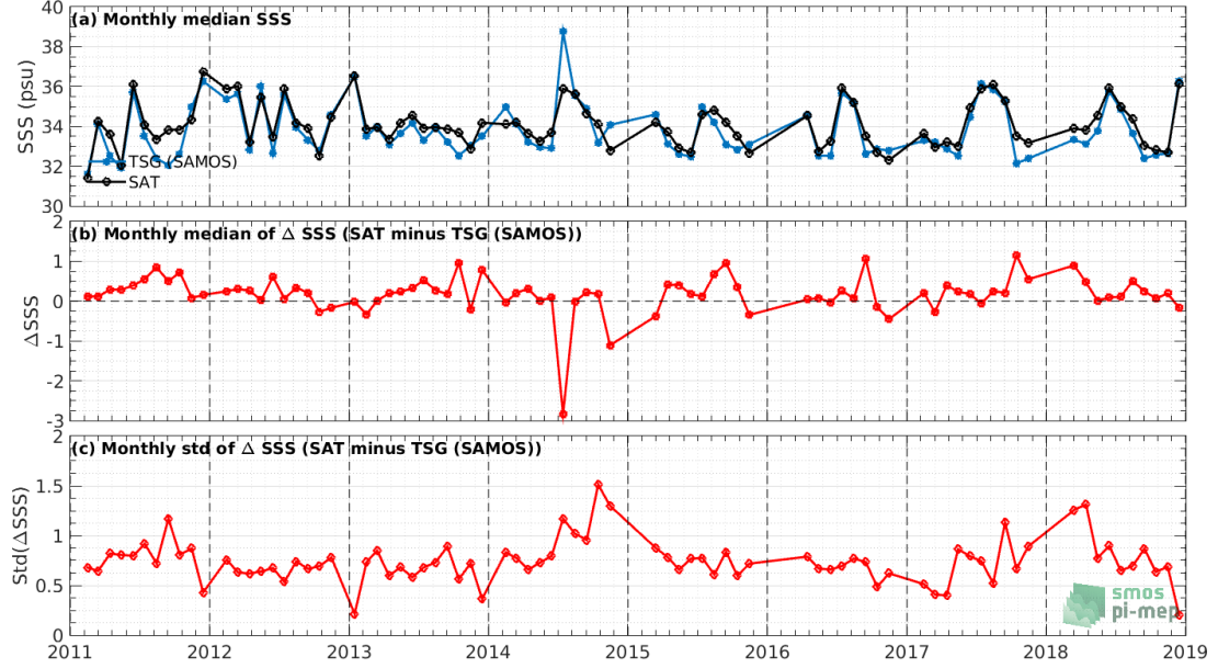
Figure 7: Time series of the monthly median SSS (top), median of \Delta\text{SSS} (Satellite - TSG (SAMOS)) and Std of \Delta\text{SSS} (Satellite - TSG (SAMOS)) over the Gulf Stream Pi-MEP region considering all match-ups collected by the Pi-MEP.
