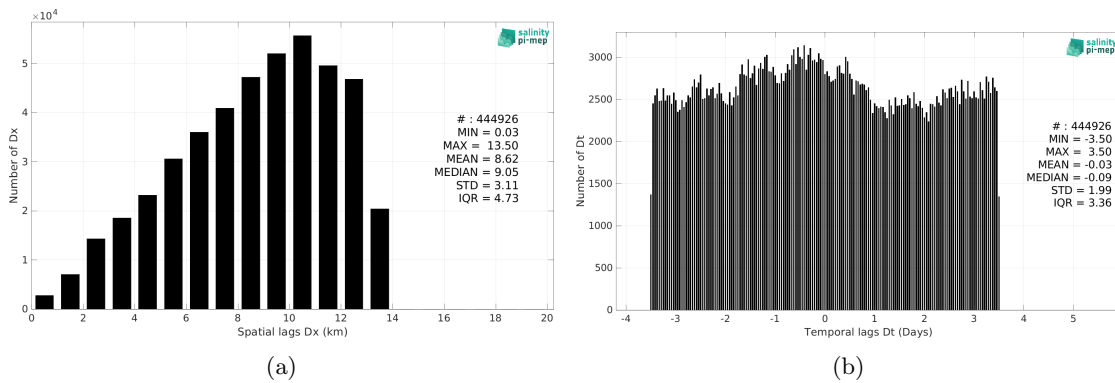
Figure 5: Histograms of the spatial (a) and temporal (b) lags between the location/time of the TSG (SAMOS) measurement and the date of the corresponding SMOS SSS L4 v1 - Weekly (CMEMS-CNR) SSS pixel.
