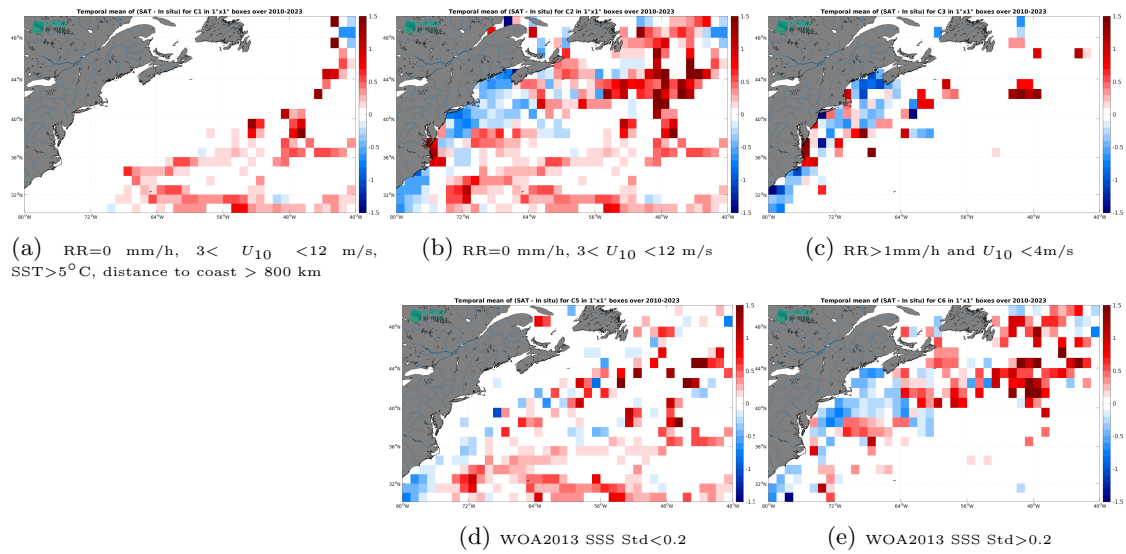
Figure 12: Temporal mean gridded over spatial boxes of size 1^\circ \times 1^\circ of \Delta SSS (SMOS SSS L4 v1 - Weekly (CMEMS-CNR) - TSG (SAMOS)) for 5 different subdatasets corresponding to:RR=0 mm/h, 3 < U_{10} < 12 m/s, SST >5^\circ C, distance to coast > 800 km (a), RR=0 mm/h, 3 < U_{10} < 12 m/s (b), RR >1 mm/h and U_{10} < 4 m/s (c), WOA2013 SSS Std <0.2 (d), WOA2013 SSS Std >0.2 (e).
