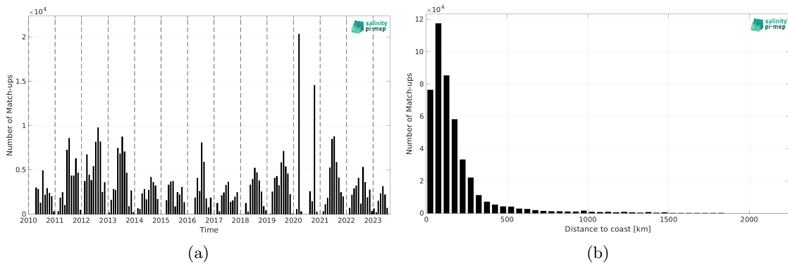
Figure 1: Number of match-ups between TSG (SAMOS) and SMOS SSS L4 v1 - Weekly (CMEMS-CNR) SSS as a function of time (a) and as function of the distance to coast (b) over the Gulf Stream Pi-MEP region and for the full satellite product period.
