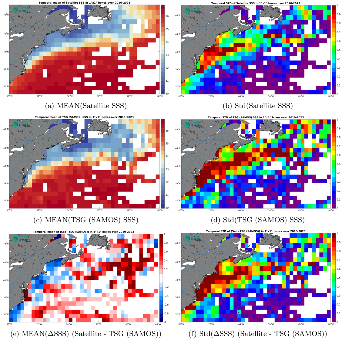
Figure 6: Temporal mean (left) and Std (right) of SSS from SMOS SSS L4 v1 - Weekly (CMEMS-CNR) (top), TSG (SAMOS) (middle), and of \Delta SSS (Satellite - TSG (SAMOS)). Only match-up pairs are used to generate these maps.
