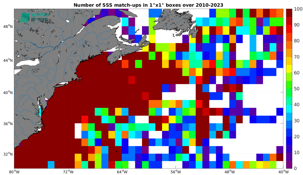
Figure 4: Number of SSS match-ups between TSG (SAMOS) SSS and the SMOS SSS L4 v1 - Weekly (CMEMS-CNR) SSS product for the Gulf Stream Pi-MEP region over 1^\circ \times 1^\circ boxes and for the full satellite product period.
