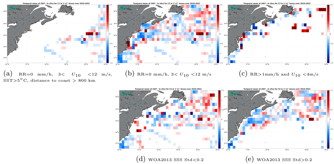
Figure 12: Temporal mean gridded over spatial boxes of size 1^\circ \times 1^\circ of \Delta SSS (SMOS SSS L4 v1 - Weekly (CMEMS-CNR) - TSG (LEGOS-DM)) for 5 different subdatasets corresponding to:RR=0 mm/h, 3 < U_{10} < 12 m/s, SST >5^\circ C, distance to coast > 800 km (a), RR=0 mm/h, 3 < U_{10} < 12 m/s (b), RR >1 mm/h and U_{10} < 4 m/s (c), WOA2013 SSS Std <0.2 (d), WOA2013 SSS Std >0.2 (e).
