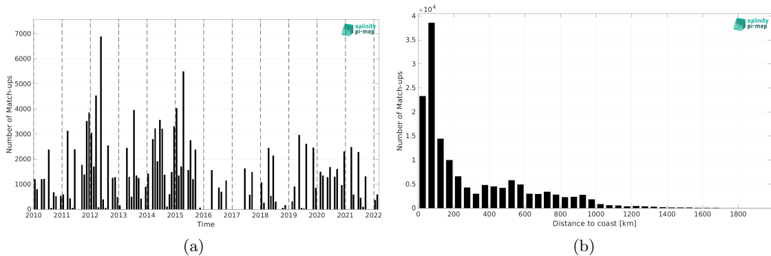
Figure 1: Number of match-ups between TSG (LEGOS-DM) and SMOS SSS L4 v1 - Weekly (CMEMS-CNR) SSS as a function of time (a) and as function of the distance to coast (b) over the Gulf Stream Pi-MEP region and for the full satellite product period.
