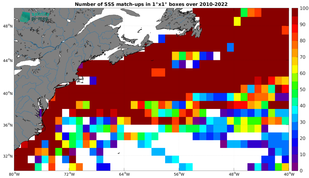
Figure 4: Number of SSS match-ups between TSG (LEGOS-DM) SSS and the SMOS SSS L4 v1 - Weekly (CMEMS-CNR) SSS product for the Gulf Stream Pi-MEP region over 1^\circ \times 1^\circ boxes and for the full satellite product period.
