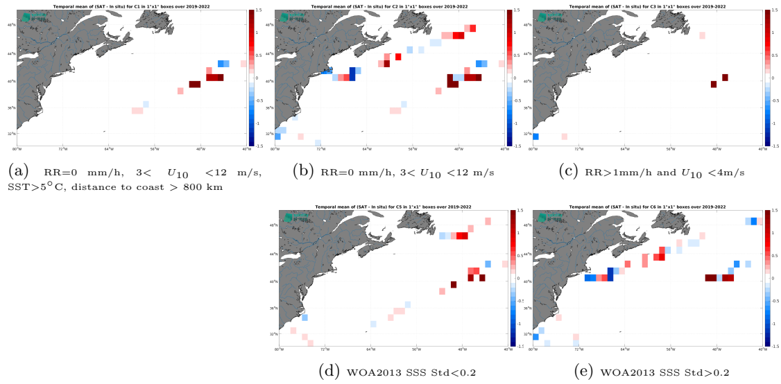
Figure 12: Temporal mean gridded over spatial boxes of size 1^\circ \times 1^\circ of \Delta SSS (SMOS SSS L4 v1 - Weekly (CMEMS-CNR) - Saildrone) for 5 different subdatasets corresponding to:RR=0 mm/h, 3 < U_{10} < 12 m/s, SST >5^\circ C, distance to coast > 800 km (a), RR=0 mm/h, 3 < U_{10} < 12 m/s (b), RR >1 mm/h and U_{10} < 4 m/s (c), WOA2013 SSS Std <0.2 (d), WOA2013 SSS Std >0.2 (e).
