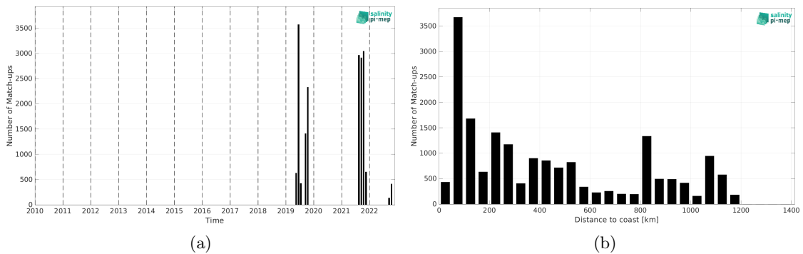
Figure 1: Number of match-ups between Saildrone and SMOS SSS L4 v1 - Weekly (CMEMS-CNR) SSS as a function of time (a) and as function of the distance to coast (b) over the Gulf Stream Pi-MEP region and for the full satellite product period.
