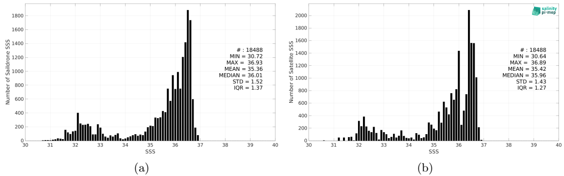
Figure 2: Histograms of SSS from Saildrone (a) and SMOS SSS L4 v1 - Weekly (CMEMS-CNR) (b) considering all match-up pairs per bins of 0.1 over the Gulf Stream Pi-MEP region and for the full satellite product period.
