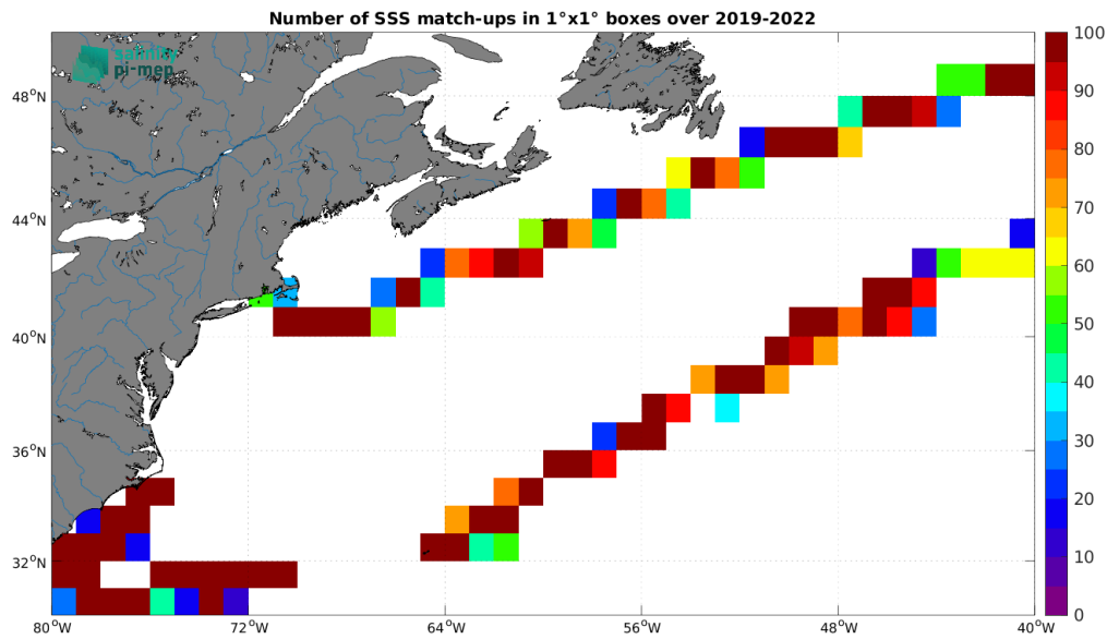
Figure 4: Number of SSS match-ups between Saildrone SSS and the SMOS SSS L4 v1 - Weekly (CMEMS-CNR) SSS product for the Gulf Stream Pi-MEP region over 1^{\circ} \times 1^{\circ} boxes and for the full satellite product period.
