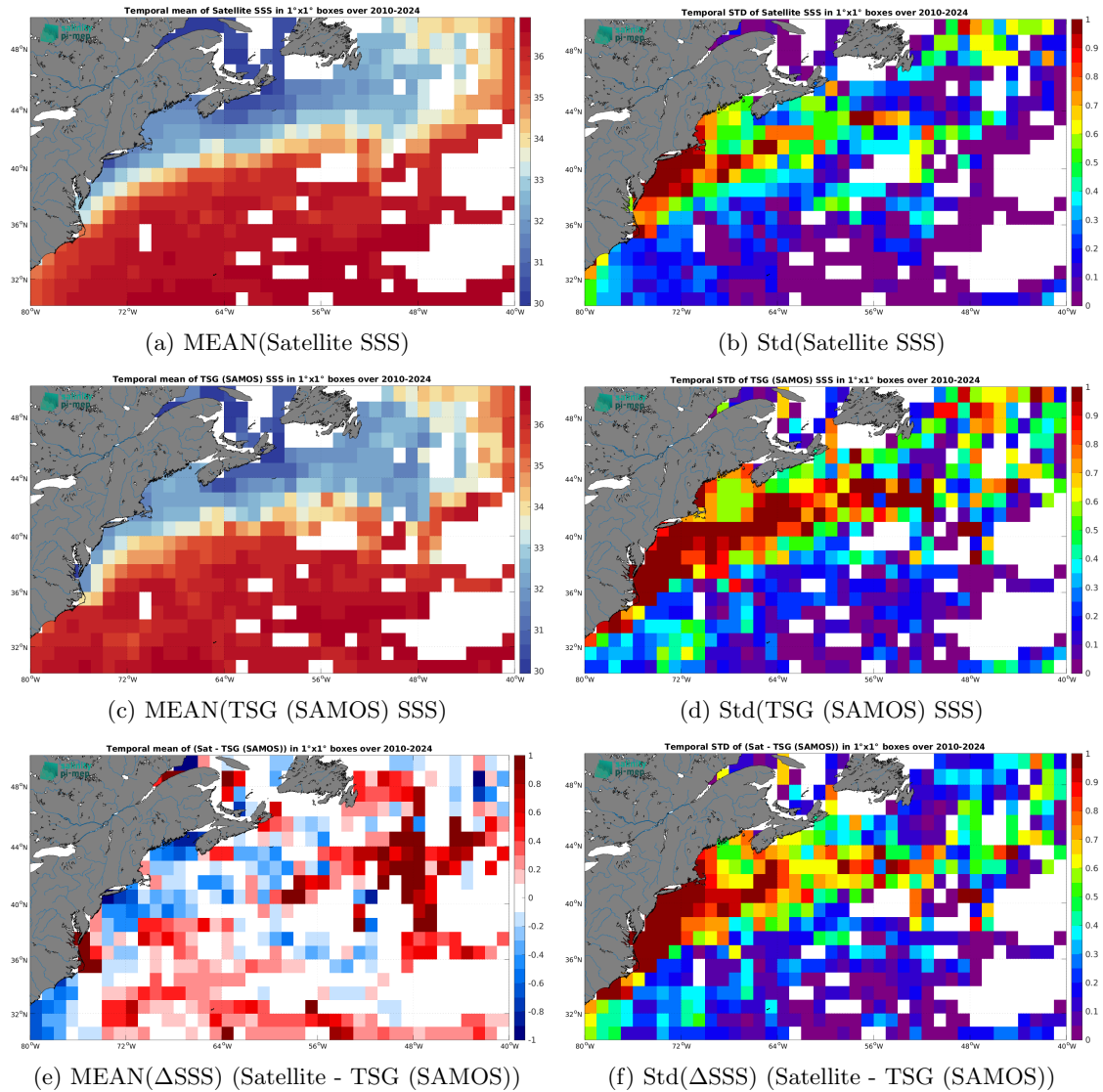
Figure 7: Temporal mean (left) and Std (right) of SSS from SMOS SSS L4 v1 - Monthly (CMEMS-CNR) (top), TSG (SAMOS) (middle), and of \Delta SSS (Satellite - TSG (SAMOS)). Only match-up pairs are used to generate these maps.
