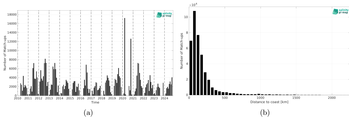
Figure 2: Number of match-ups between TSG (SAMOS) and SMOS SSS L4 v1 - Monthly (CMEMS-CNR) SSS as a function of time (a) and as function of the distance to coast (b) over the Gulf Stream Pi-MEP region and for the full satellite product period.
