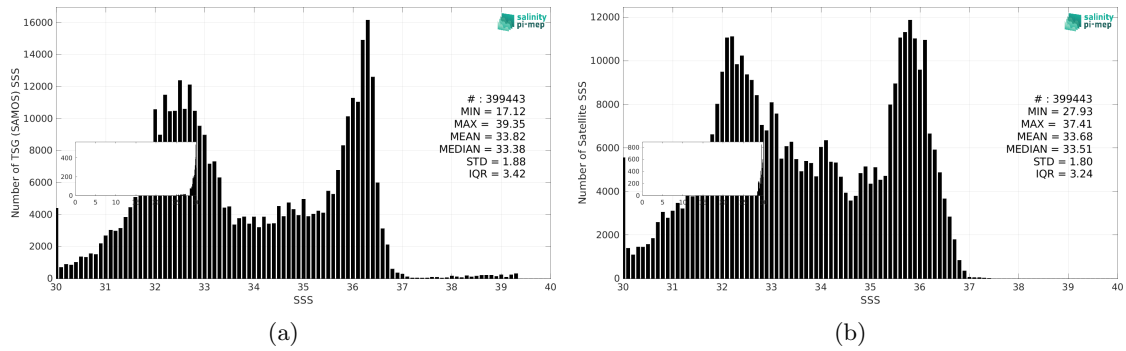
Figure 3: Histograms of SSS from TSG (SAMOS) (a) and SMOS SSS L4 v1 - Monthly (CMEMS-CNR) (b) considering all match-up pairs per bins of 0.1 over the Gulf Stream Pi-MEP region and for the full satellite product period.
