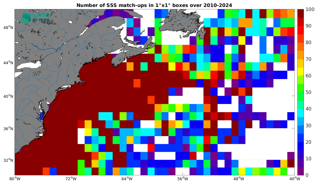
Figure 5: Number of SSS match-ups between TSG (SAMOS) SSS and the SMOS SSS L4 v1 - Monthly (CMEMS-CNR) SSS product for the Gulf Stream Pi-MEP region over 1^\circ \times 1^\circ boxes and for the full satellite product period.
