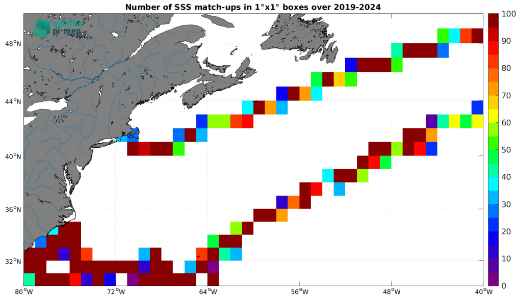
Figure 5: Number of SSS match-ups between Saildrone SSS and the SMOS SSS L4 v1 - Monthly (CMEMS-CNR) SSS product for the Gulf Stream Pi-MEP region over 1^\circ \times 1^\circ boxes and for the full satellite product period.
