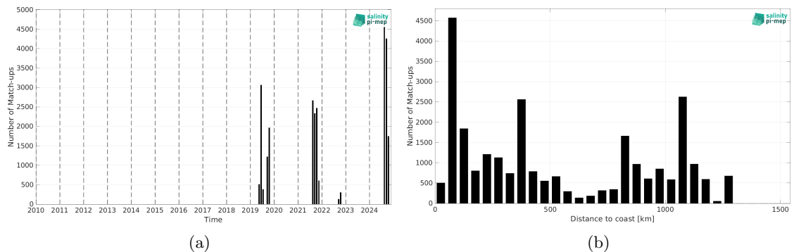
Figure 2: Number of match-ups between Saildrone and SMOS SSS L4 v1 - Monthly (CMEMS-CNR) SSS as a function of time (a) and as function of the distance to coast (b) over the Gulf Stream Pi-MEP region and for the full satellite product period.
