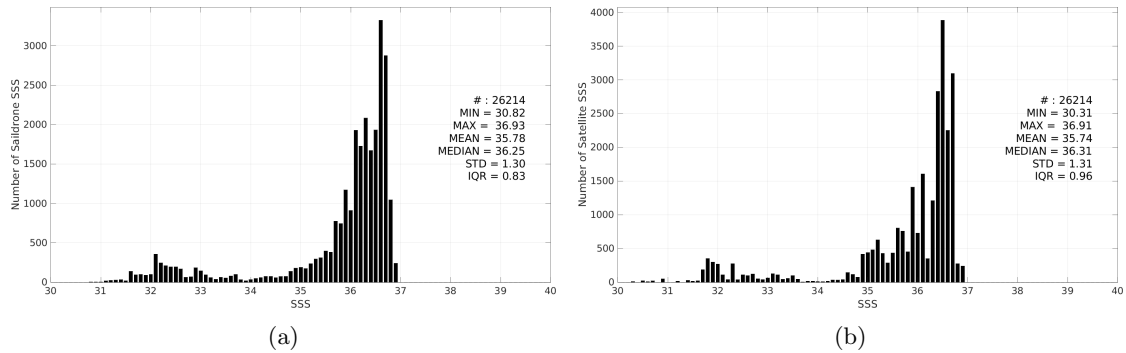
Figure 3: Histograms of SSS from Saildrone (a) and SMOS SSS L4 v1 - Monthly (CMEMS-CNR) (b) considering all match-up pairs per bins of 0.1 over the Gulf Stream Pi-MEP region and for the full satellite product period.
