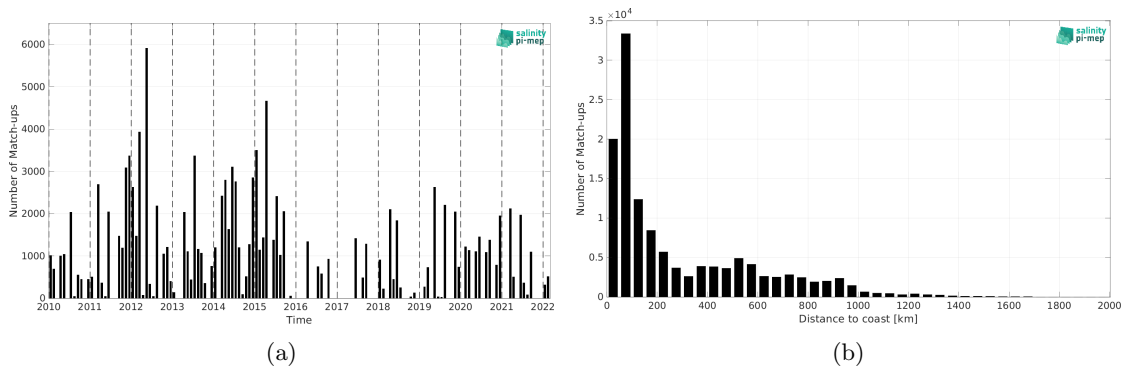
Figure 2: Number of match-ups between TSG (LEGOS-DM) and SMOS SSS L4 v1 - Daily (CMEMS-CNR) SSS as a function of time (a) and as function of the distance to coast (b) over the Gulf Stream Pi-MEP region and for the full satellite product period.
