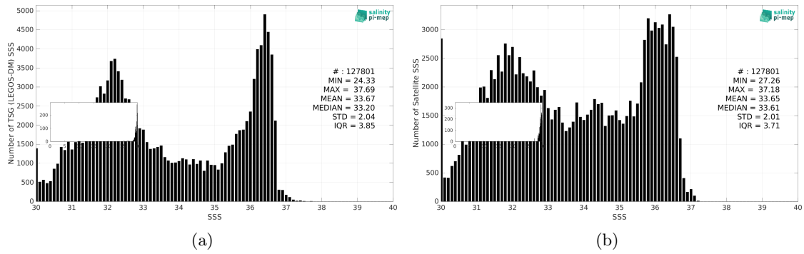
Figure 3: Histograms of SSS from TSG (LEGOS-DM) (a) and SMOS SSS L4 v1 - Daily (CMEMS-CNR) (b) considering all match-up pairs per bins of 0.1 over the Gulf Stream Pi-MEP region and for the full satellite product period.
