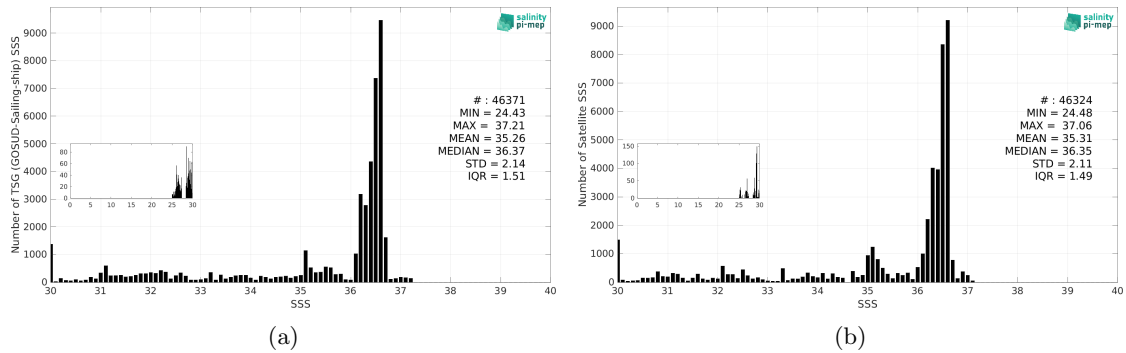
Figure 3: Histograms of SSS from TSG (GOSUD-Sailing-ship) (a) and SMOS SSS L4 v1 - Daily (CMEMS-CNR) (b) considering all match-up pairs per bins of 0.1 over the Gulf Stream Pi-MEP region and for the full satellite product period.
