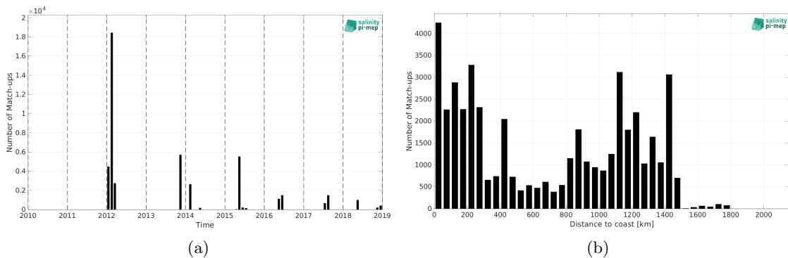
Figure 2: Number of match-ups between TSG (GOSUD-Sailing-ship) and SMOS SSS L4 v1 - Daily (CMEMS-CNR) SSS as a function of time (a) and as function of the distance to coast (b) over the Gulf Stream Pi-MEP region and for the full satellite product period.
