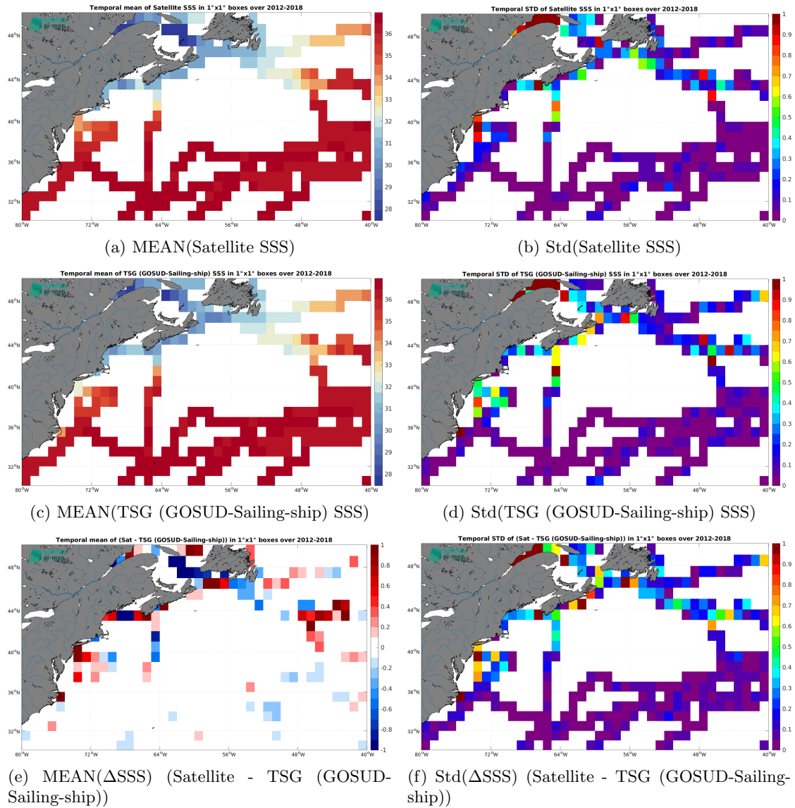
Figure 7: Temporal mean (left) and Std (right) of SSS from SMOS SSS L4 v1 - Daily (CMEMS-CNR) (top), TSG (GOSUD-Sailing-ship) (middle), and of \Delta SSS (Satellite - TSG (GOSUD-Sailing-ship)). Only match-up pairs are used to generate these maps.
