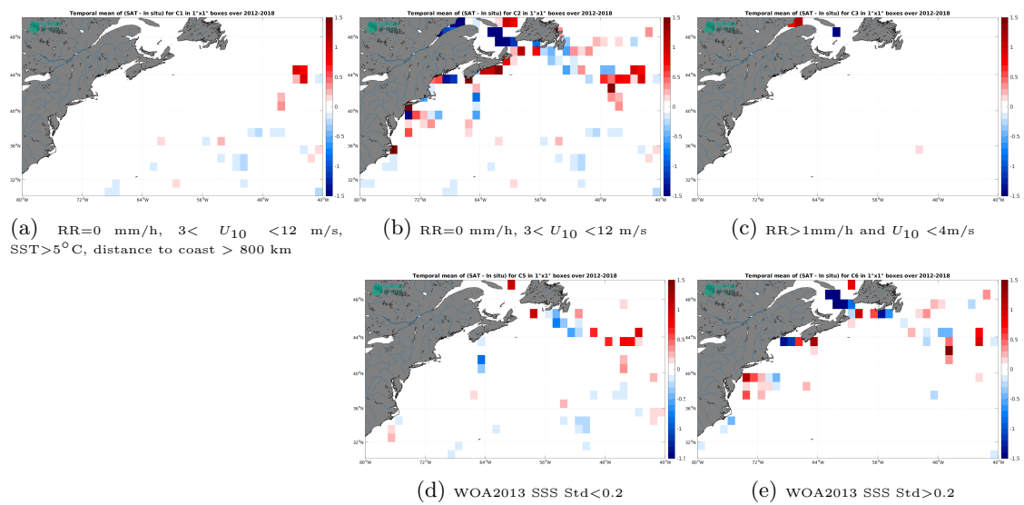
Figure 14: Temporal mean gridded over spatial boxes of size 1^\circ \times 1^\circ of \Delta SSS (SMOS SSS L4 v1 - Daily (CMEMS-CNR) - TSG (GOSUD-Sailing-ship)) for 5 different subdatasets corresponding to:RR=0 mm/h, 3 < U_{10} < 12 m/s, SST >5^\circ\text{C} , distance to coast > 800 km (a), RR=0 mm/h, 3 < U_{10} < 12 m/s (b), RR >1 mm/h and U_{10} < 4 m/s (c), WOA2013 SSS Std <0.2 (d), WOA2013 SSS Std >0.2 (e).
