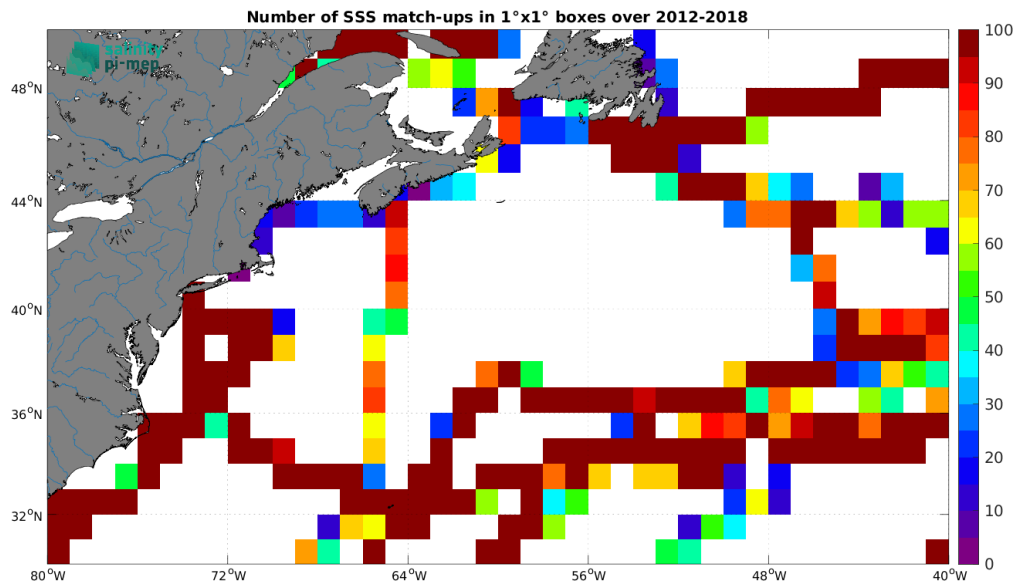
Figure 5: Number of SSS match-ups between TSG (GOSUD-Sailing-ship) SSS and the SMOS SSS L4 v1 - Daily (CMEMS-CNR) SSS product for the Gulf Stream Pi-MEP region over 1^\circ \times 1^\circ boxes and for the full satellite product period.
