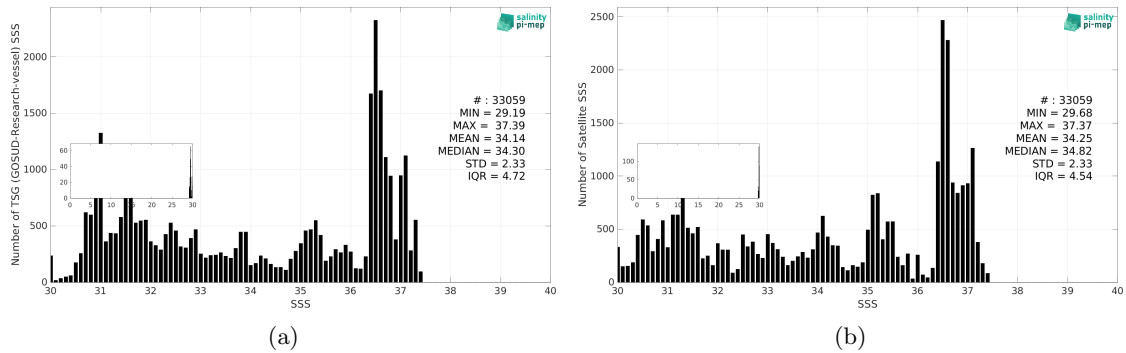
Figure 3: Histograms of SSS from TSG (GOSUD-Research-vessel) (a) and SMOS SSS L4 v1 - Daily (CMEMS-CNR) (b) considering all match-up pairs per bins of 0.1 over the Gulf Stream Pi-MEP region and for the full satellite product period.
