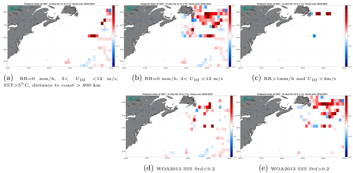
Figure 14: Temporal mean gridded over spatial boxes of size 1^\circ \times 1^\circ of \Delta SSS (SMOS SSS L4 v1 - Daily (CMEMS-CNR) - TSG (GOSUD-Research-vessel)) for 5 different subdatasets corresponding to:RR=0 mm/h, 3 < U_{10} < 12 m/s, SST>5°C, distance to coast > 800 km (a), RR=0 mm/h, 3 < U_{10} < 12 m/s (b), RR>1mm/h and U_{10} < 4 m/s (c), WOA2013 SSS Std<0.2 (d), WOA2013 SSS Std>0.2 (e).
