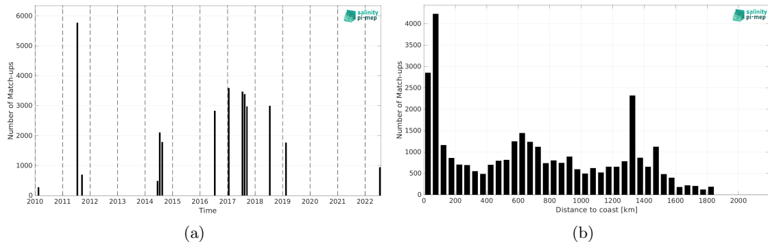
Figure 2: Number of match-ups between TSG (GOSUD-Research-vessel) and SMOS SSS L4 v1 - Daily (CMEMS-CNR) SSS as a function of time (a) and as function of the distance to coast (b) over the Gulf Stream Pi-MEP region and for the full satellite product period.
