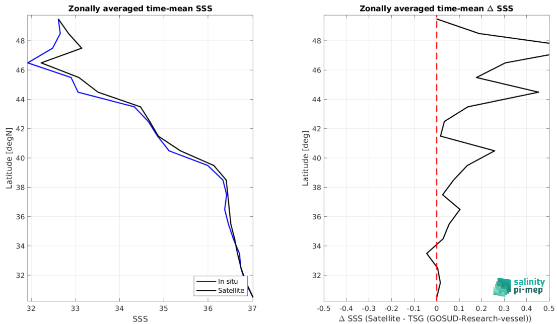
Figure 9: Left panel: Zonal mean SSS from SMOS SSS L4 v1 - Daily (CMEMS-CNR) satellite product (black) and from TSG (GOSUD-Research-vessel) (blue). Right panel: Zonal mean of \Delta SSS (Satellite - TSG (GOSUD-Research-vessel)) for all the collected Pi-MEP match-up pairs estimated over the full satellite product period.
