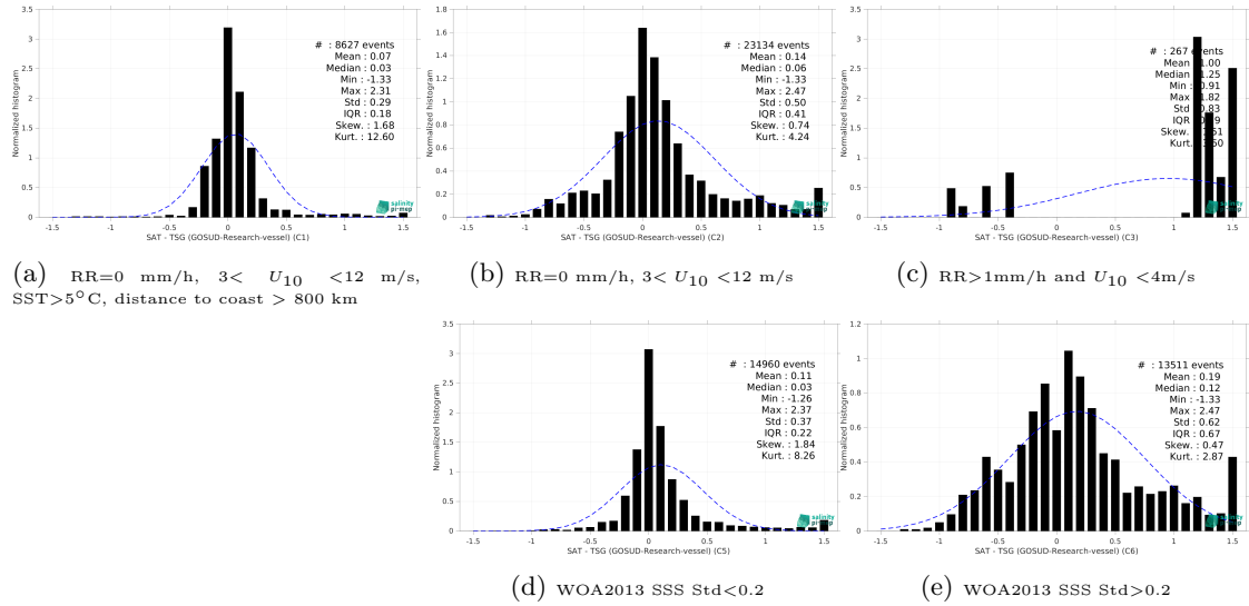
Figure 15: Normalized histogram of \Delta SSS (SMOS SSS L4 v1 - Daily (CMEMS-CNR) - TSG (GOSUD-Research-vessel)) for 5 different subdatasets corresponding to: RR=0 mm/h, 3 < U_{10} < 12 m/s, SST > 5°C, distance to coast > 800 km (a), RR=0 mm/h, 3 < U_{10} < 12 m/s (b), RR > 1mm/h and U_{10} < 4 m/s (c), WOA2013 SSS Std < 0.2 (d), WOA2013 SSS Std > 0.2 (e).
