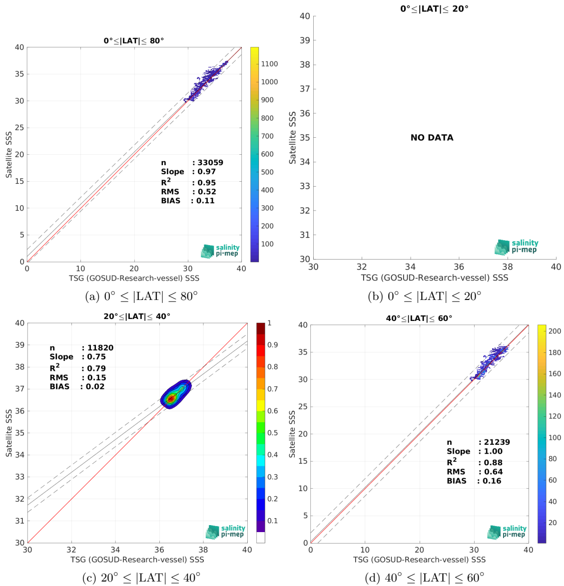
Figure 10: Contour maps of the concentration of SMOS SSS L4 v1 - Daily (CMEMS-CNR) SSS (y-axis) versus TSG (GOSUD-Research-vessel) SSS (x-axis) at match-up pairs for different latitude bands. For each plot, the red line shows x=y . The black thin and dashed lines indicate a linear fit through the data cloud and the \pm 95\% confidence levels, respectively. The number match-up pairs n , the slope and R^2 coefficient of the linear fit, the root mean square (RMS) and the mean bias between satellite and in situ data are indicated for each latitude band in each plots.
