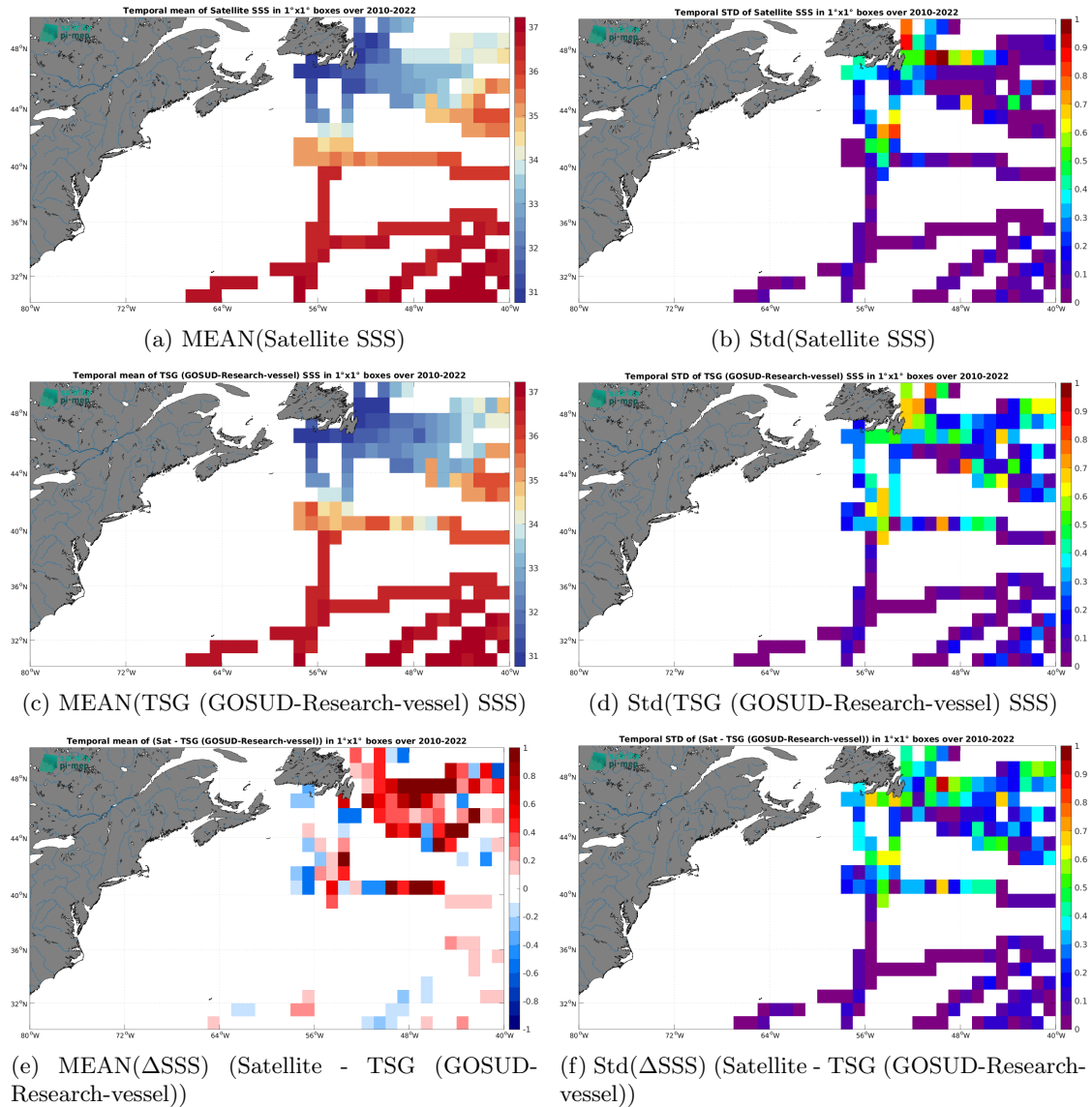
Figure 7: Temporal mean (left) and Std (right) of SSS from SMOS SSS L4 v1 - Daily (CMEMS-CNR) (top), TSG (GOSUD-Research-vessel) (middle), and of \Delta SSS (Satellite - TSG (GOSUD-Research-vessel)). Only match-up pairs are used to generate these maps.
