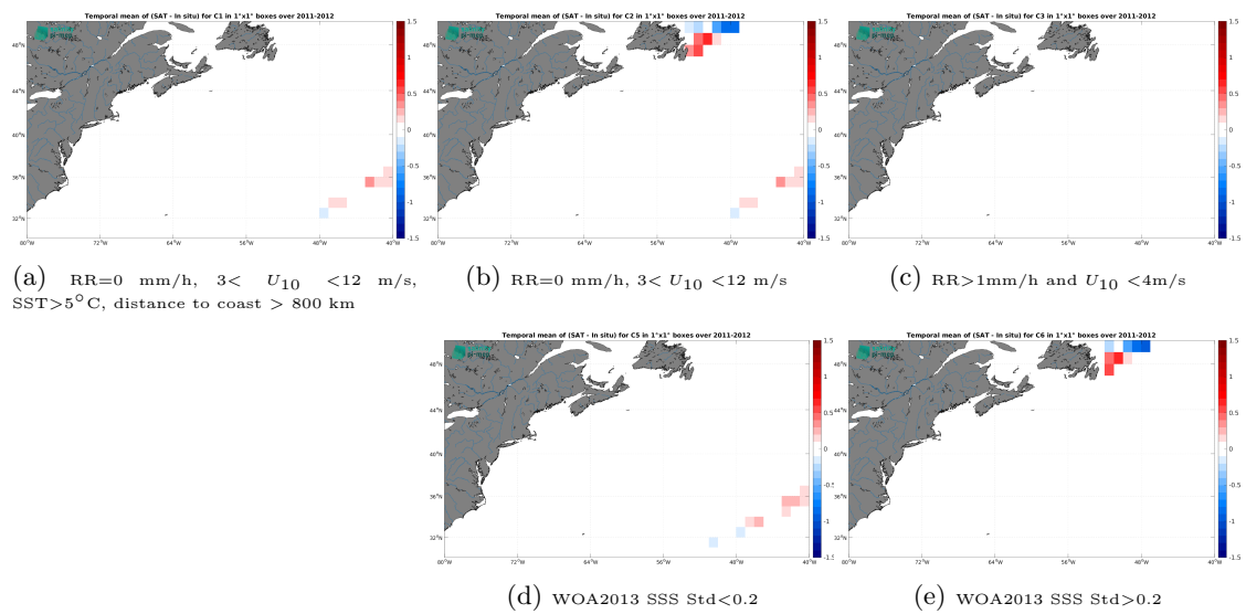
Figure 14: Temporal mean gridded over spatial boxes of size 1^\circ \times 1^\circ of \Delta SSS (SMOS SSS L4 v1 - Daily (CMEMS-CNR) - TSG (CSIC-UTM)) for 5 different subdatasets corresponding to:RR=0 mm/h, 3 < U_{10} < 12 m/s, SST > 5°C, distance to coast > 800 km (a), RR=0 mm/h, 3 < U_{10} < 12 m/s (b), RR > 1mm/h and U_{10} < 4 m/s (c), WOA2013 SSS Std < 0.2 (d), WOA2013 SSS Std > 0.2 (e).
