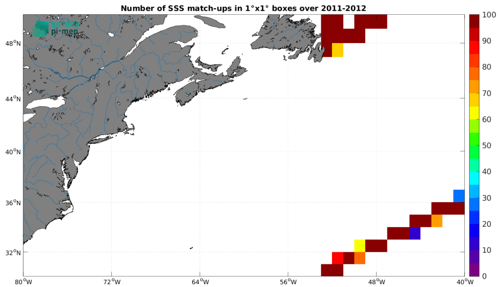
Figure 5: Number of SSS match-ups between TSG (CSIC-UTM) SSS and the SMOS SSS L4 v1 - Daily (CMEMS-CNR) SSS product for the Gulf Stream Pi-MEP region over 1^\circ \times 1^\circ boxes and for the full satellite product period.
