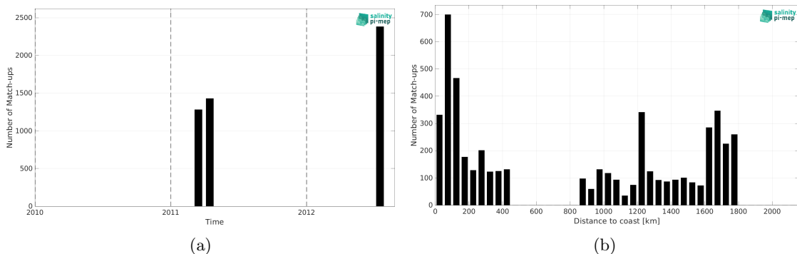
Figure 2: Number of match-ups between TSG (CSIC-UTM) and SMOS SSS L4 v1 - Daily (CMEMS-CNR) SSS as a function of time (a) and as function of the distance to coast (b) over the Gulf Stream Pi-MEP region and for the full satellite product period.
