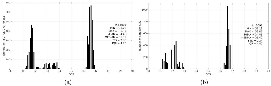
Figure 3: Histograms of SSS from TSG (CSIC-UTM) (a) and SMOS SSS L4 v1 - Daily (CMEMS-CNR) (b) considering all match-up pairs per bins of 0.1 over the Gulf Stream Pi-MEP region and for the full satellite product period.
