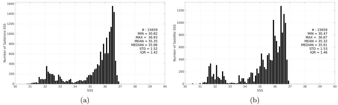
Figure 3: Histograms of SSS from Saildrone (a) and SMOS SSS L4 v1 - Daily (CMEMS-CNR) (b) considering all match-up pairs per bins of 0.1 over the Gulf Stream Pi-MEP region and for the full satellite product period.
