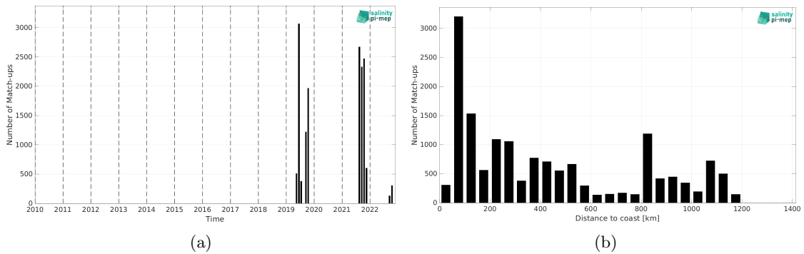
Figure 2: Number of match-ups between Saildrone and SMOS SSS L4 v1 - Daily (CMEMS-CNR) SSS as a function of time (a) and as function of the distance to coast (b) over the Gulf Stream Pi-MEP region and for the full satellite product period.
