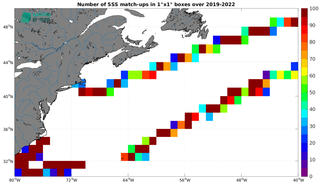
Figure 5: Number of SSS match-ups between Saildrone SSS and the SMOS SSS L4 v1 - Daily (CMEMS-CNR) SSS product for the Gulf Stream Pi-MEP region over 1^{\circ} \times 1^{\circ} boxes and for the full satellite product period.
