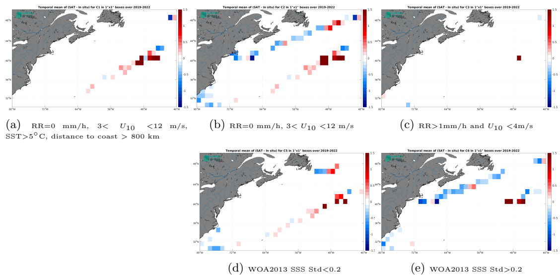
Figure 14: Temporal mean gridded over spatial boxes of size 1^\circ \times 1^\circ of \Delta SSS (SMOS SSS L4 v1 - Daily (CMEMS-CNR) - Sailability) for 5 different subdatasets corresponding to: RR=0 mm/h, 3 < U_{10} < 12 m/s, SST > 5^\circ C , distance to coast > 800 km (a), RR=0 mm/h, 3 < U_{10} < 12 m/s (b), RR > 1 mm/h and U_{10} < 4 m/s (c), WOA2013 SSS Std < 0.2 (d), WOA2013 SSS Std > 0.2 (e).
