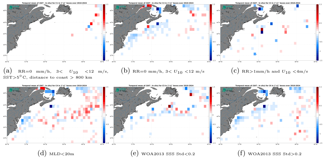
Figure 14: Temporal mean gridded over spatial boxes of size 1^\circ \times 1^\circ of \Delta SSS (SMOS SSS L4 v1 - Daily (CMEMS-CNR) - Argo) for 6 different subdatasets corresponding to:RR=0 mm/h, 3 < U_{10} < 12 m/s, SST >5^\circ C, distance to coast > 800 km (a), RR=0 mm/h, 3 < U_{10} < 12 m/s (b), RR >1 mm/h and U_{10} < 4 m/s (c),MLD <20 m (d),WOA2013 SSS Std <0.2 (e),WOA2013 SSS Std >0.2 (f).
