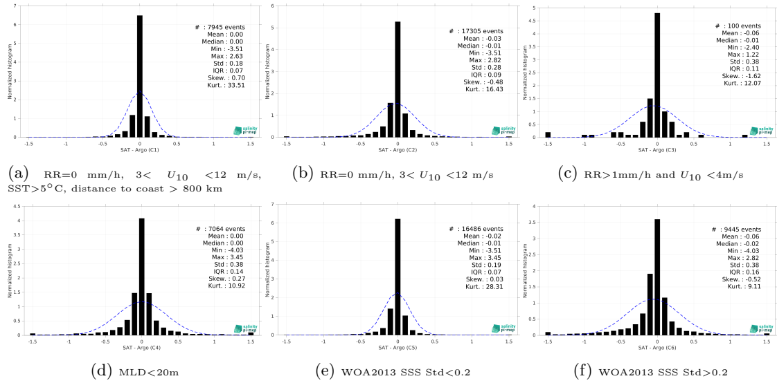
Figure 15: Normalized histogram of \Delta SSS (SMOS SSS L4 v1 - Daily (CMEMS-CNR) - Argo) for 6 different subdatasets corresponding to: RR=0 mm/h, 3 < U_{10} < 12 m/s, SST > 5°C, distance to coast > 800 km (a), RR=0 mm/h, 3 < U_{10} < 12 m/s (b), RR > 1mm/h and U_{10} < 4 m/s (c), MLD < 20m (d), WOA2013 SSS Std < 0.2 (e), WOA2013 SSS Std > 0.2 (f).
