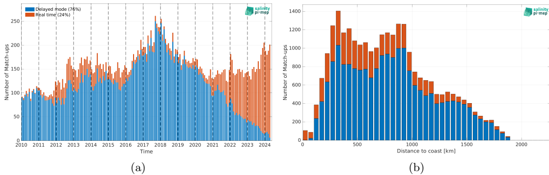
Figure 2: Number of match-ups between Argo and SMOS SSS L4 v1 - Daily (CMEMS-CNR) SSS as a function of time (a) and as function of the distance to coast (b) over the Gulf Stream Pi-MEP region and for the full satellite product period.
