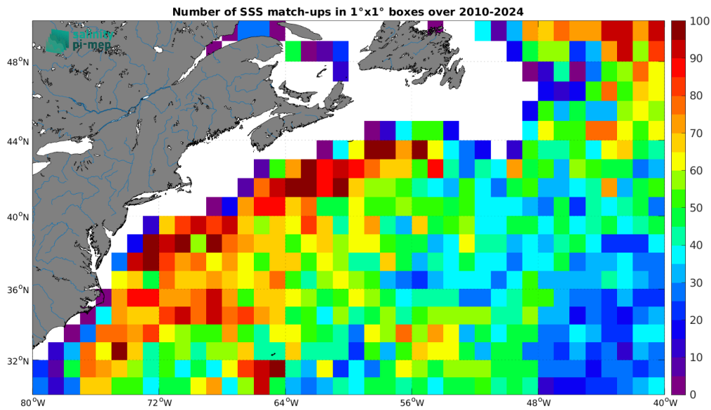
Figure 5: Number of SSS match-ups between Argo SSS and the SMOS SSS L4 v1 - Daily (CMEMS-CNR) SSS product for the Gulf Stream Pi-MEP region over 1^\circ \times 1^\circ boxes and for the full satellite product period.
