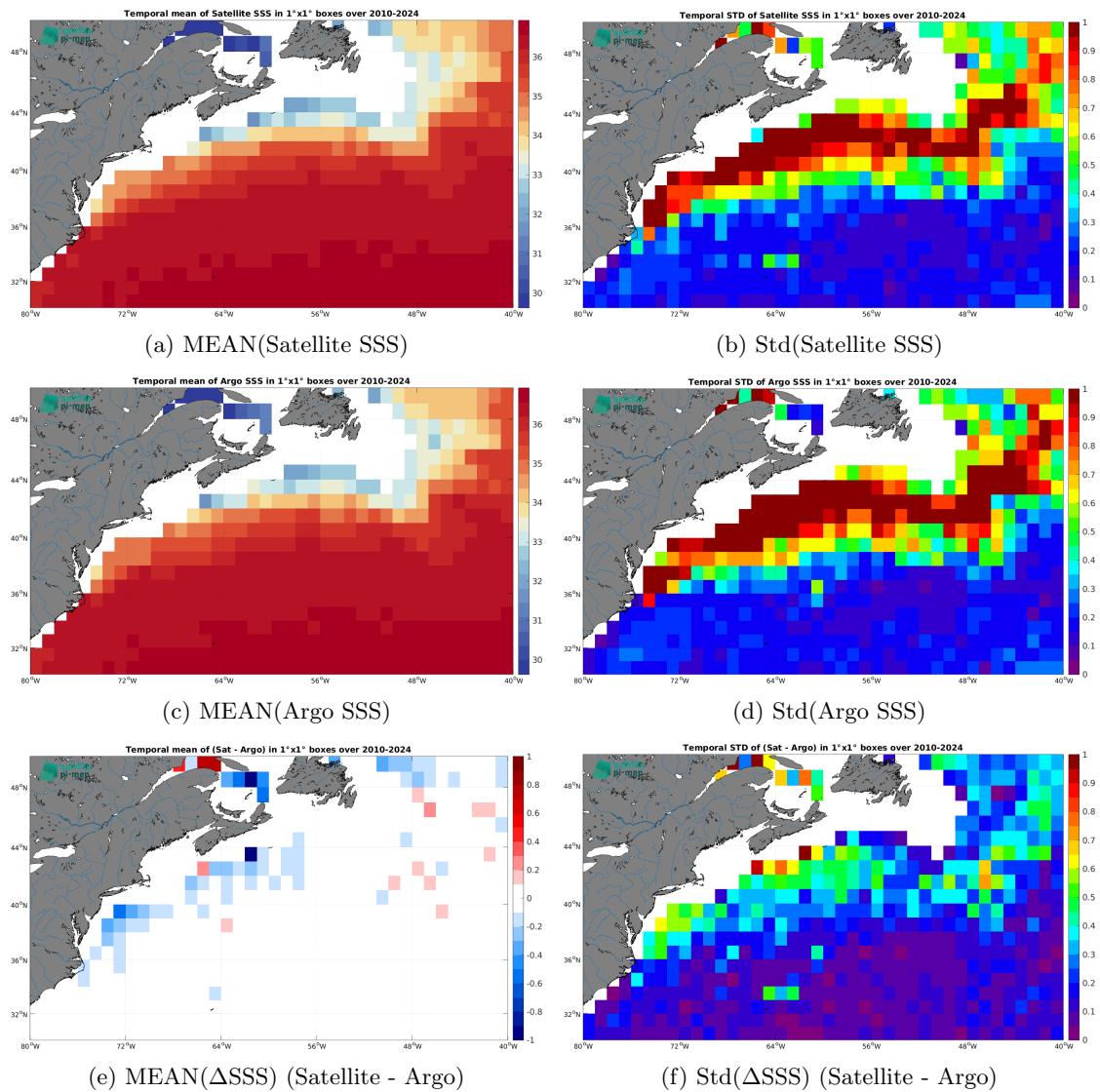
Figure 7: Temporal mean (left) and Std (right) of SSS from SMOS SSS L4 v1 - Daily (CMEMS-CNR) (top), Argo (middle), and of \Delta SSS (Satellite - Argo). Only match-up pairs are used to generate these maps.
