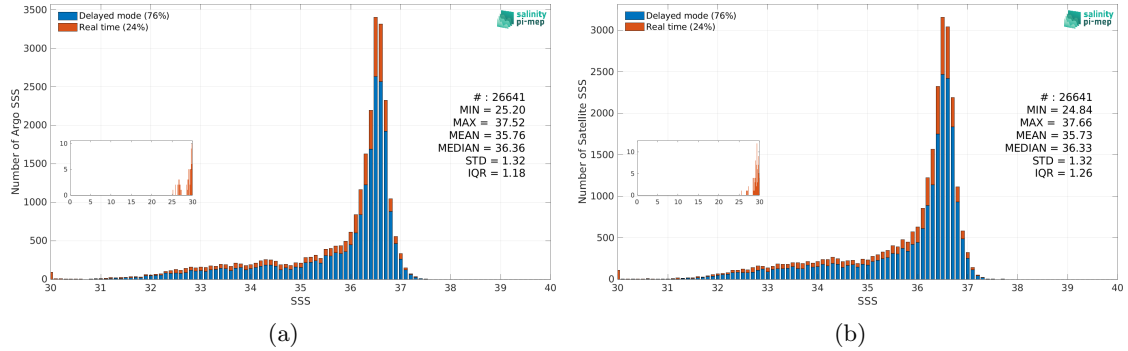
Figure 3: Histograms of SSS from Argo (a) and SMOS SSS L4 v1 - Daily (CMEMS-CNR) (b) considering all match-up pairs per bins of 0.1 over the Gulf Stream Pi-MEP region and for the full satellite product period.
