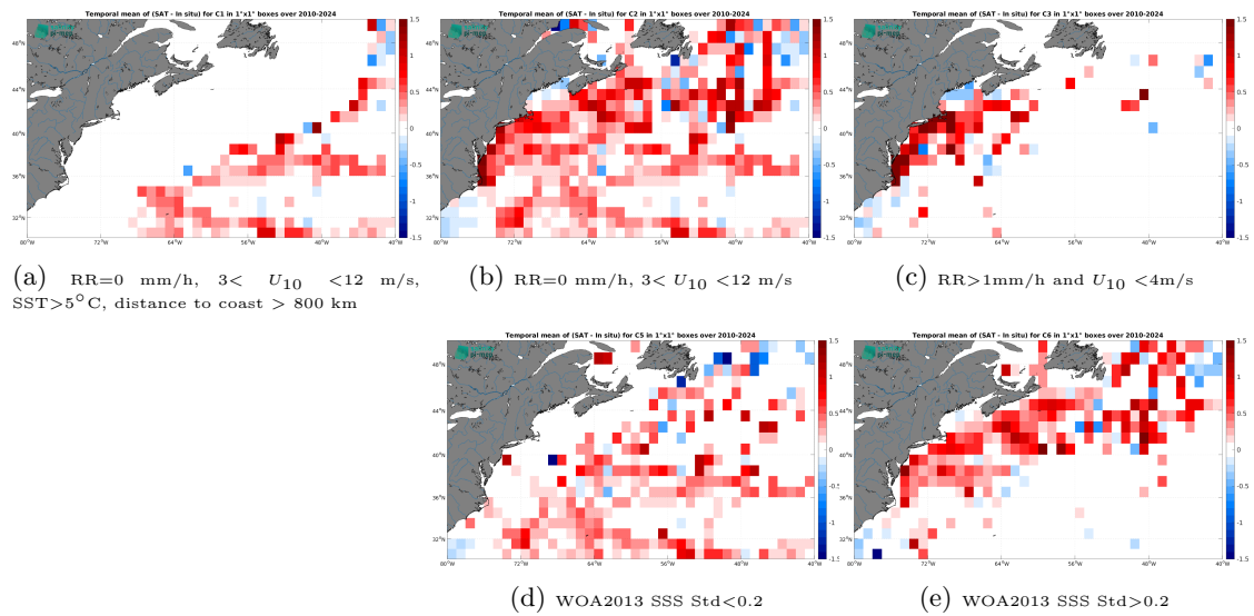
Figure 14: Temporal mean gridded over spatial boxes of size 1^\circ \times 1^\circ of \Delta SSS (SMOS SSS L4 OI v346 - Weekly (CMEMS-CATDS-LOPS) - TSG (SAMOS)) for 5 different subdatasets corresponding to:RR=0 mm/h, 3 < U_{10} < 12 m/s, SST>5°C, distance to coast > 800 km (a), RR=0 mm/h, 3 < U_{10} < 12 m/s (b), RR>1mm/h and U_{10} < 4 m/s (c), WOA2013 SSS Std<0.2 (d), WOA2013 SSS Std>0.2 (e).
