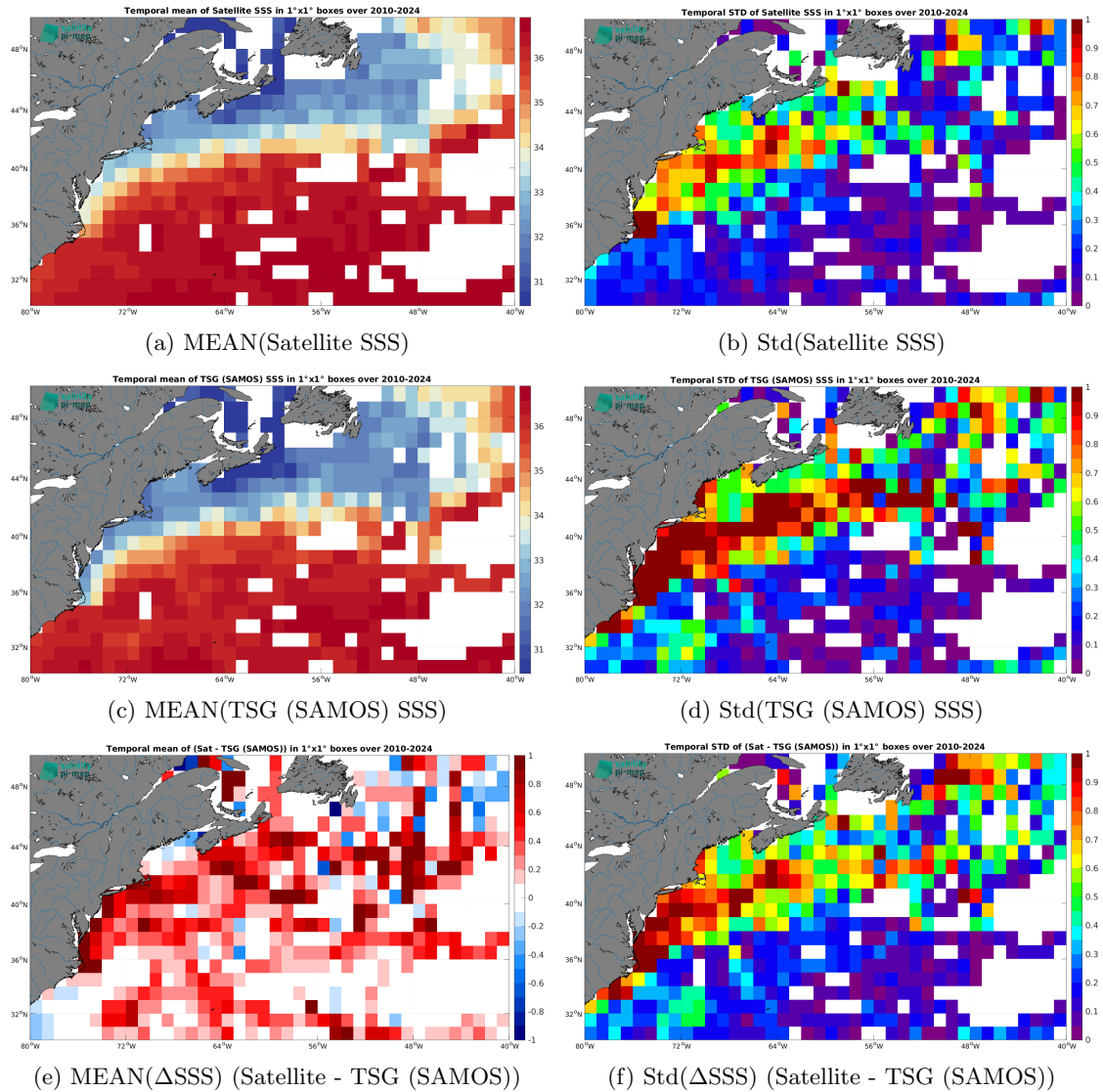
Figure 7: Temporal mean (left) and Std (right) of SSS from SMOS SSS L4 OI v346 - Weekly (CMEMS-CATDS-LOPS) (top), TSG (SAMOS) ( in situ ) dataset (middle), and of \Delta SSS (Satellite - TSG (SAMOS)). Only match-up pairs are used to generate these maps.
