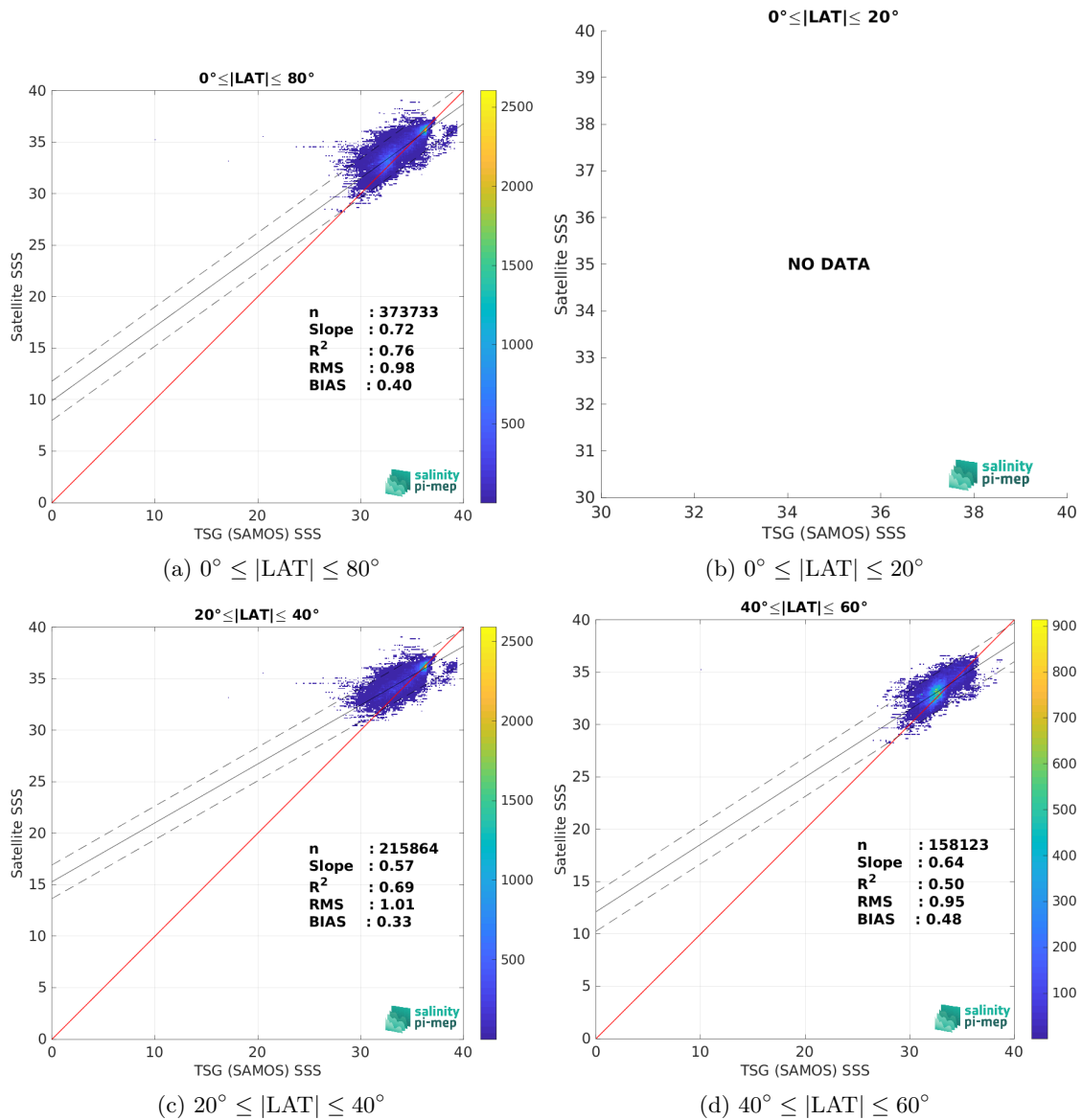
Figure 10: Contour maps of the concentration of SMOS SSS L4 OI v346 - Weekly (CMEMS-CATDS-LOPS) SSS ( y -axis) versus TSG (SAMOS) SSS ( x -axis) at match-up pairs for different latitude bands. For each plot, the red line shows x=y . The black thin and dashed lines indicate a linear fit through the data cloud and the \pm 95\% confidence levels, respectively. The number match-up pairs n , the slope and R^2 coefficient of the linear fit, the root mean square (RMS) and the mean bias between satellite and in situ data are indicated for each latitude band in each plots.
