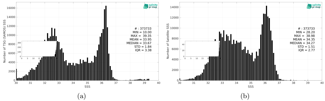
Figure 3: Histograms of SSS from TSG (SAMOS) (a) and SMOS SSS L4 OI v346 - Weekly (CMEMS-CATDS-LOPS) (b) considering all match-up pairs per bins of 0.1 over the Gulf Stream Pi-MEP region and for the full satellite product period.
