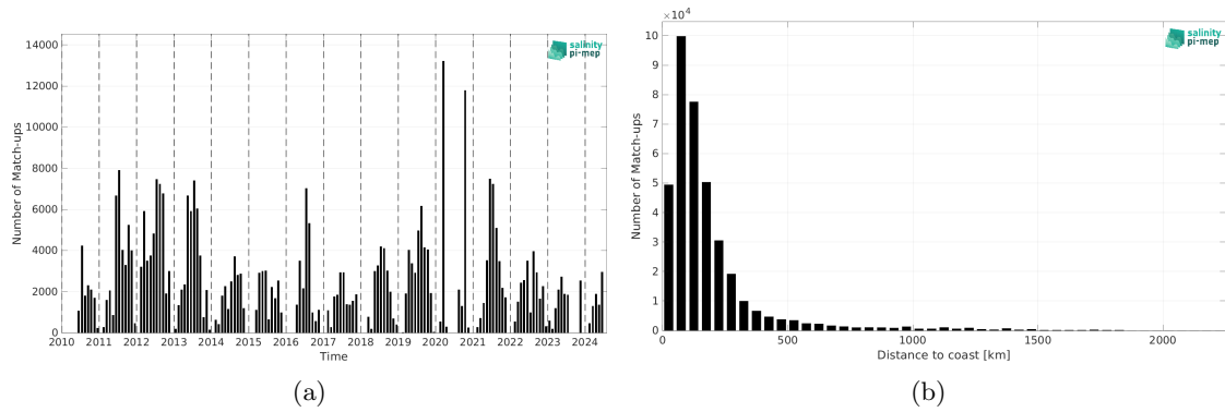
Figure 2: Number of match-ups between TSG (SAMOS) and SMOS SSS L4 OI v346 - Weekly (CMEMS-CATDS-LOPS) SSS as a function of time (a) and as function of the distance to coast (b) over the Gulf Stream Pi-MEP region and for the full satellite product period.
