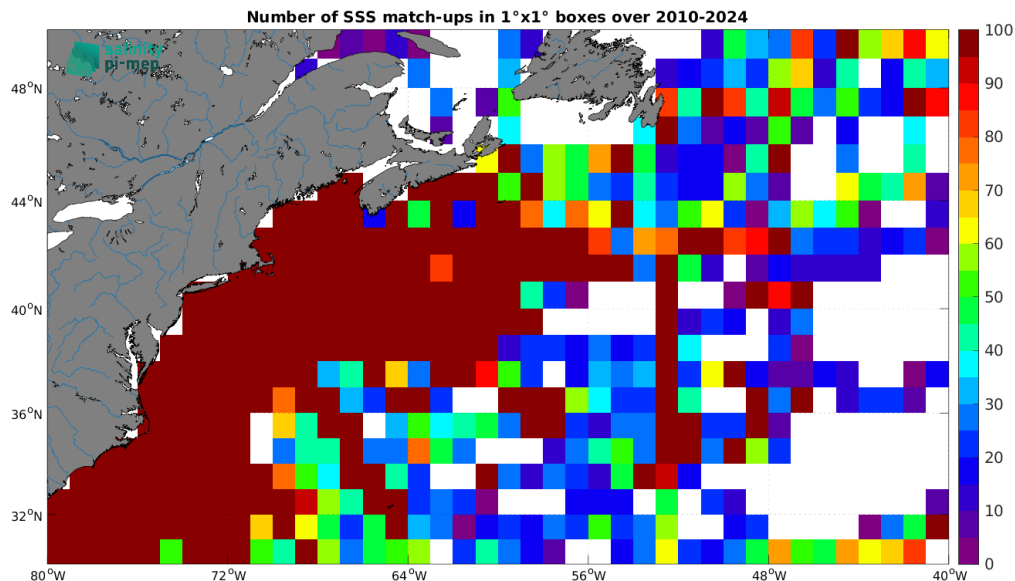
Figure 5: Number of SSS match-ups between TSG (SAMOS) SSS and the SMOS SSS L4 OI v346 - Weekly (CMEMS-CATDS-LOPS) SSS product for the Gulf Stream Pi-MEP region over 1^\circ \times 1^\circ boxes and for the full satellite product period.
