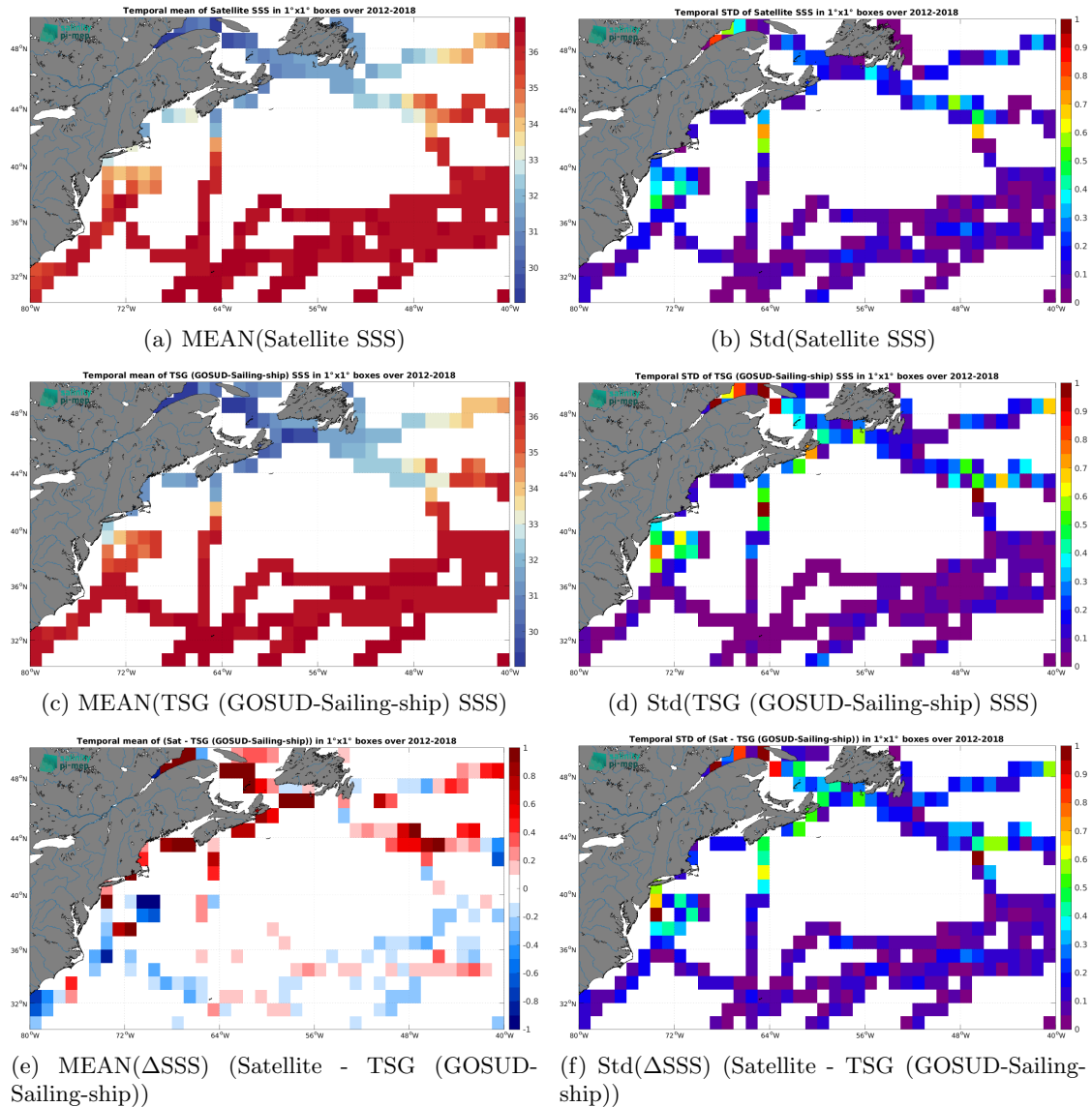
Figure 7: Temporal mean (left) and Std (right) of SSS from SMOS SSS L4 OI v346 - Weekly (CMEMS-CATDS-LOPS) (top), TSG (GOSUD-Sailing-ship) (middle), and of \Delta SSS (Satellite - TSG (GOSUD-Sailing-ship)). Only match-up pairs are used to generate these maps.
