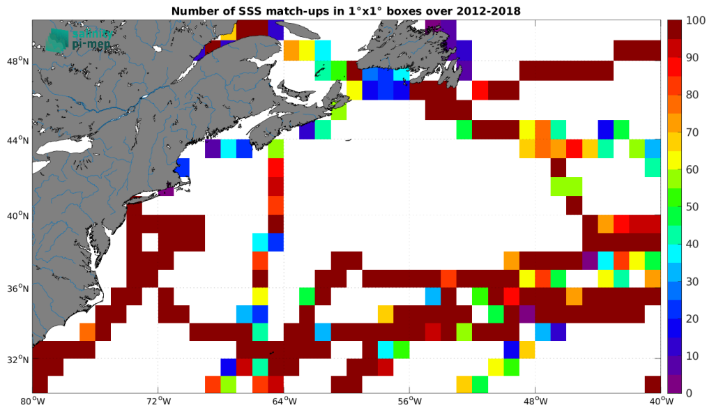
Figure 5: Number of SSS match-ups between TSG (GOSUD-Sailing-ship) SSS and the SMOS SSS L4 OI v346 - Weekly (CMEMS-CATDS-LOPS) SSS product for the Gulf Stream Pi-MEP region over 1^\circ \times 1^\circ boxes and for the full satellite product period.
