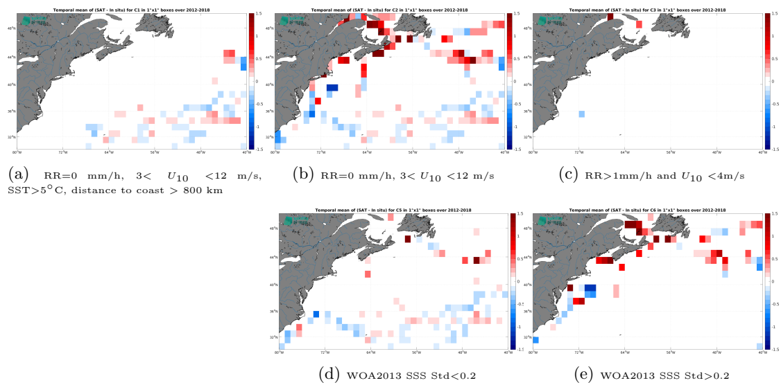
Figure 14: Temporal mean gridded over spatial boxes of size 1^\circ \times 1^\circ of \Delta SSS (SMOS SSS L4 OI v346 - Weekly (CMEMS-CATDS-LOPS) - TSG (GOSUD-Sailing-ship)) for 5 different sub-datasets corresponding to:RR=0 mm/h, 3 < U_{10} < 12 m/s, SST >5^\circ C , distance to coast > 800 km (a), RR=0 mm/h, 3 < U_{10} < 12 m/s (b), RR >1 mm/h and U_{10} < 4 m/s (c), WOA2013 SSS Std <0.2 (d), WOA2013 SSS Std >0.2 (e).
