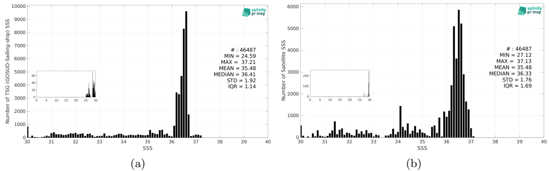
Figure 3: Histograms of SSS from TSG (GOSUD-Sailing-ship) (a) and SMOS SSS L4 OI v346 - Weekly (CMEMS-CATDS-LOPS) (b) considering all match-up pairs per bins of 0.1 over the Gulf Stream Pi-MEP region and for the full satellite product period.
