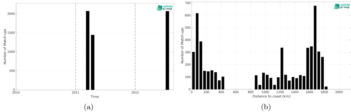
Figure 2: Number of match-ups between TSG (CSIC-UTM) and SMOS SSS L4 OI v346 - Weekly (CMEMS-CATDS-LOPS) SSS as a function of time (a) and as function of the distance to coast (b) over the Gulf Stream Pi-MEP region and for the full satellite product period.
