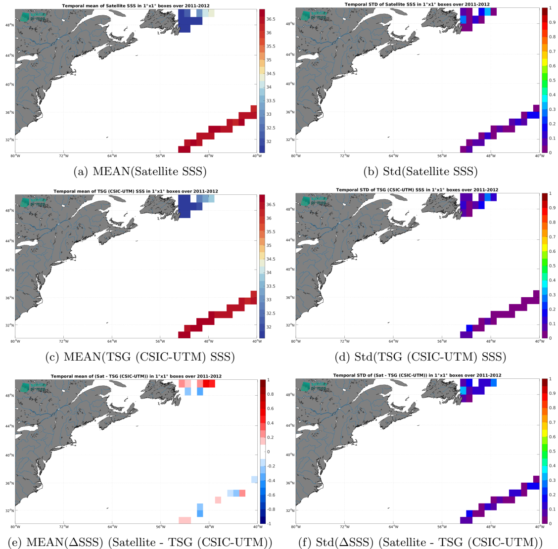
Figure 7: Temporal mean (left) and Std (right) of SSS from SMOS SSS L4 OI v346 - Weekly (CMEMS-CATDS-LOPS) (top), TSG (CSIC-UTM) (middle), and of \Delta SSS (Satellite - TSG (CSIC-UTM)). Only match-up pairs are used to generate these maps.
