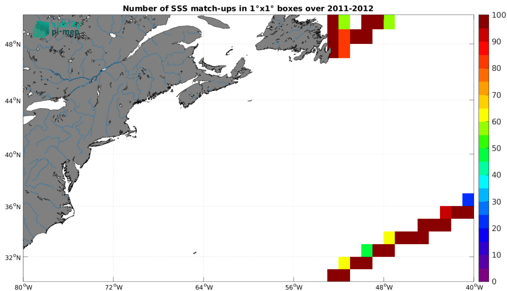
Figure 5: Number of SSS match-ups between TSG (CSIC-UTM) SSS and the SMOS SSS L4 OI v346 - Weekly (CMEMS-CATDS-LOPS) SSS product for the Gulf Stream Pi-MEP region over 1^\circ \times 1^\circ boxes and for the full satellite product period.
