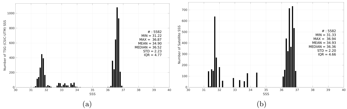
Figure 3: Histograms of SSS from TSG (CSIC-UTM) (a) and SMOS SSS L4 OI v346 - Weekly (CMEMS-CATDS-LOPS) (b) considering all match-up pairs per bins of 0.1 over the Gulf Stream Pi-MEP region and for the full satellite product period.
