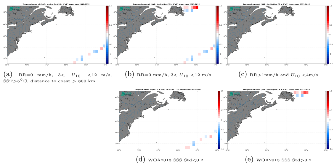
Figure 14: Temporal mean gridded over spatial boxes of size 1^\circ \times 1^\circ of \Delta\text{SSS} (SMOS SSS L4 OI v346 - Weekly (CMEMS-CATDS-LOPS) - TSG (CSIC-UTM)) for 5 different subdatasets corresponding to:RR=0 mm/h, 3 < U_{10} < 12 m/s, SST >5^\circ\text{C} , distance to coast > 800 km (a), RR=0 mm/h, 3 < U_{10} < 12 m/s (b), RR >1 mm/h and U_{10} < 4 m/s (c), WOA2013 SSS Std <0.2 (d), WOA2013 SSS Std >0.2 (e).
