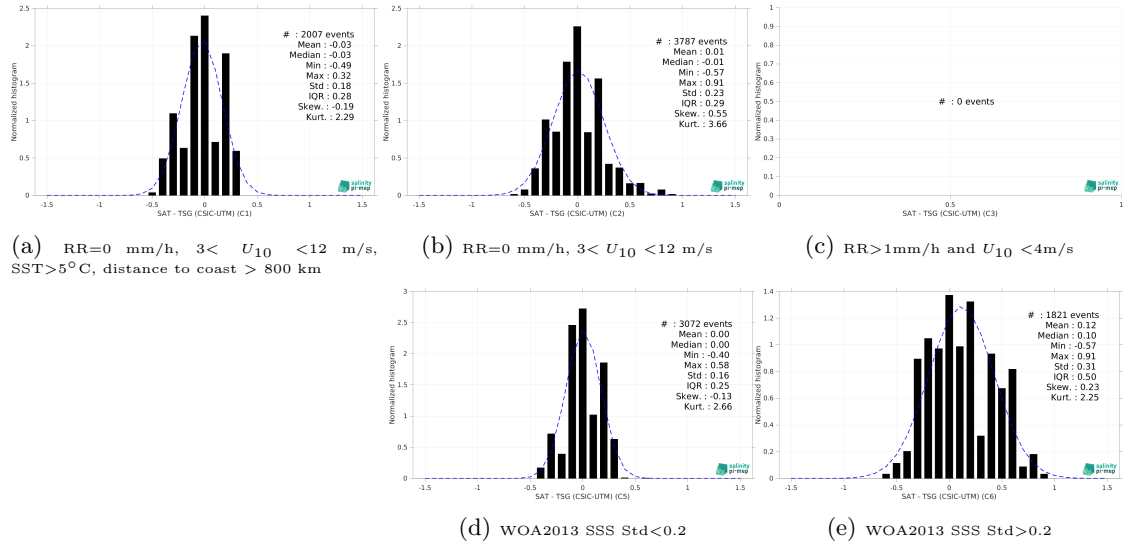
Figure 15: Normalized histogram of \Delta SSS (SMOS SSS L4 OI v346 - Weekly (CMEMS-CATDS-LOPS) - TSG (CSIC-UTM)) for 5 different subdatasets corresponding to: RR=0 mm/h, 3 < U_{10} < 12 m/s, SST > 5°C, distance to coast > 800 km (a), RR=0 mm/h, 3 < U_{10} < 12 m/s (b), RR > 1mm/h and U_{10} < 4 m/s (c), WOA2013 SSS Std < 0.2 (d), WOA2013 SSS Std > 0.2 (e).
