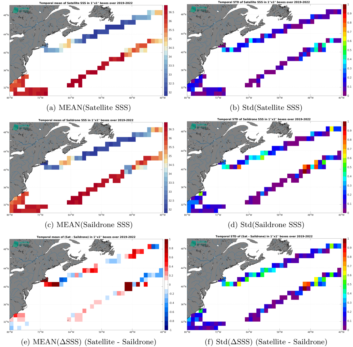
Figure 7: Temporal mean (left) and Std (right) of SSS from SMOS SSS L4 OI v346 - Weekly (CMEMS-CATDS-LOPS) (top), Saildrone (middle), and of \Delta SSS (Satellite - Saildrone). Only match-up pairs are used to generate these maps.
