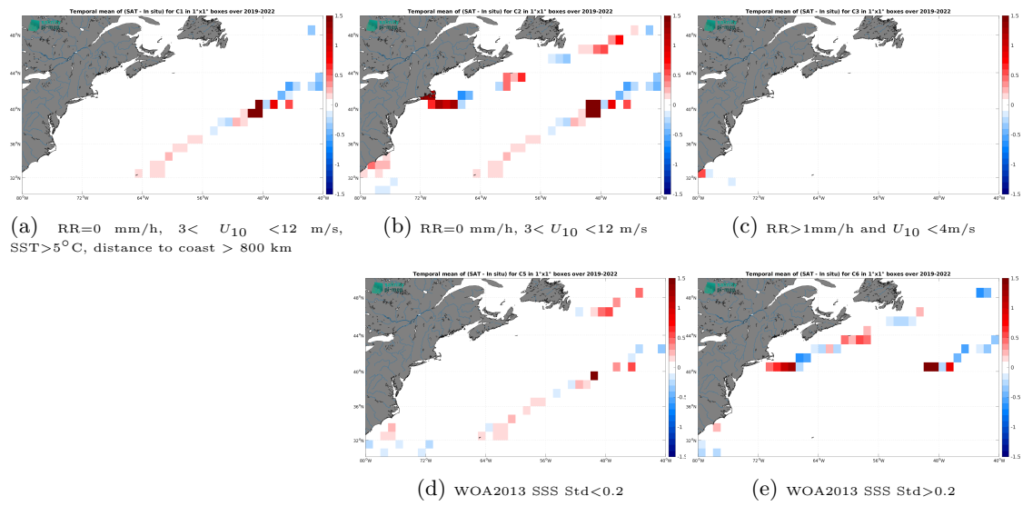
Figure 14: Temporal mean gridded over spatial boxes of size 1^\circ \times 1^\circ of \Delta SSS (SMOS SSS L4 OI v346 - Weekly (CMEMS-CATDS-LOPS) - Saildrone) for 5 different subdatasets corresponding to:RR=0 mm/h, 3 < U_{10} < 12 m/s, SST >5^\circ\text{C} , distance to coast > 800 km (a), RR=0 mm/h, 3 < U_{10} < 12 m/s (b), RR >1 mm/h and U_{10} < 4 m/s (c), WOA2013 SSS Std <0.2 (d), WOA2013 SSS Std >0.2 (e).
