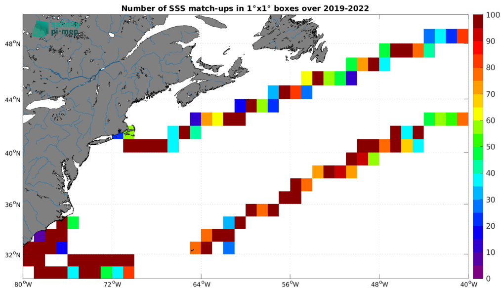
Figure 5: Number of SSS match-ups between Saildrone SSS and the SMOS SSS L4 OI v346 - Weekly (CMEMS-CATDS-LOPS) SSS product for the Gulf Stream Pi-MEP region over 1^\circ \times 1^\circ boxes and for the full satellite product period.
