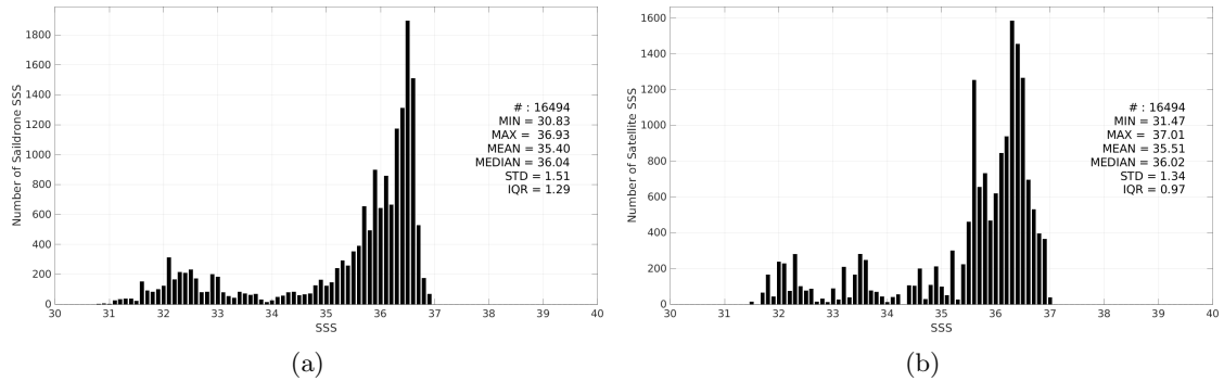
Figure 3: Histograms of SSS from Saildrone (a) and SMOS SSS L4 OI v346 - Weekly (CMEMS-CATDS-LOPS) (b) considering all match-up pairs per bins of 0.1 over the Gulf Stream Pi-MEP region and for the full satellite product period.
