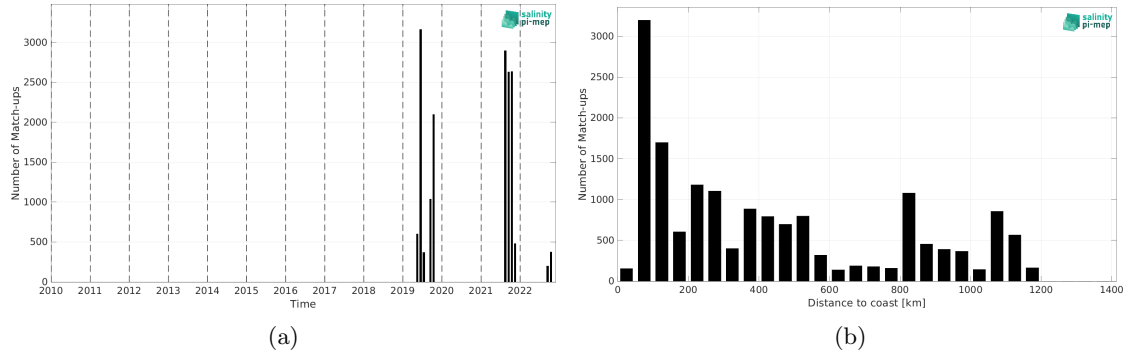
Figure 2: Number of match-ups between Saildrone and SMOS SSS L4 OI v346 - Weekly (CMEMS-CATDS-LOPS) SSS as a function of time (a) and as function of the distance to coast (b) over the Gulf Stream Pi-MEP region and for the full satellite product period.
