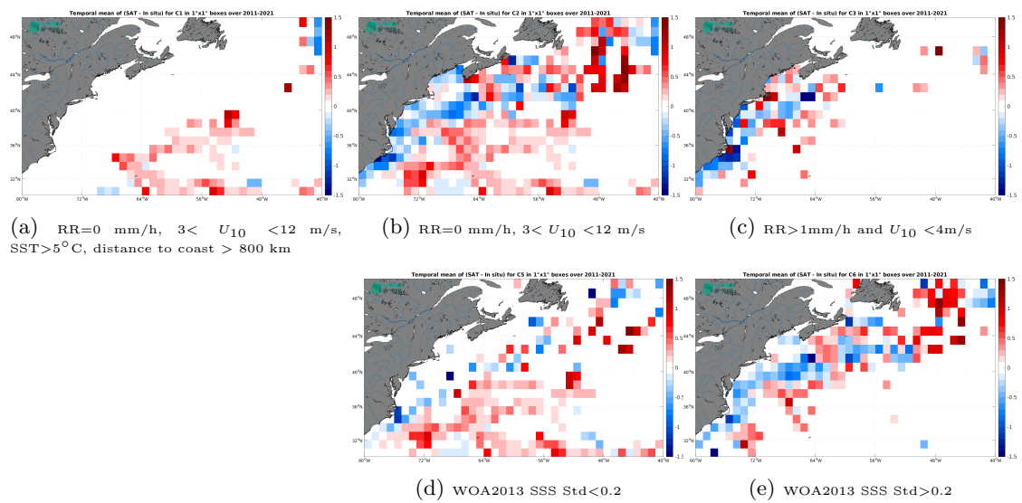
Figure 14: Temporal mean gridded over spatial boxes of size 1^\circ \times 1^\circ of \Delta SSS (SMOS SSS L4 v2 - Daily (BEC) - TSG (SAMOS)) for 5 different subdatasets corresponding to:RR=0 mm/h, 3 < U_{10} < 12 m/s, SST>5°C, distance to coast > 800 km (a), RR=0 mm/h, 3 < U_{10} < 12 m/s (b), RR>1mm/h and U_{10} < 4 m/s (c), WOA2013 SSS Std<0.2 (d), WOA2013 SSS Std>0.2 (e).
