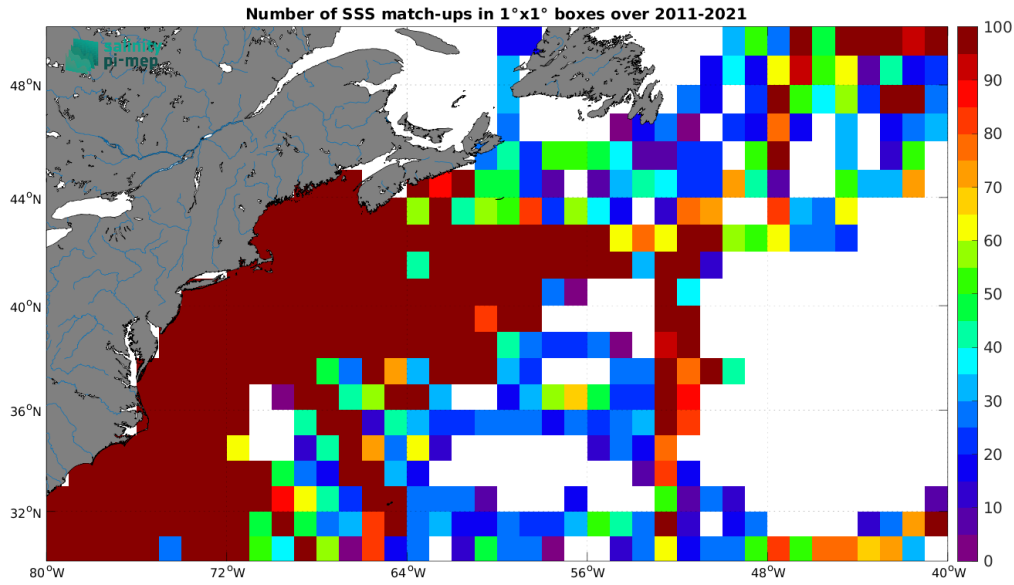
Figure 5: Number of SSS match-ups between TSG (SAMOS) SSS and the SMOS SSS L4 v2 - Daily (BEC) SSS product for the Gulf Stream Pi-MEP region over 1^\circ \times 1^\circ boxes and for the full satellite product period.
