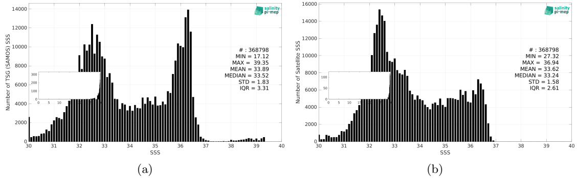
Figure 3: Histograms of SSS from TSG (SAMOS) (a) and SMOS SSS L4 v2 - Daily (BEC) (b) considering all match-up pairs per bins of 0.1 over the Gulf Stream Pi-MEP region and for the full satellite product period.
