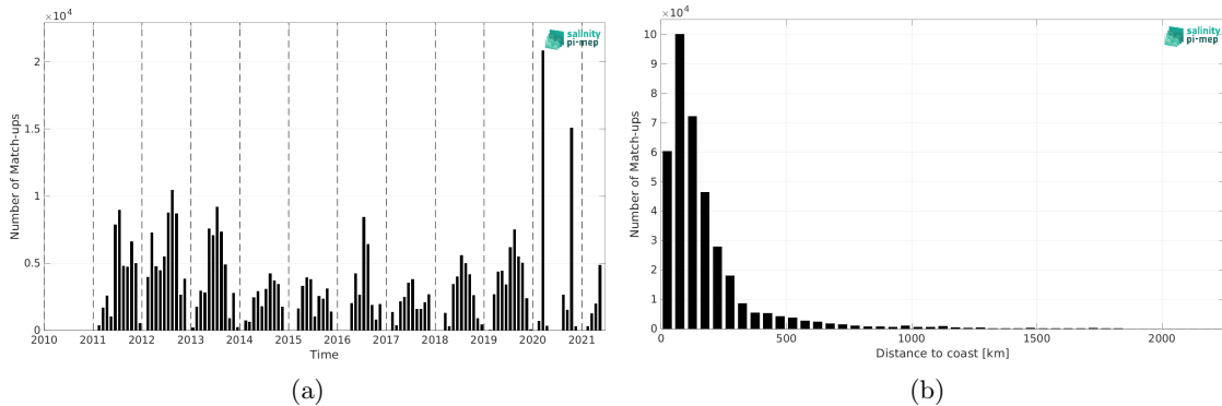
Figure 2: Number of match-ups between TSG (SAMOS) and SMOS SSS L4 v2 - Daily (BEC) SSS as a function of time (a) and as function of the distance to coast (b) over the Gulf Stream Pi-MEP region and for the full satellite product period.
