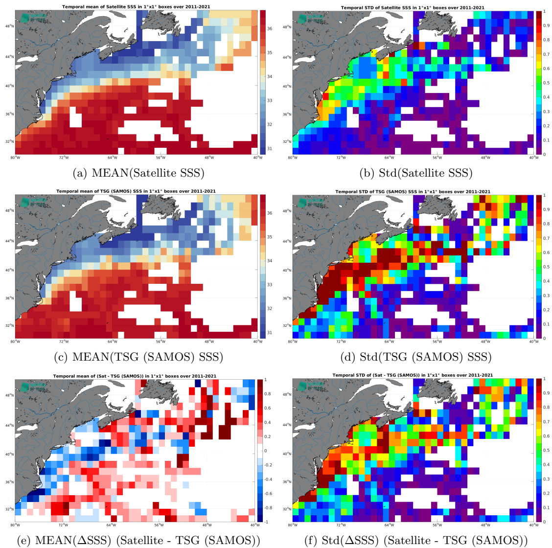
Figure 7: Temporal mean (left) and Std (right) of SSS from SMOS SSS L4 v2 - Daily (BEC) (top), TSG (SAMOS) (middle), and of \Delta SSS (Satellite - TSG (SAMOS)). Only match-up pairs are used to generate these maps.
