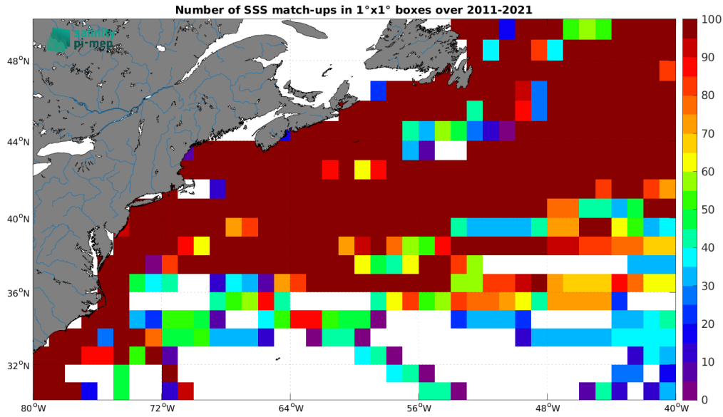
Figure 4: Number of SSS match-ups between TSG (LEGOS-DM) SSS and the SMOS SSS L4 v2 - Daily (BEC) SSS product for the Gulf Stream Pi-MEP region over 1^{\circ} \times 1^{\circ} boxes and for the full satellite product period.
