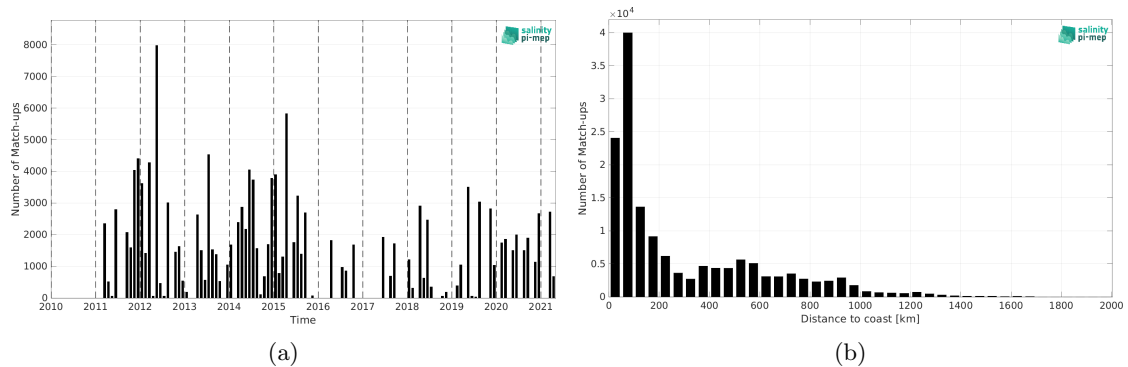
Figure 1: Number of match-ups between TSG (LEGOS-DM) and SMOS SSS L4 v2 - Daily (BEC) SSS as a function of time (a) and as function of the distance to coast (b) over the Gulf Stream Pi-MEP region and for the full satellite product period.
