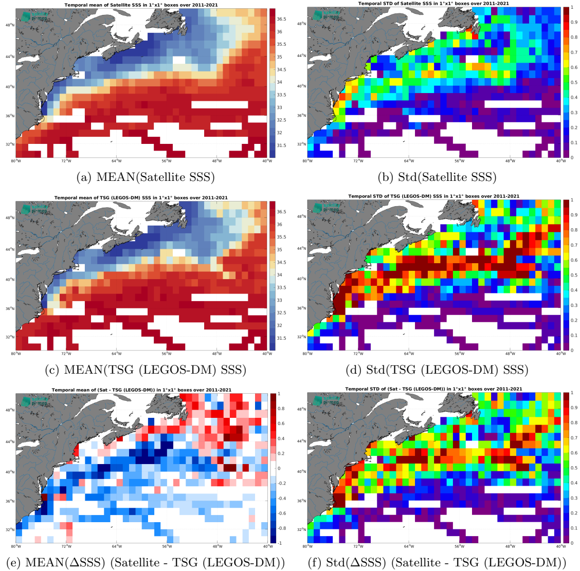
Figure 6: Temporal mean (left) and Std (right) of SSS from SMOS SSS L4 v2 - Daily (BEC) (top), TSG (LEGOS-DM) (middle), and of \Delta SSS (Satellite - TSG (LEGOS-DM)). Only match-up pairs are used to generate these maps.
