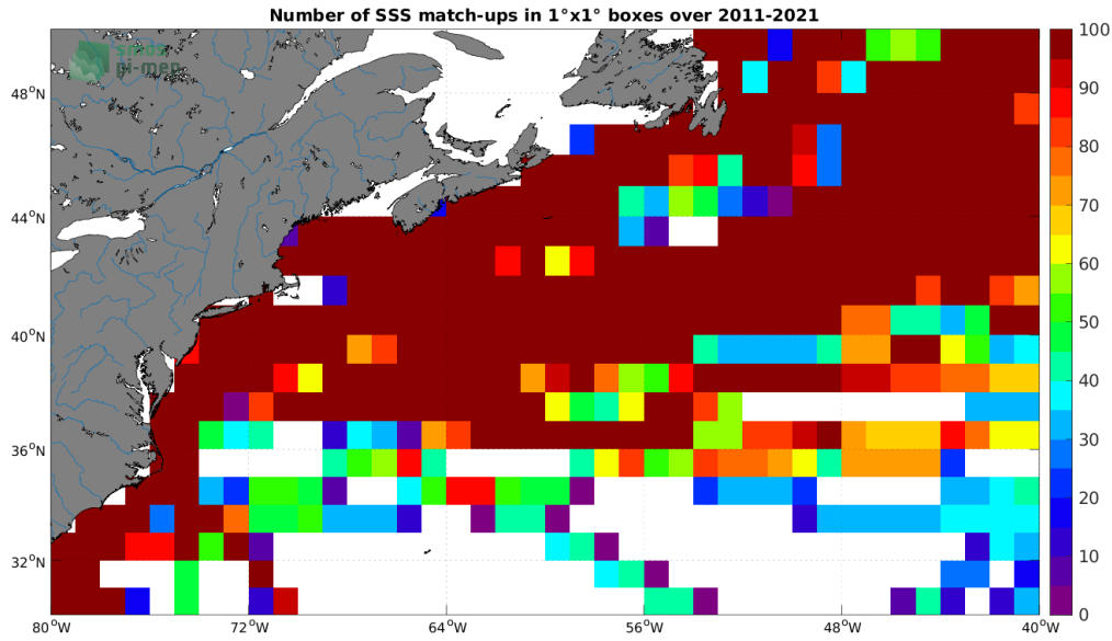
Figure 4: Number of SSS match-ups between TSG (LEGOS-DM) SSS and the SMOS SSS L4 v2 - Daily (BEC) SSS product for the Gulf Stream Pi-MEP region over 1^\circ \times 1^\circ boxes and for the full satellite product period.
