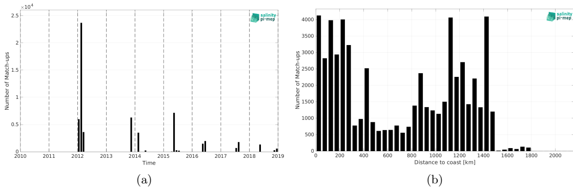
Figure 2: Number of match-ups between TSG (GOSUD-Sailing-ship) and SMOS SSS L4 v2 - Daily (BEC) SSS as a function of time (a) and as function of the distance to coast (b) over the Gulf Stream Pi-MEP region and for the full satellite product period.
