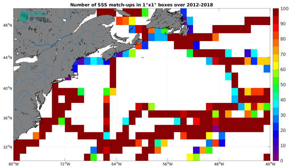
Figure 5: Number of SSS match-ups between TSG (GOSUD-Sailing-ship) SSS and the SMOS SSS L4 v2 - Daily (BEC) SSS product for the Gulf Stream Pi-MEP region over 1^\circ \times 1^\circ boxes and for the full satellite product period.
