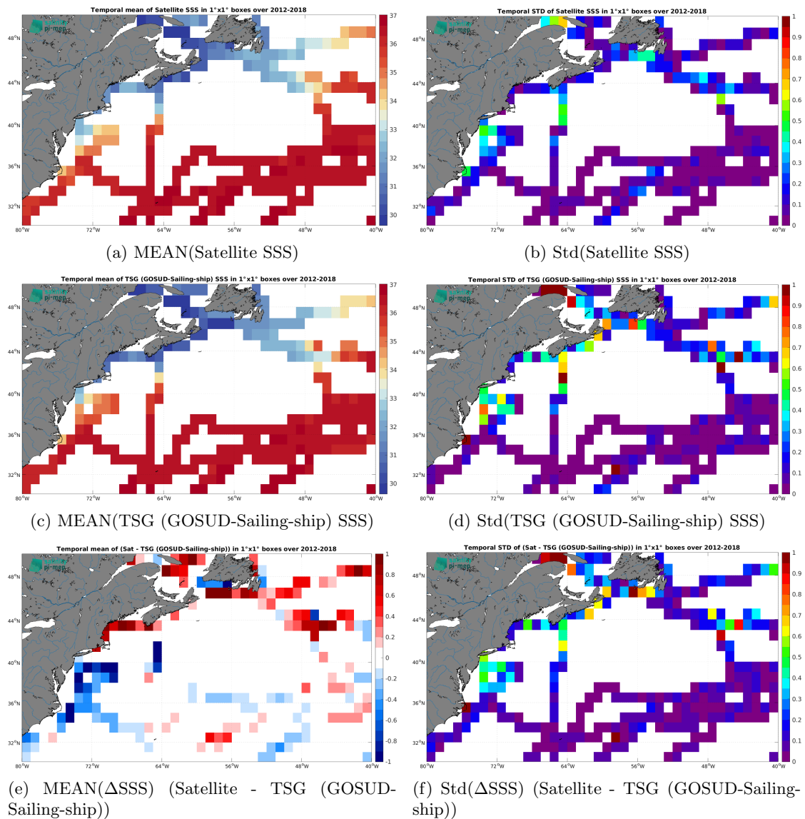
Figure 7: Temporal mean (left) and Std (right) of SSS from SMOS SSS L4 v2 - Daily (BEC) (top), TSG (GOSUD-Sailing-ship) (middle), and of \Delta SSS (Satellite - TSG (GOSUD-Sailing-ship)). Only match-up pairs are used to generate these maps.
