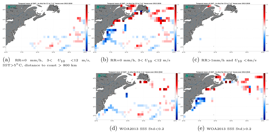
Figure 14: Temporal mean gridded over spatial boxes of size 1^\circ \times 1^\circ of \Delta SSS (SMOS SSS L4 v2 - Daily (BEC) - TSG (GOSUD-Sailing-ship)) for 5 different subdatasets corresponding to:RR=0 mm/h, 3 < U_{10} < 12 m/s, SST > 5°C, distance to coast > 800 km (a), RR=0 mm/h, 3 < U_{10} < 12 m/s (b), RR > 1mm/h and U_{10} < 4 m/s (c), WOA2013 SSS Std < 0.2 (d), WOA2013 SSS Std > 0.2 (e).
