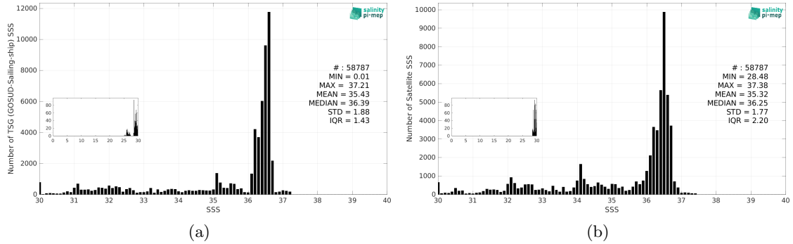
Figure 3: Histograms of SSS from TSG (GOSUD-Sailing-ship) (a) and SMOS SSS L4 v2 - Daily (BEC) (b) considering all match-up pairs per bins of 0.1 over the Gulf Stream Pi-MEP region and for the full satellite product period.
