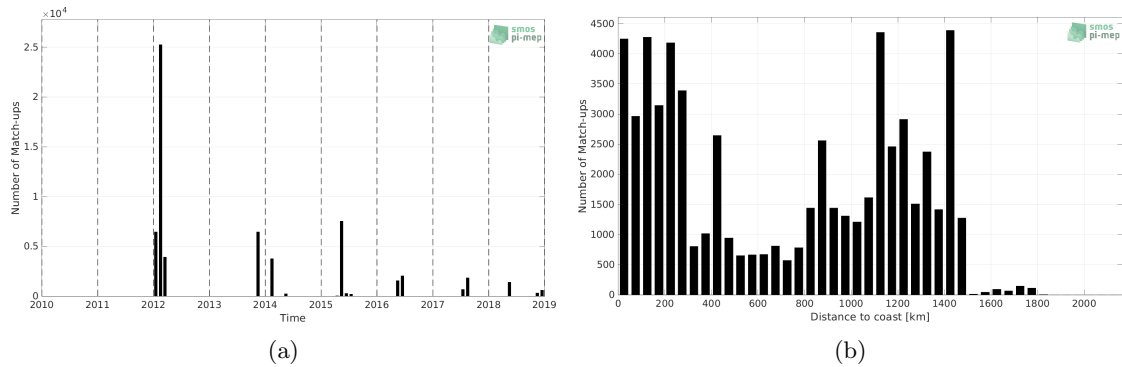
Figure 1: Number of match-ups between TSG (GOSUD-Sailing-ship) and SMOS SSS L4 v2 - Daily (BEC) SSS as a function of time (a) and as function of the distance to coast (b) over the Gulf Stream Pi-MEP region and for the full satellite product period.
