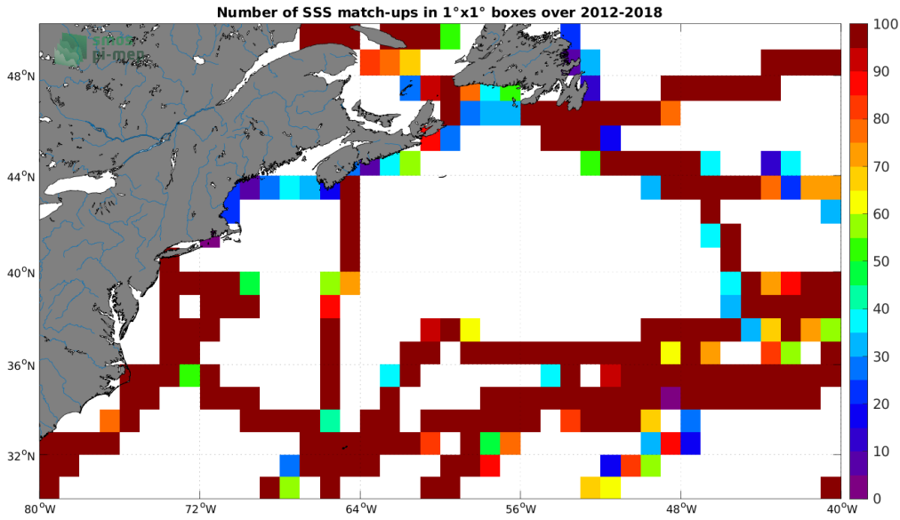
Figure 4: Number of SSS match-ups between TSG (GOSUD-Sailing-ship) SSS and the SMOS SSS L4 v2 - Daily (BEC) SSS product for the Gulf Stream Pi-MEP region over 1^\circ \times 1^\circ boxes and for the full satellite product period.
