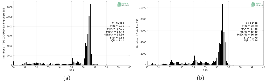
Figure 2: Histograms of SSS from TSG (GOSUD-Sailing-ship) (a) and SMOS SSS L4 v2 - Daily (BEC) (b) considering all match-up pairs per bins of 0.1 over the Gulf Stream Pi-MEP region and for the full satellite product period.
