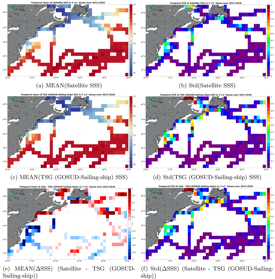
Figure 6: Temporal mean (left) and Std (right) of SSS from SMOS SSS L4 v2 - Daily (BEC) (top), TSG (GOSUD-Sailing-ship) (middle), and of \Delta SSS (Satellite - TSG (GOSUD-Sailing-ship)). Only match-up pairs are used to generate these maps.
