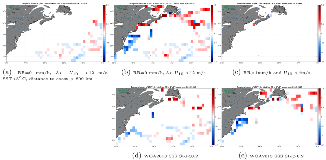
Figure 12: Temporal mean gridded over spatial boxes of size 1^\circ \times 1^\circ of \Delta SSS (SMOS SSS L4 v2 - Daily (BEC) - TSG (GOSUD-Sailing-ship)) for 5 different subdatasets corresponding to:RR=0 mm/h, 3 < U_{10} < 12 m/s, SST > 5°C, distance to coast > 800 km (a), RR=0 mm/h, 3 < U_{10} < 12 m/s (b), RR > 1mm/h and U_{10} < 4 m/s (c), WOA2013 SSS Std < 0.2 (d), WOA2013 SSS Std > 0.2 (e).
