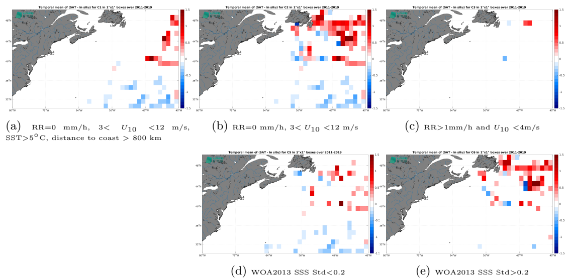
Figure 14: Temporal mean gridded over spatial boxes of size 1^\circ \times 1^\circ of \Delta SSS (SMOS SSS L4 v2 - Daily (BEC) - TSG (GOSUD-Research-vessel)) for 5 different subdatasets corresponding to:RR=0 mm/h, 3 < U_{10} < 12 m/s, SST >5^\circ C, distance to coast > 800 km (a), RR=0 mm/h, 3 < U_{10} < 12 m/s (b), RR >1 mm/h and U_{10} < 4 m/s (c), WOA2013 SSS Std <0.2 (d), WOA2013 SSS Std >0.2 (e).
