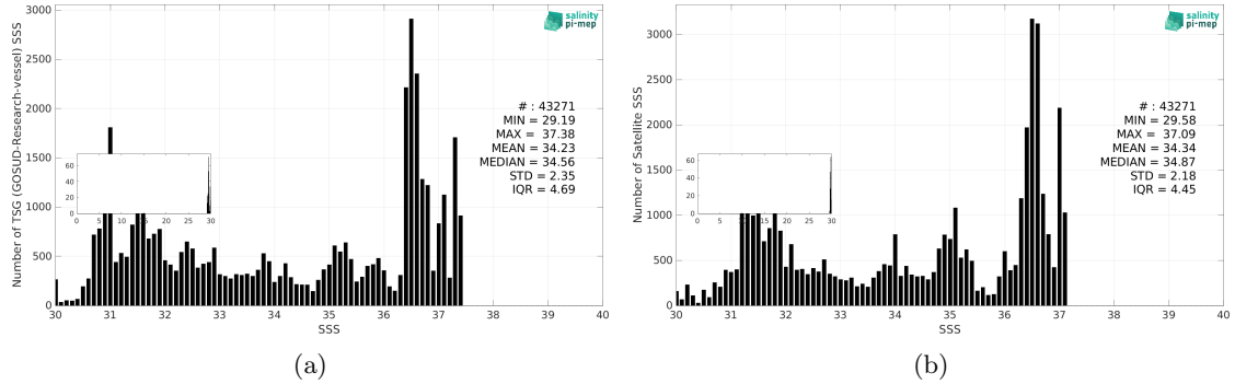
Figure 3: Histograms of SSS from TSG (GOSUD-Research-vessel) (a) and SMOS SSS L4 v2 - Daily (BEC) (b) considering all match-up pairs per bins of 0.1 over the Gulf Stream Pi-MEP region and for the full satellite product period.
