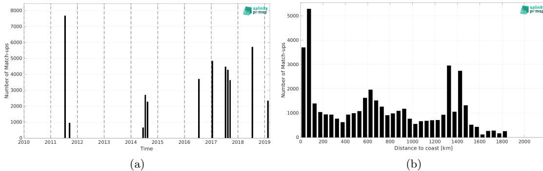
Figure 2: Number of match-ups between TSG (GOSUD-Research-vessel) and SMOS SSS L4 v2 - Daily (BEC) SSS as a function of time (a) and as function of the distance to coast (b) over the Gulf Stream Pi-MEP region and for the full satellite product period.
