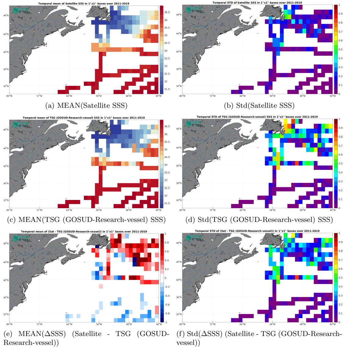
Figure 7: Temporal mean (left) and Std (right) of SSS from SMOS SSS L4 v2 - Daily (BEC) (top), TSG (GOSUD-Research-vessel) (middle), and of \Delta SSS (Satellite - TSG (GOSUD-Research-vessel)). Only match-up pairs are used to generate these maps.
