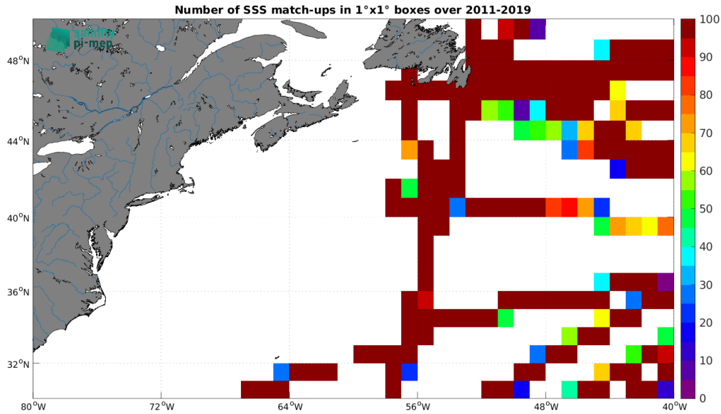
Figure 5: Number of SSS match-ups between TSG (GOSUD-Research-vessel) SSS and the SMOS SSS L4 v2 - Daily (BEC) SSS product for the Gulf Stream Pi-MEP region over 1^\circ \times 1^\circ boxes and for the full satellite product period.
