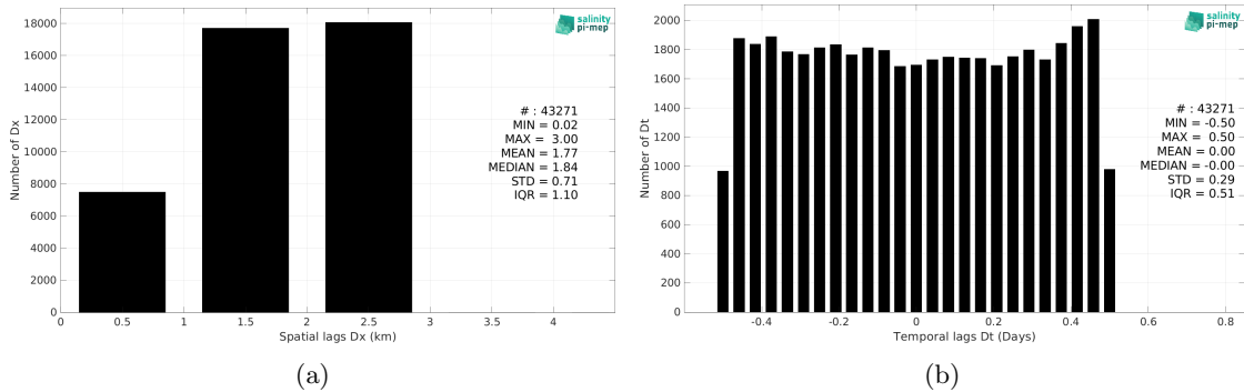
Figure 6: Histograms of the spatial (a) and temporal (b) lags between the location/time of the TSG (GOSUD-Research-vessel) measurement and the date of the corresponding SMOS SSS L4 v2 - Daily (BEC) SSS pixel.
