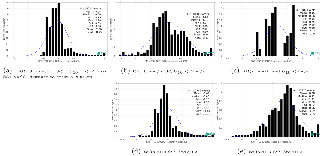
Figure 15: Normalized histogram of \Delta SSS (SMOS SSS L4 v2 - Daily (BEC) - TSG (GOSUD-Research-vessel)) for 5 different subdatasets corresponding to: RR=0 mm/h, 3 < U_{10} < 12 m/s, SST>5°C, distance to coast > 800 km (a), RR=0 mm/h, 3 < U_{10} < 12 m/s (b), RR>1mm/h and U_{10} < 4 m/s (c), WOA2013 SSS Std<0.2 (d), WOA2013 SSS Std>0.2 (e).
