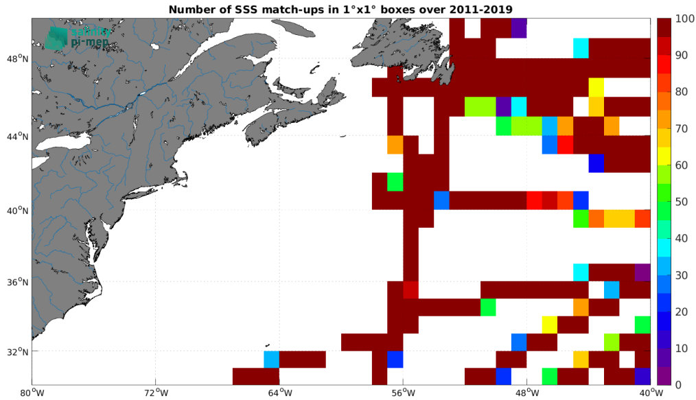
Figure 4: Number of SSS match-ups between TSG (GOSUD-Research-vessel) SSS and the SMOS SSS L4 v2 - Daily (BEC) SSS product for the Gulf Stream Pi-MEP region over 1^\circ \times 1^\circ boxes and for the full satellite product period.
