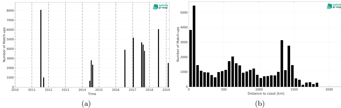
Figure 1: Number of match-ups between TSG (GOSUD-Research-vessel) and SMOS SSS L4 v2 - Daily (BEC) SSS as a function of time (a) and as function of the distance to coast (b) over the Gulf Stream Pi-MEP region and for the full satellite product period.
