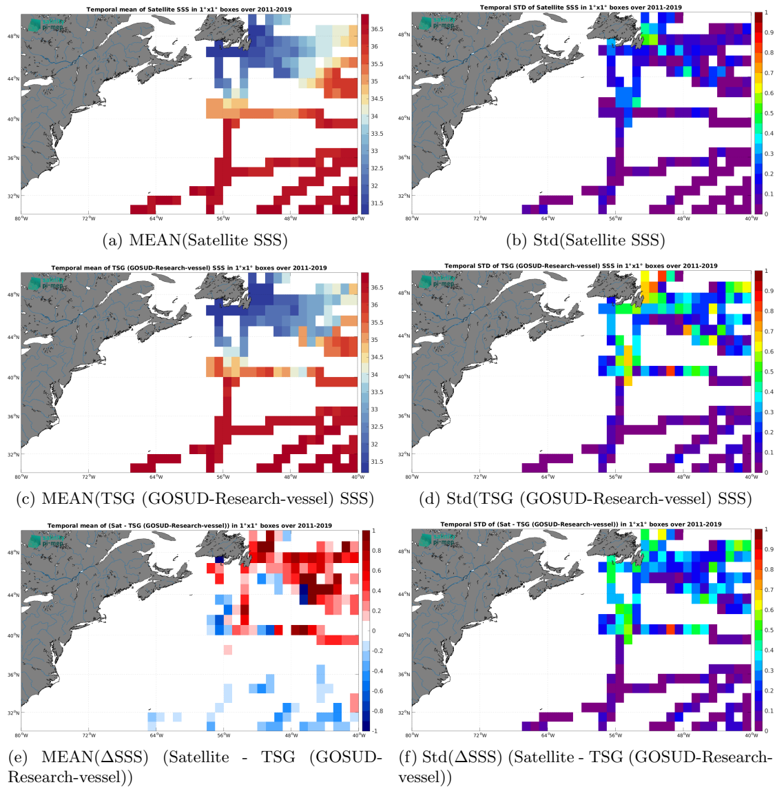
Figure 6: Temporal mean (left) and Std (right) of SSS from SMOS SSS L4 v2 - Daily (BEC) (top), TSG (GOSUD-Research-vessel) (middle), and of \Delta SSS (Satellite - TSG (GOSUD-Research-vessel)). Only match-up pairs are used to generate these maps.
