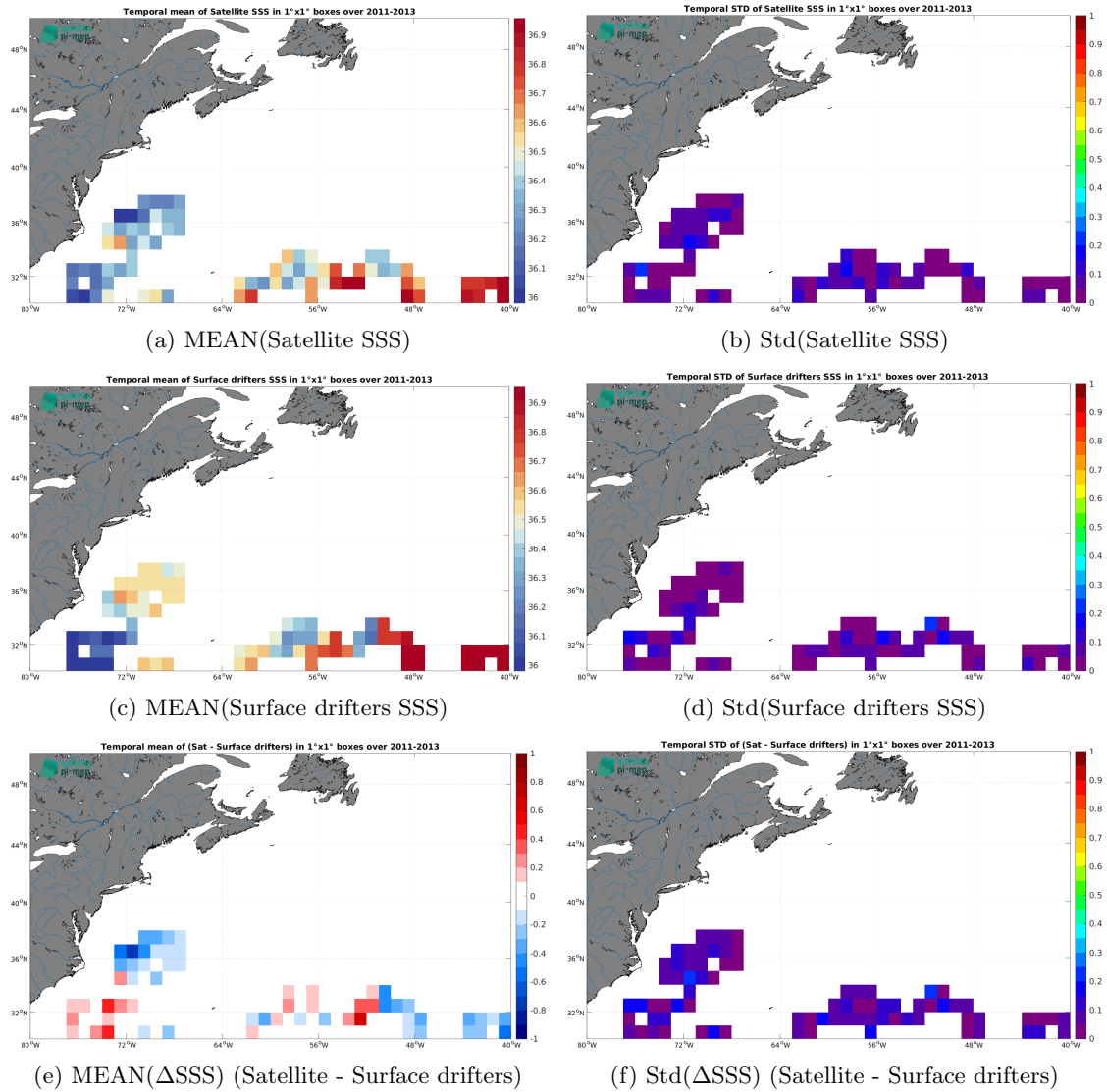
Figure 6: Temporal mean (left) and Std (right) of SSS from SMOS SSS L4 v2 - Daily (BEC) (top), Surface drifters (middle), and of \Delta SSS (Satellite - Surface drifters). Only match-up pairs are used to generate these maps.
