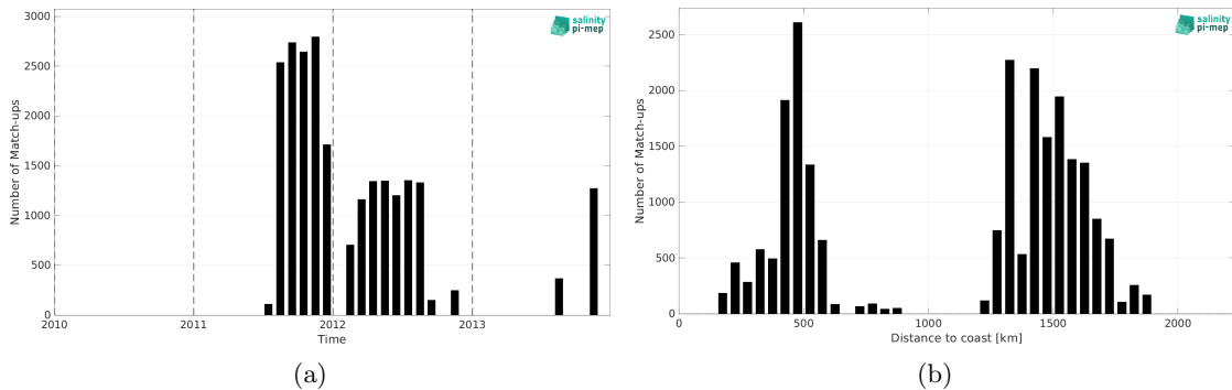
Figure 2: Number of match-ups between Surface drifters and SMOS SSS L4 v2 - Daily (BEC) SSS as a function of time (a) and as function of the distance to coast (b) over the Gulf Stream Pi-MEP region and for the full satellite product period.
