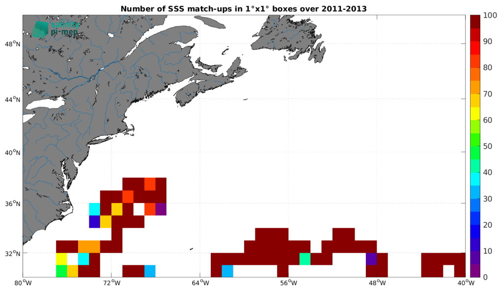
Figure 4: Number of SSS match-ups between Surface drifters SSS and the SMOS SSS L4 v2 - Daily (BEC) SSS product for the Gulf Stream Pi-MEP region over 1^\circ \times 1^\circ boxes and for the full satellite product period.
