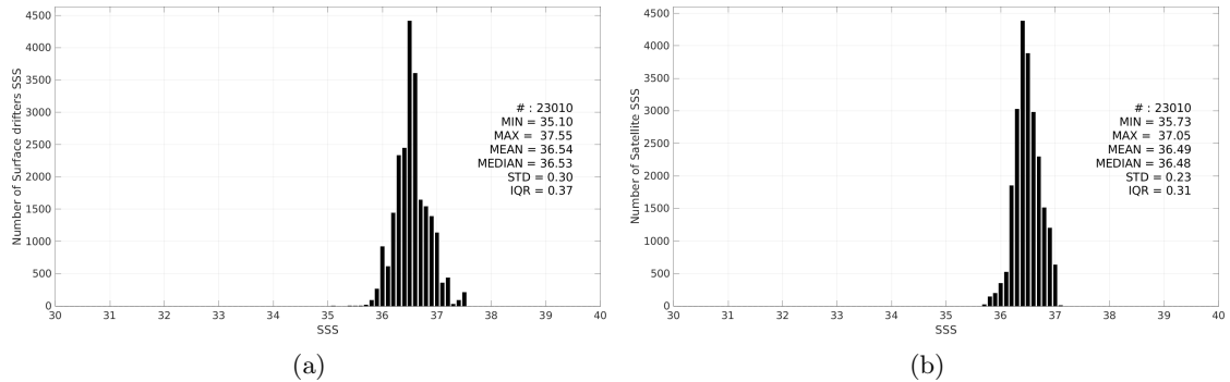
Figure 3: Histograms of SSS from Surface drifters (a) and SMOS SSS L4 v2 - Daily (BEC) (b) considering all match-up pairs per bins of 0.1 over the Gulf Stream Pi-MEP region and for the full satellite product period.
