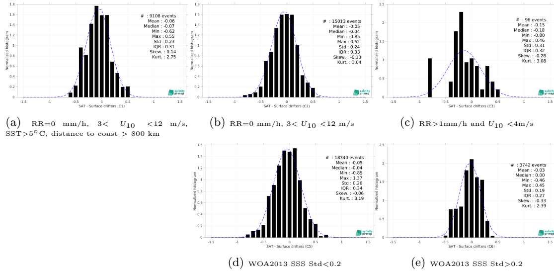
Figure 14: Normalized histogram of \Delta\text{SSS} (SMOS SSS L4 v2 - Daily (BEC) - Surface drifters) for 5 different subdatasets corresponding to: RR=0 mm/h, 3 < U_{10} < 12 m/s, SST > 5^\circ\text{C} , distance to coast > 800 km (a), RR=0 mm/h, 3 < U_{10} < 12 m/s (b), RR > 1 mm/h and U_{10} < 4 m/s (c), WOA2013 SSS Std < 0.2 (d), WOA2013 SSS Std > 0.2 (e).
