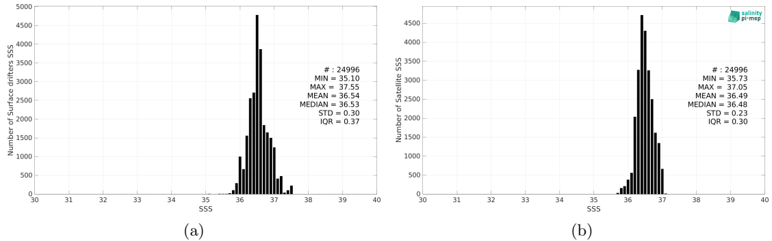
Figure 2: Histograms of SSS from Surface drifters (a) and SMOS SSS L4 v2 - Daily (BEC) (b) considering all match-up pairs per bins of 0.1 over the Gulf Stream Pi-MEP region and for the full satellite product period.
