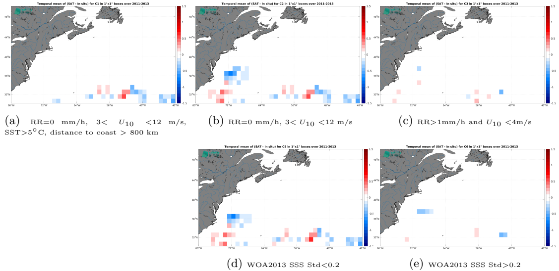
Figure 11: Temporal mean gridded over spatial boxes of size 1^{\circ}\times 1^{\circ} of \Delta\text{SSS} (SMOS SSS L4 v2 - Daily (BEC) - Surface drifters) for 5 different subdatasets corresponding to:RR=0 mm/h, 3 < U_{10} < 12 m/s, \text{SST} > 5^{\circ}\text{C} , distance to coast > 800 km (a), RR=0 mm/h, 3 < U_{10} < 12 m/s (b), RR > 1 mm/h and U_{10} < 4 m/s (c), WOA2013 SSS Std < 0.2 (d), WOA2013 SSS Std > 0.2 (e).
