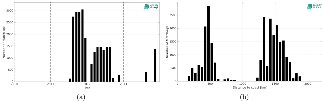
Figure 1: Number of match-ups between Surface drifters and SMOS SSS L4 v2 - Daily (BEC) SSS as a function of time (a) and as function of the distance to coast (b) over the Gulf Stream Pi-MEP region and for the full satellite product period.
