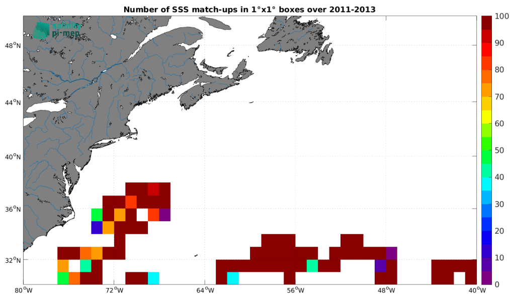
Figure 3: Number of SSS match-ups between Surface drifters SSS and the SMOS SSS L4 v2 - Daily (BEC) SSS product for the Gulf Stream Pi-MEP region over 1^\circ \times 1^\circ boxes and for the full satellite product period.
