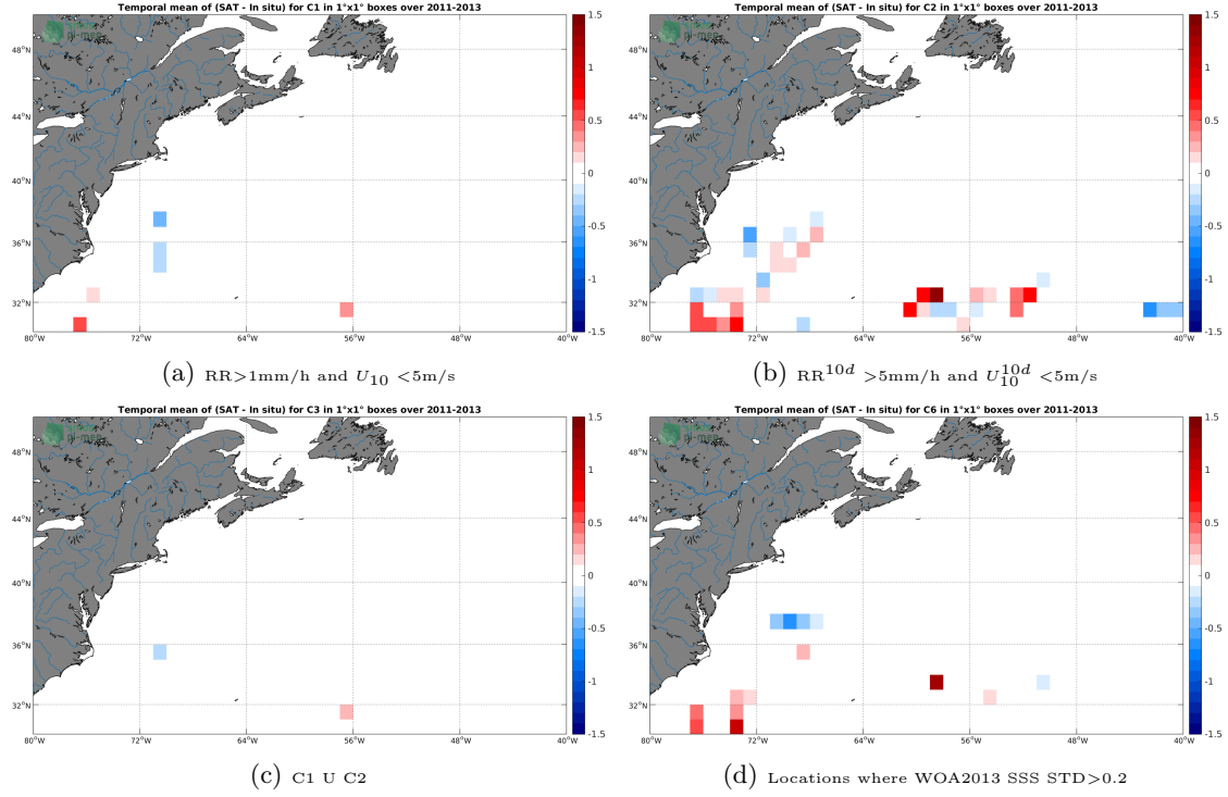
Figure 11: Temporal mean gridded over spatial boxes of size 1^\circ \times 1^\circ of \Delta SSS (SMOS-L3-ICDC-V3-MONTHLY-0.5DEG - Surface drifters) for 4 different subdatasets corresponding to: RR > 1\text{mm/h} and U_{10} < 5\text{m/s} (a), RR^{10d} > 5\text{mm/h} and U_{10}^{10d} < 5\text{m/s} (b), C1 U C2 (c), Locations where WOA2013 SSS STD > 0.2 (d).
