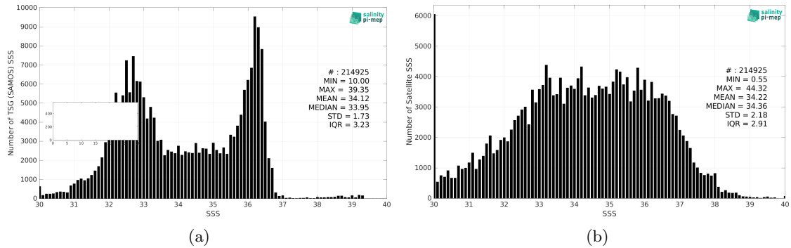
Figure 2: Histograms of SSS from TSG (SAMOS) (a) and SMOS SSS L2Q v331 - With FLAG (CMEMS-CATDS-CPDC) (b) considering all match-up pairs per bins of 0.1 over the Gulf Stream Pi-MEP region and for the full satellite product period.
