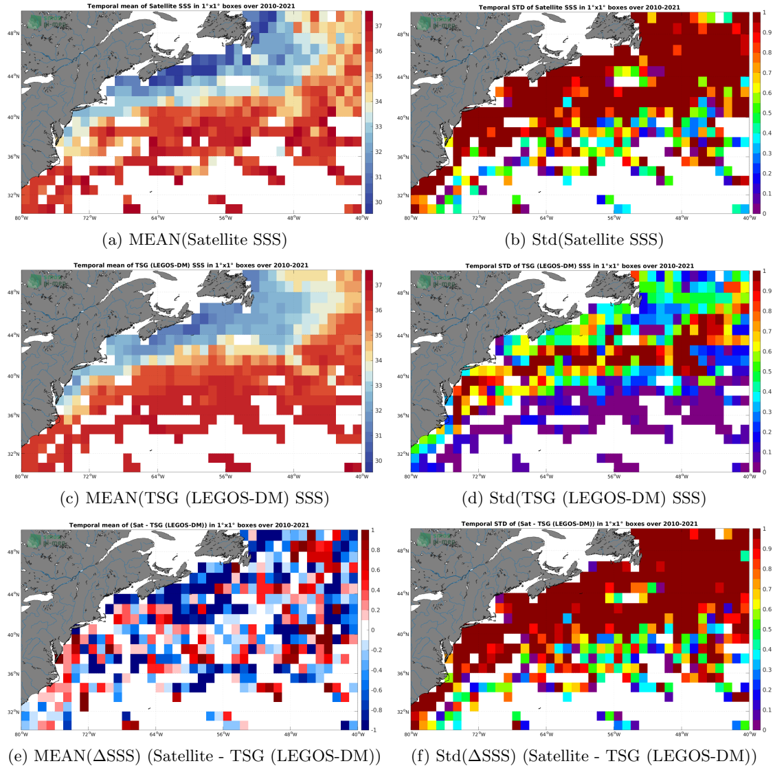
Figure 6: Temporal mean (left) and Std (right) of SSS from SMOS SSS L2Q v331 - With FLAG (CMEMS-CATDS-CPDC) (top), TSG (LEGOS-DM) (middle), and of \Delta SSS (Satellite - TSG (LEGOS-DM)). Only match-up pairs are used to generate these maps.
