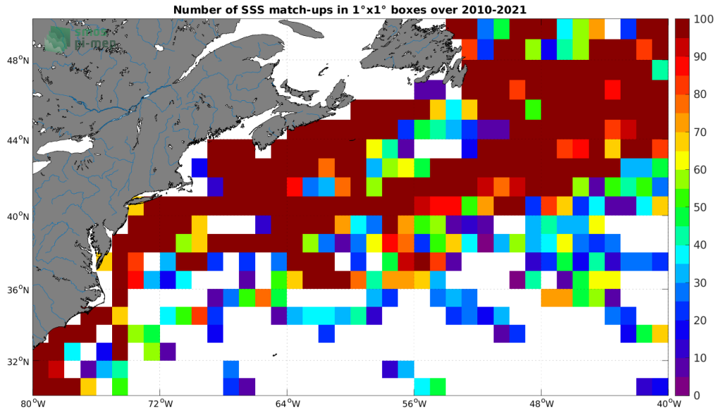
Figure 4: Number of SSS match-ups between TSG (LEGOS-DM) SSS and the SMOS SSS L2Q v331 - With FLAG (CMEMS-CATDS-CPDC) SSS product for the Gulf Stream Pi-MEP region over 1^\circ \times 1^\circ boxes and for the full satellite product period.
