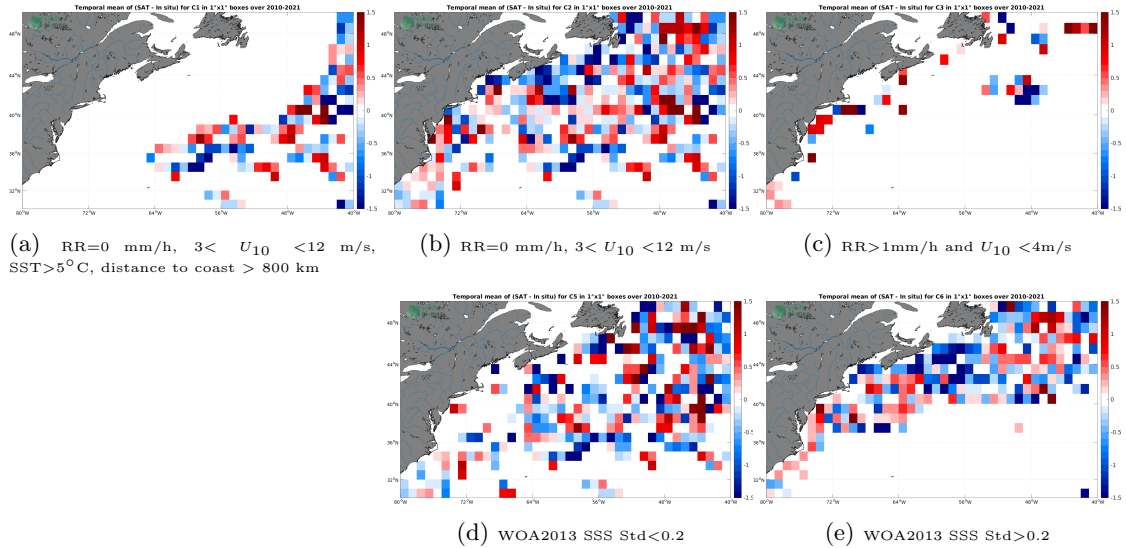
Figure 12: Temporal mean gridded over spatial boxes of size 1^{\circ}\times 1^{\circ} of \Delta\text{SSS} (SMOS SSS L2Q v331 - With FLAG (CMEMS-CATDS-CPDC) - TSG (LEGOS-DM)) for 5 different subdatasets corresponding to:RR=0 mm/h, 3 < U_{10} < 12 m/s, SST >5^{\circ}\text{C} , distance to coast > 800 km (a), RR=0 mm/h, 3 < U_{10} < 12 m/s (b), RR >1 mm/h and U_{10} < 4 m/s (c), WOA2013 SSS Std <0.2 (d), WOA2013 SSS Std >0.2 (e).
