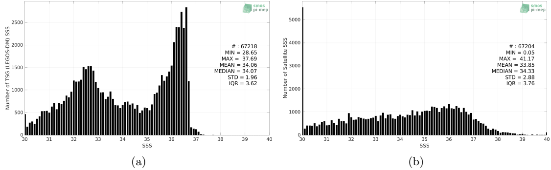
Figure 2: Histograms of SSS from TSG (LEGOS-DM) (a) and SMOS SSS L2Q v331 - With FLAG (CMEMS-CATDS-CPDC) (b) considering all match-up pairs per bins of 0.1 over the Gulf Stream Pi-MEP region and for the full satellite product period.
