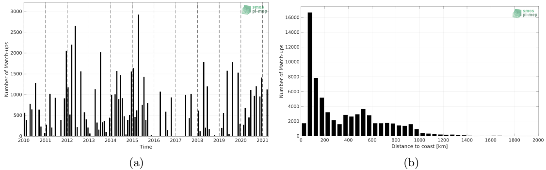
Figure 1: Number of match-ups between TSG (LEGOS-DM) and SMOS SSS L2Q v331 - With FLAG (CMEMS-CATDS-CPDC) SSS as a function of time (a) and as function of the distance to coast (b) over the Gulf Stream Pi-MEP region and for the full satellite product period.
