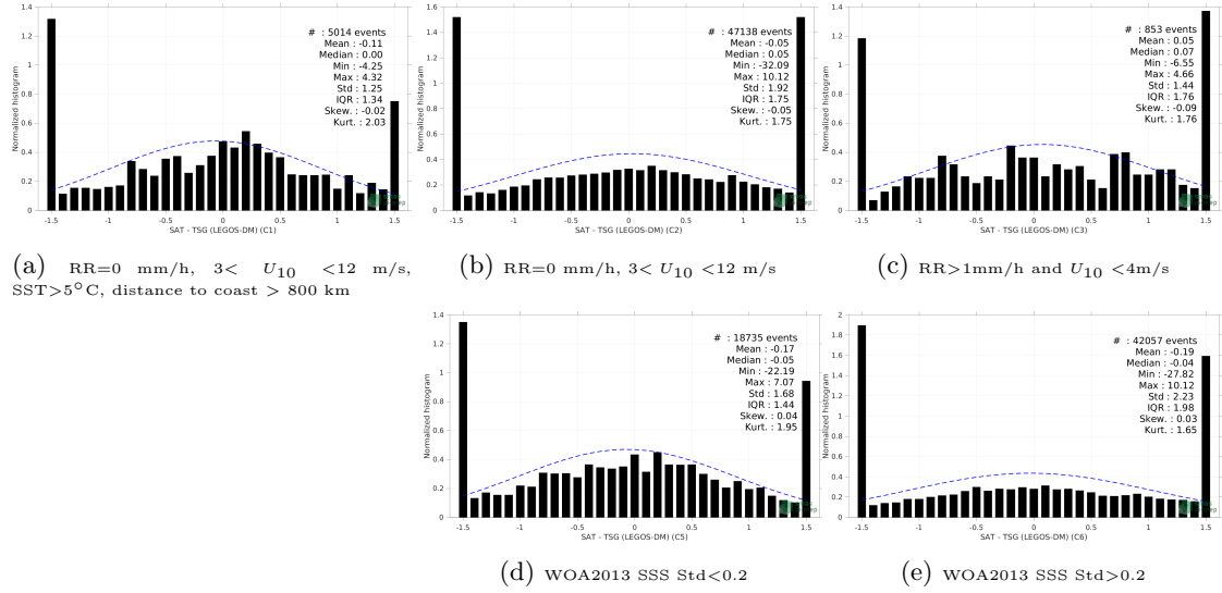
Figure 13: Normalized histogram of \Delta\text{SSS} (SMOS SSS L2Q v331 - With FLAG (CMEMS-CATDS-CPDC) - TSG (LEGOS-DM)) for 5 different subdatasets corresponding to: RR=0 mm/h, 3 < U_{10} < 12 m/s, SST > 5^\circ\text{C} , distance to coast > 800 km (a), RR=0 mm/h, 3 < U_{10} < 12 m/s (b), RR > 1 mm/h and U_{10} < 4 m/s (c), WOA2013 SSS Std < 0.2 (d), WOA2013 SSS Std > 0.2 (e).
