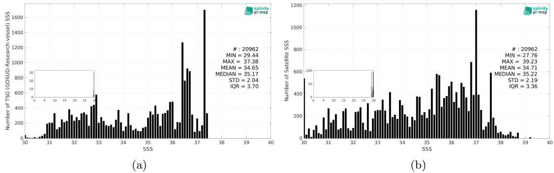
Figure 3: Histograms of SSS from TSG (GOSUD-Research-vessel) (a) and SMOS SSS L2Q v331 - With FLAG (CMEMS-CATDS-CPDC) (b) considering all match-up pairs per bins of 0.1 over the Gulf Stream Pi-MEP region and for the full satellite product period.
