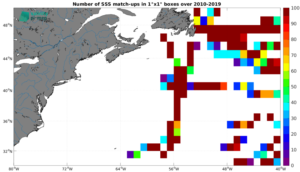
Figure 5: Number of SSS match-ups between TSG (GOSUD-Research-vessel) SSS and the SMOS SSS L2Q v331 - With FLAG (CMEMS-CATDS-CPDC) SSS product for the Gulf Stream Pi-MEP region over 1^{\circ} \times 1^{\circ} boxes and for the full satellite product period.
