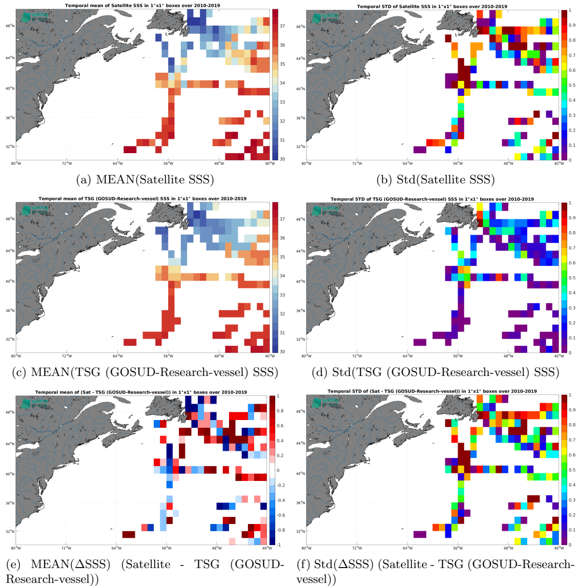
Figure 7: Temporal mean (left) and Std (right) of SSS from SMOS SSS L2Q v331 - With FLAG (CMEMS-CATDS-CPDC) (top), TSG (GOSUD-Research-vessel) (middle), and of \Delta SSS (Satellite - TSG (GOSUD-Research-vessel)). Only match-up pairs are used to generate these maps.
