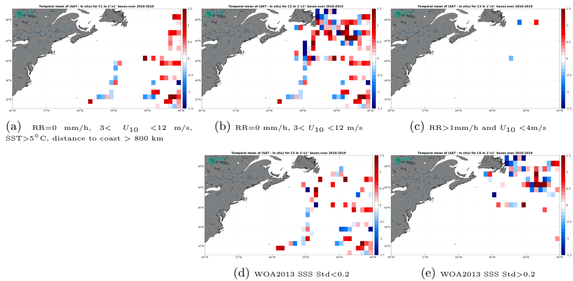
Figure 14: Temporal mean gridded over spatial boxes of size 1^\circ \times 1^\circ of \Delta SSS (SMOS SSS L2Q v331 - With FLAG (CMEMS-CATDS-CPDC) - TSG (GOSUD-Research-vessel)) for 5 different subdatasets corresponding to:RR=0 mm/h, 3 < U_{10} < 12 m/s, SST > 5°C, distance to coast > 800 km (a), RR=0 mm/h, 3 < U_{10} < 12 m/s (b), RR > 1mm/h and U_{10} < 4 m/s (c), WOA2013 SSS Std < 0.2 (d), WOA2013 SSS Std > 0.2 (e).
