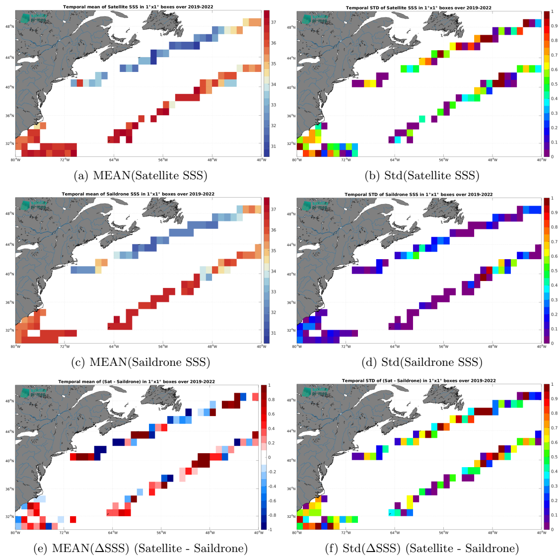
Figure 7: Temporal mean (left) and Std (right) of SSS from SMOS SSS L2Q v331 - With FLAG (CMEMS-CATDS-CPDC) (top), Saildrone (middle), and of \Delta SSS (Satellite - Saildrone). Only match-up pairs are used to generate these maps.
