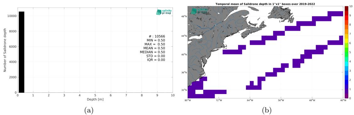
Figure 4: Histograms of the depth of the upper level SSS measurements from Sairdrone in the Match-up DataBase for the Gulf Stream Pi-MEP region (a) and temporal mean spatial distribution of pressure of the in situ SSS data over 1^\circ \times 1^\circ boxes and for the full satellite product period (b).
