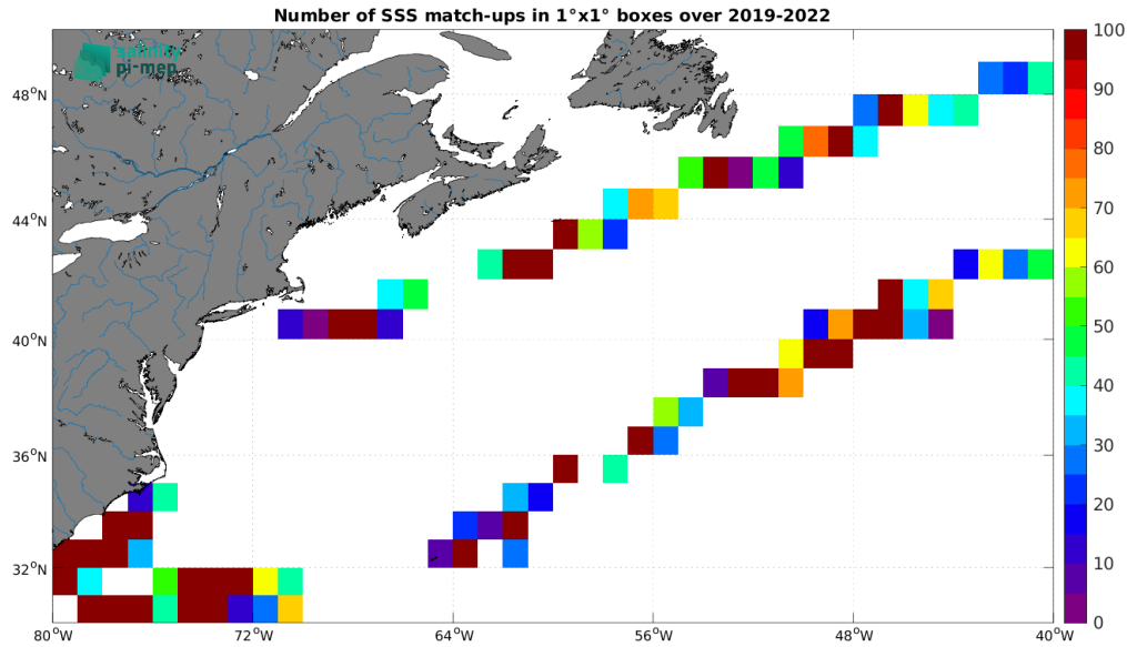
Figure 5: Number of SSS match-ups between Saildrone SSS and the SMOS SSS L2Q v331 - With FLAG (CMEMS-CATDS-CPDC) SSS product for the Gulf Stream Pi-MEP region over 1^\circ \times 1^\circ boxes and for the full satellite product period.
