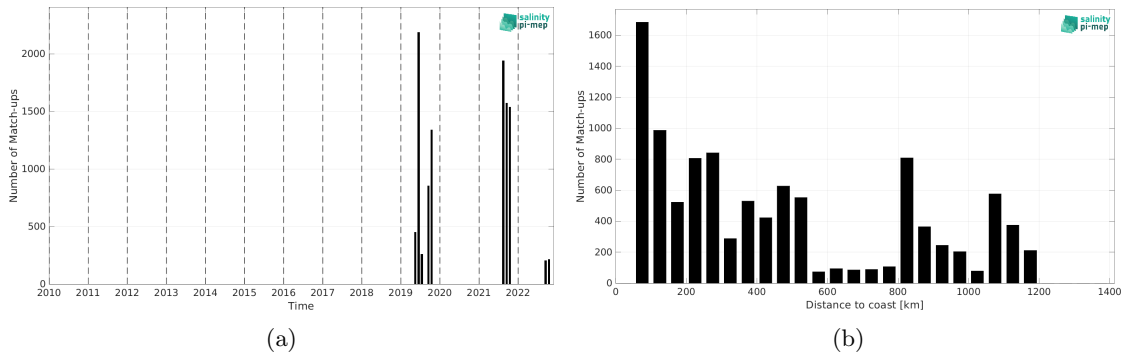
Figure 2: Number of match-ups between Saildrone and SMOS SSS L2Q v331 - With FLAG (CMEMS-CATDS-CPDC) SSS as a function of time (a) and as function of the distance to coast (b) over the Gulf Stream Pi-MEP region and for the full satellite product period.
