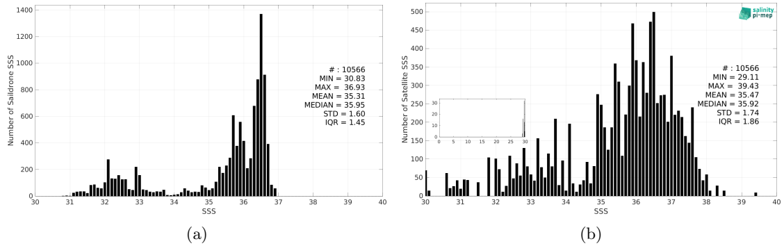
Figure 3: Histograms of SSS from Sairdrone (a) and SMOS SSS L2Q v331 - With FLAG (CMEMS-CATDS-CPDC) (b) considering all match-up pairs per bins of 0.1 over the Gulf Stream Pi-MEP region and for the full satellite product period.
