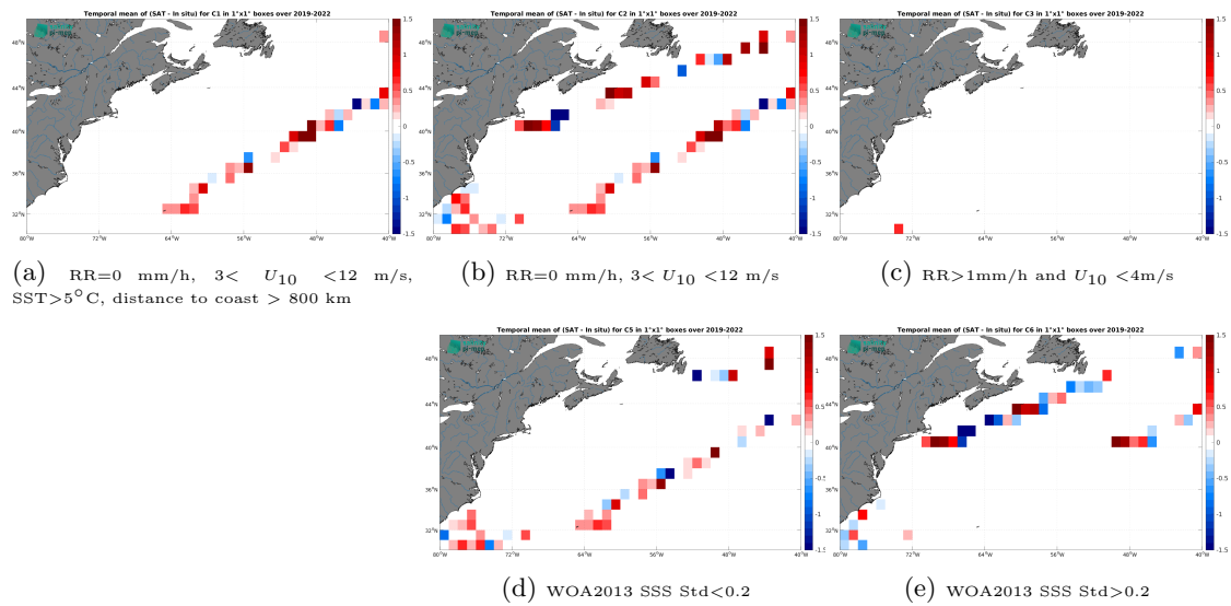
Figure 14: Temporal mean gridded over spatial boxes of size 1^\circ \times 1^\circ of \Delta SSS (SMOS SSS L2Q v331 - With FLAG (CMEMS-CATDS-CPDC) - Saildrone) for 5 different subdatasets corresponding to:RR=0 mm/h, 3 < U_{10} < 12 m/s, SST >5^\circ C, distance to coast > 800 km (a), RR=0 mm/h, 3 < U_{10} < 12 m/s (b), RR >1 mm/h and U_{10} < 4 m/s (c), WOA2013 SSS Std <0.2 (d), WOA2013 SSS Std >0.2 (e).
