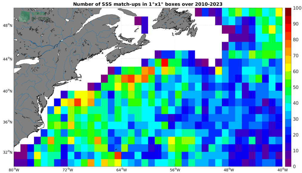
Figure 4: Number of SSS match-ups between Argo SSS and the SMOS SSS L2Q v331 - With FLAG (CMEMS-CATDS-CPDC) SSS product for the Gulf Stream Pi-MEP region over 1^\circ \times 1^\circ boxes and for the full satellite product period.
