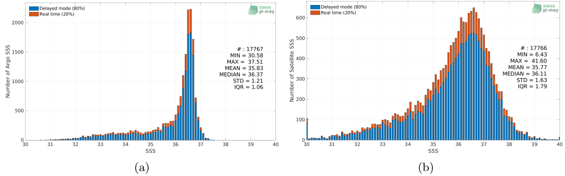
Figure 2: Histograms of SSS from Argo (a) and SMOS SSS L2Q v331 - With FLAG (CMEMS-CATDS-CPDC) (b) considering all match-up pairs per bins of 0.1 over the Gulf Stream Pi-MEP region and for the full satellite product period.
