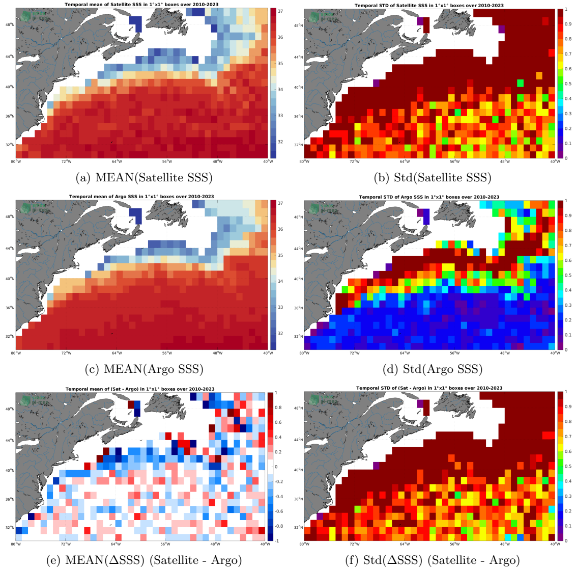
Figure 6: Temporal mean (left) and Std (right) of SSS from SMOS SSS L2Q v331 - With FLAG (CMEMS-CATDS-CPDC) (top), Argo (middle), and of \Delta SSS (Satellite - Argo). Only match-up pairs are used to generate these maps.
