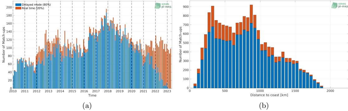
Figure 1: Number of match-ups between Argo and SMOS SSS L2Q v331 - With FLAG (CMEMS-CATDS-CPDC) SSS as a function of time (a) and as function of the distance to coast (b) over the Gulf Stream Pi-MEP region and for the full satellite product period.
