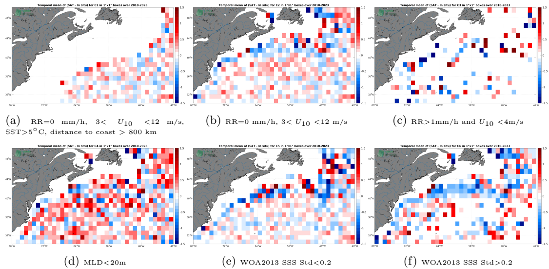
Figure 12: Temporal mean gridded over spatial boxes of size 1^\circ \times 1^\circ of \Delta SSS (SMOS SSS L2Q v331 - With FLAG (CMEMS-CATDS-CPDC) - Argo) for 6 different subdatasets corresponding to:RR=0 mm/h, 3 < U_{10} < 12 m/s, SST > 5^\circ\text{C} , distance to coast > 800 km (a), RR=0 mm/h, 3 < U_{10} < 12 m/s (b), RR > 1 mm/h and U_{10} < 4 m/s (c),MLD < 20 m (d),WOA2013 SSS Std < 0.2 (e),WOA2013 SSS Std > 0.2 (f).
