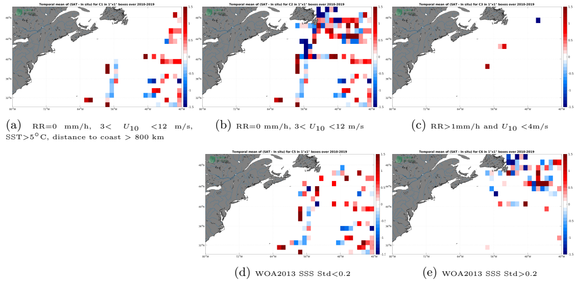
Figure 12: Temporal mean gridded over spatial boxes of size 1^\circ \times 1^\circ of \Delta SSS (SMOS SSS L2Q v331 - No FLAG (CMEMS-CATDS-CPDC) - TSG (GOSUD-Research-vessel)) for 5 different subdatasets corresponding to:RR=0 mm/h, 3 < U_{10} < 12 m/s, SST > 5^\circ\text{C} , distance to coast > 800 km (a), RR=0 mm/h, 3 < U_{10} < 12 m/s (b), RR > 1 mm/h and U_{10} < 4 m/s (c), WOA2013 SSS Std < 0.2 (d), WOA2013 SSS Std > 0.2 (e).
