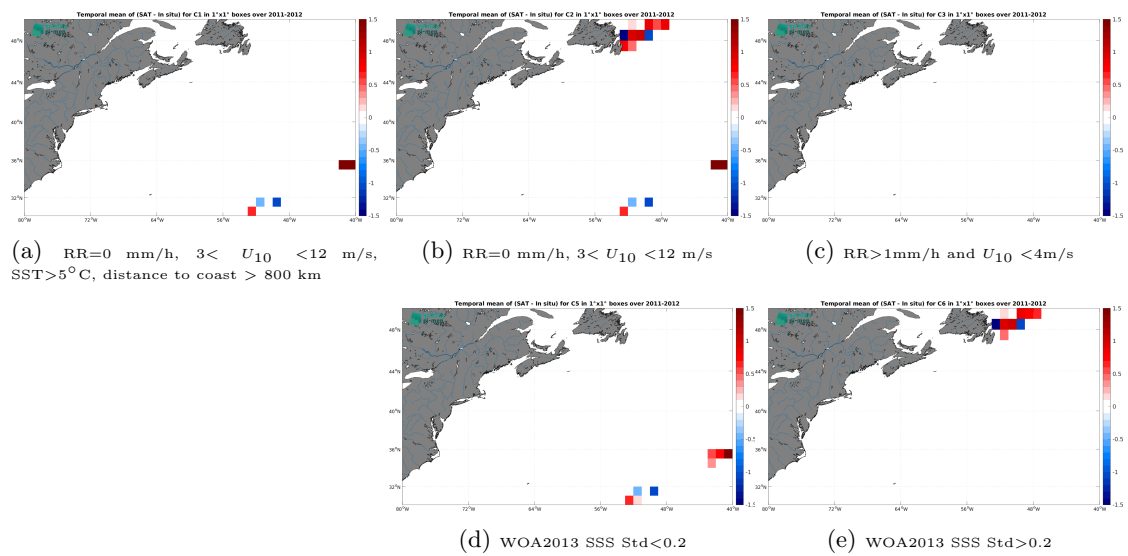
Figure 14: Temporal mean gridded over spatial boxes of size 1^\circ \times 1^\circ of \Delta SSS (SMOS SSS L2Q v331 - No FLAG (CMEMS-CATDS-CPDC) - TSG (CSIC-UTM)) for 5 different subdatasets corresponding to:RR=0 mm/h, 3 < U_{10} < 12 m/s, SST >5^\circ\text{C} , distance to coast > 800 km (a), RR=0 mm/h, 3 < U_{10} < 12 m/s (b), RR >1 mm/h and U_{10} < 4 m/s (c), WOA2013 SSS Std <0.2 (d), WOA2013 SSS Std >0.2 (e).
