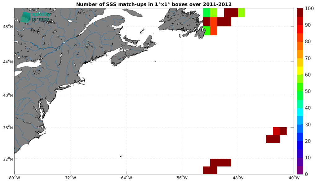
Figure 5: Number of SSS match-ups between TSG (CSIC-UTM) SSS and the SMOS SSS L2Q v331 - No FLAG (CMEMS-CATDS-CPDC) SSS product for the Gulf Stream Pi-MEP region over 1^\circ \times 1^\circ boxes and for the full satellite product period.
