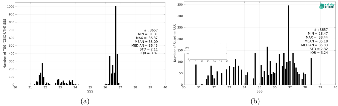
Figure 3: Histograms of SSS from TSG (CSIC-UTM) (a) and SMOS SSS L2Q v331 - No FLAG (CMEMS-CATDS-CPDC) (b) considering all match-up pairs per bins of 0.1 over the Gulf Stream Pi-MEP region and for the full satellite product period.
