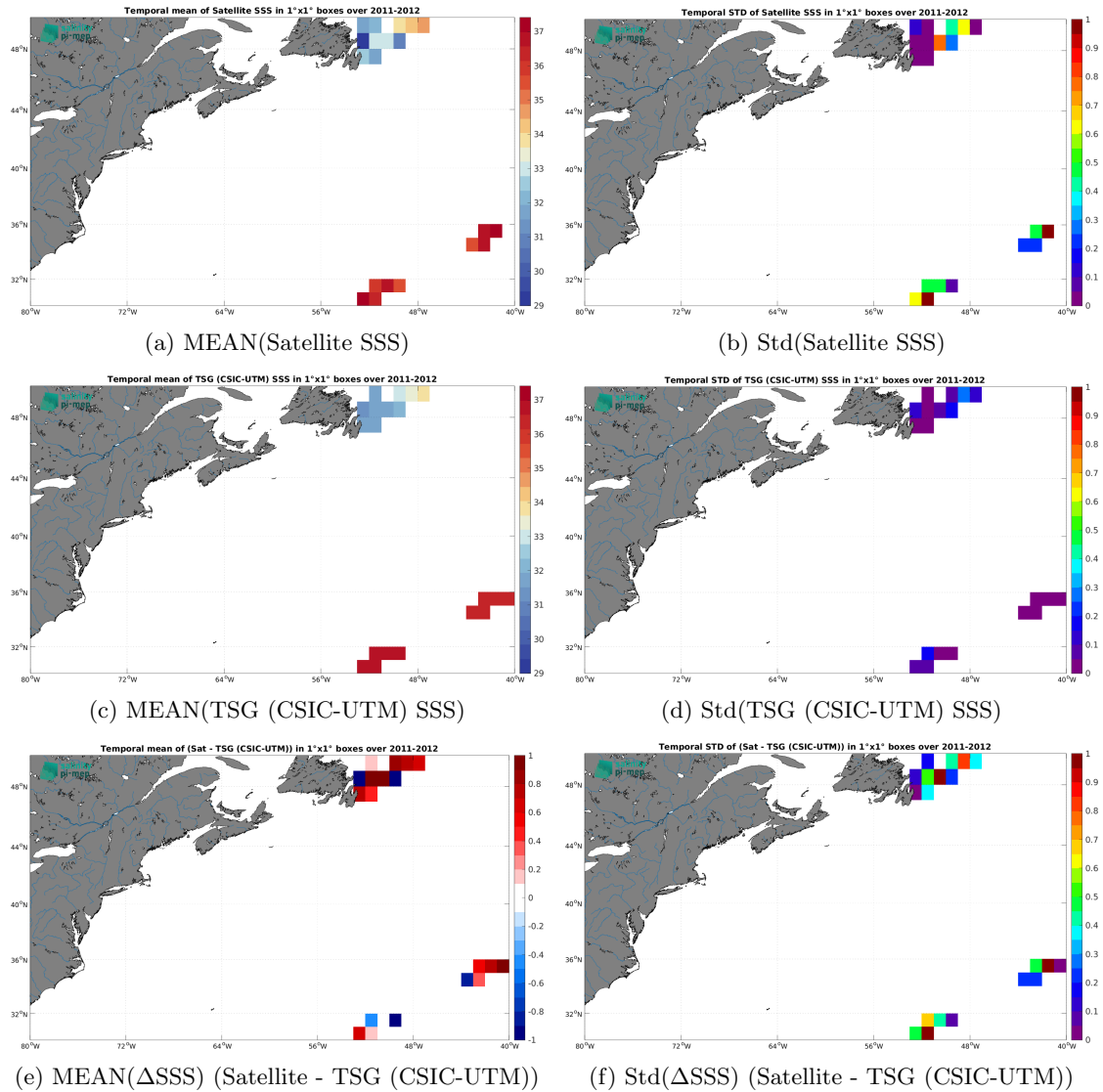
Figure 7: Temporal mean (left) and Std (right) of SSS from SMOS SSS L2Q v331 - No FLAG (CMEMS-CATDS-CPDC) (top), TSG (CSIC-UTM) (middle), and of \Delta SSS (Satellite - TSG (CSIC-UTM)). Only match-up pairs are used to generate these maps.
