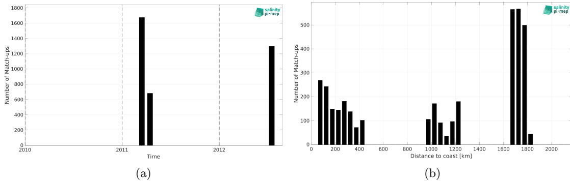
Figure 2: Number of match-ups between TSG (CSIC-UTM) and SMOS SSS L2Q v331 - No FLAG (CMEMS-CATDS-CPDC) SSS as a function of time (a) and as function of the distance to coast (b) over the Gulf Stream Pi-MEP region and for the full satellite product period.
