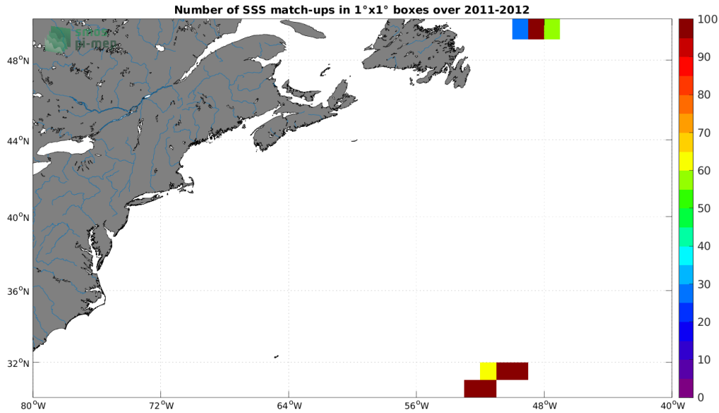
Figure 4: Number of SSS match-ups between TSG (CSIC-UTM) SSS and the SMOS SSS L2Q v331 - No FLAG (CMEMS-CATDS-CPDC) SSS product for the Gulf Stream Pi-MEP region over 1^\circ \times 1^\circ boxes and for the full satellite product period.
