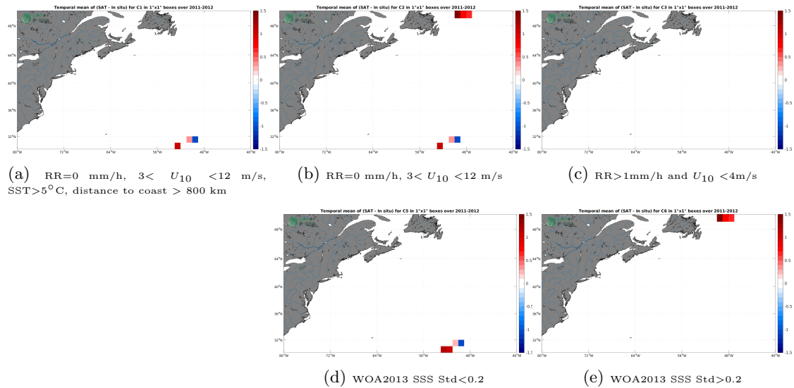
Figure 12: Temporal mean gridded over spatial boxes of size 1^{\circ}\times 1^{\circ} of \Delta\text{SSS} (SMOS SSS L2Q v331 - No FLAG (CMEMS-CATDS-CPDC) - TSG (CSIC-UTM)) for 5 different subdatasets corresponding to:RR=0 mm/h, 3 < U_{10} < 12 m/s, SST >5^{\circ}\text{C} , distance to coast > 800 km (a), RR=0 mm/h, 3 < U_{10} < 12 m/s (b), RR >1 mm/h and U_{10} < 4 m/s (c), WOA2013 SSS Std <0.2 (d), WOA2013 SSS Std >0.2 (e).
