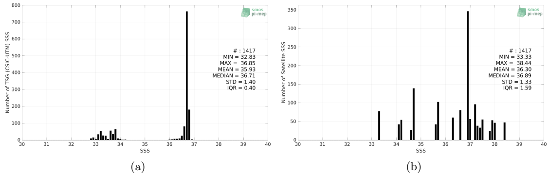
Figure 2: Histograms of SSS from TSG (CSIC-UTM) (a) and SMOS SSS L2Q v331 - No FLAG (CMEMS-CATDS-CPDC) (b) considering all match-up pairs per bins of 0.1 over the Gulf Stream Pi-MEP region and for the full satellite product period.
