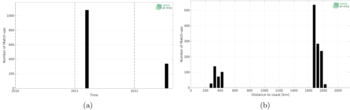
Figure 1: Number of match-ups between TSG (CSIC-UTM) and SMOS SSS L2Q v331 - No FLAG (CMEMS-CATDS-CPDC) SSS as a function of time (a) and as function of the distance to coast (b) over the Gulf Stream Pi-MEP region and for the full satellite product period.
