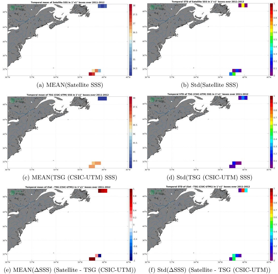
Figure 6: Temporal mean (left) and Std (right) of SSS from SMOS SSS L2Q v331 - No FLAG (CMEMS-CATDS-CPDC) (top), TSG (CSIC-UTM) (middle), and of \Delta SSS (Satellite - TSG (CSIC-UTM)). Only match-up pairs are used to generate these maps.
