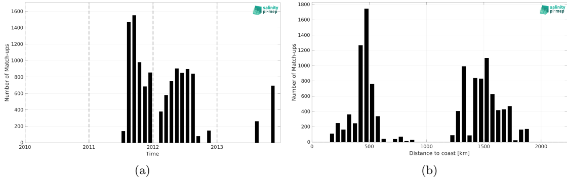
Figure 2: Number of match-ups between Surface drifters and SMOS SSS L2Q v331 - No FLAG (CMEMS-CATDS-CPDC) SSS as a function of time (a) and as function of the distance to coast (b) over the Gulf Stream Pi-MEP region and for the full satellite product period.
