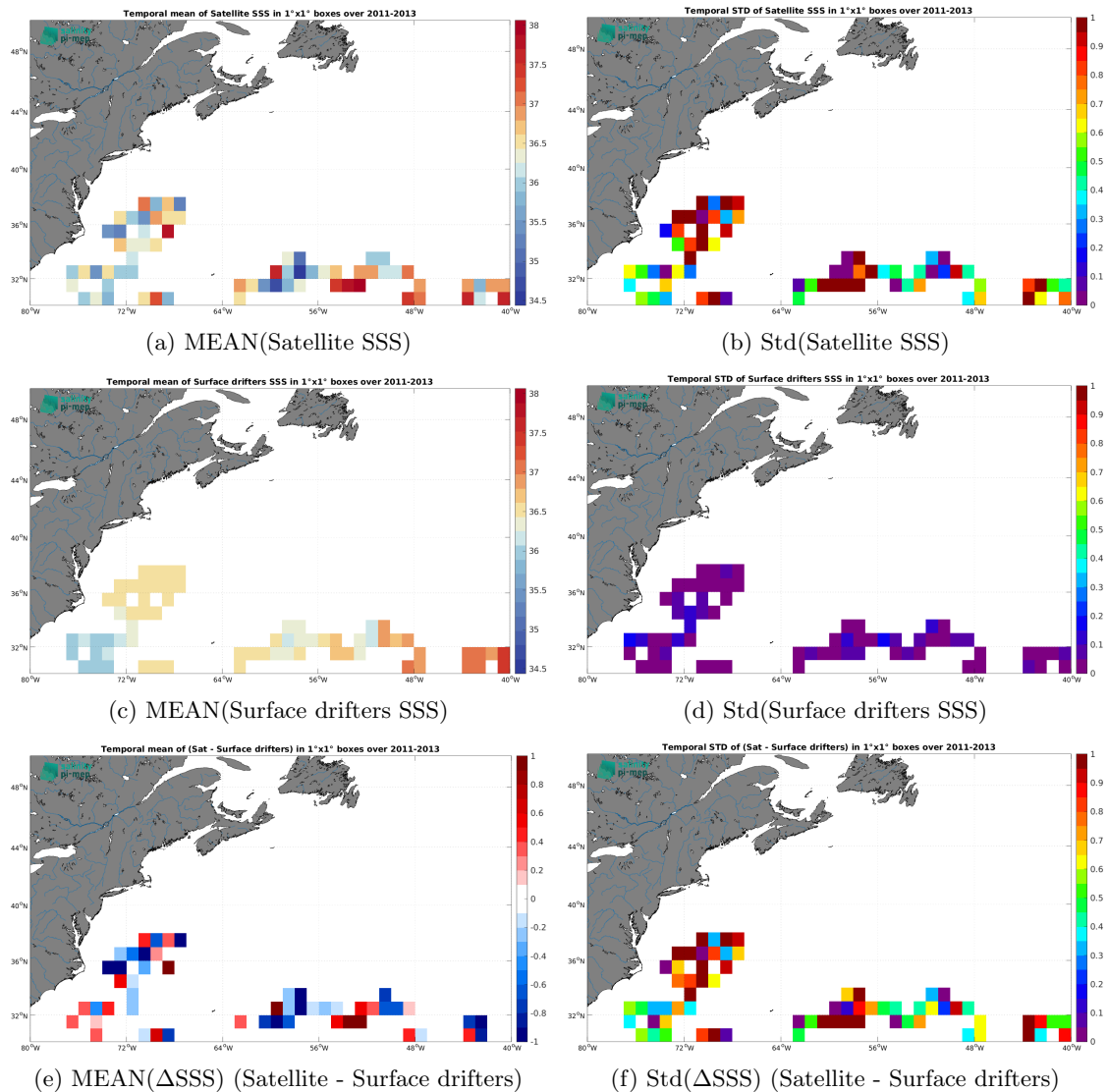
Figure 6: Temporal mean (left) and Std (right) of SSS from SMOS SSS L2Q v331 - No FLAG (CMEMS-CATDS-CPDC) (top), Surface drifters (middle), and of \Delta SSS (Satellite - Surface drifters). Only match-up pairs are used to generate these maps.
