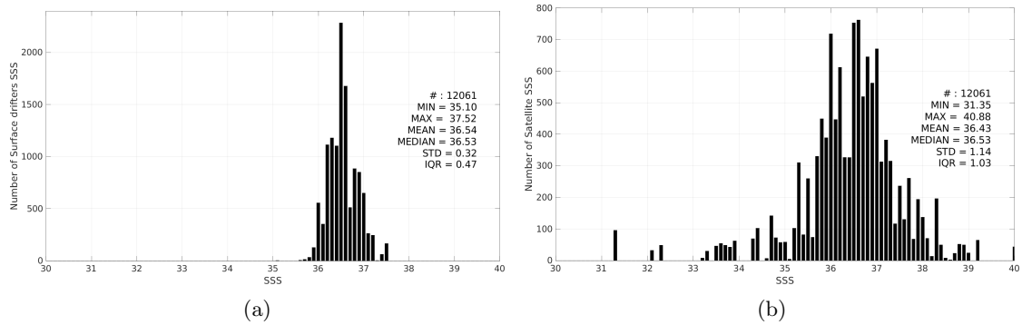
Figure 3: Histograms of SSS from Surface drifters (a) and SMOS SSS L2Q v331 - No FLAG (CMEMS-CATDS-CPDC) (b) considering all match-up pairs per bins of 0.1 over the Gulf Stream Pi-MEP region and for the full satellite product period.
