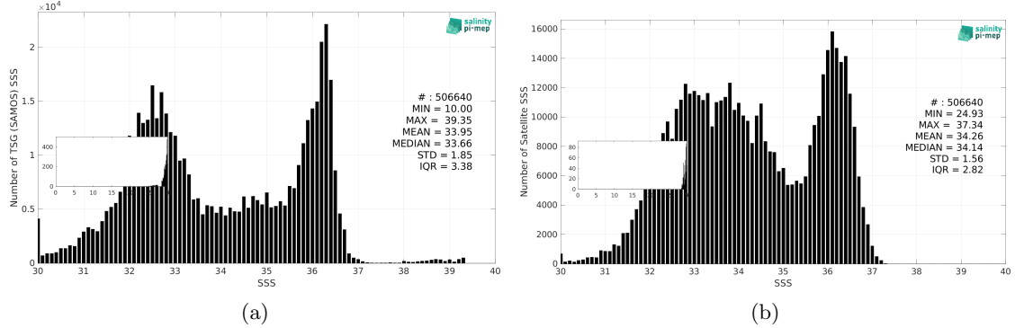
Figure 2: Histograms of SSS from TSG (SAMOS) (a) and SMOS SSS L3 v9 - 9 Days (CATDS-CEC-LOCEAN) (b) considering all match-up pairs per bins of 0.1 over the Gulf Stream Pi-MEP region and for the full satellite product period.
