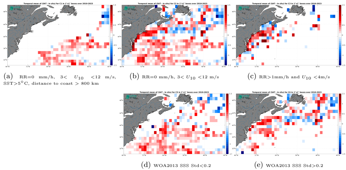
Figure 12: Temporal mean gridded over spatial boxes of size 1^\circ \times 1^\circ of \Delta SSS (SMOS SSS L3 v9 - 9 Days (CATDS-CEC-LOCEAN) - TSG (SAMOS)) for 5 different subdatasets corresponding to:RR=0 mm/h, 3 < U_{10} < 12 m/s, SST >5^\circ C, distance to coast > 800 km (a), RR=0 mm/h, 3 < U_{10} < 12 m/s (b), RR >1 mm/h and U_{10} < 4 m/s (c), WOA2013 SSS Std <0.2 (d), WOA2013 SSS Std >0.2 (e).
