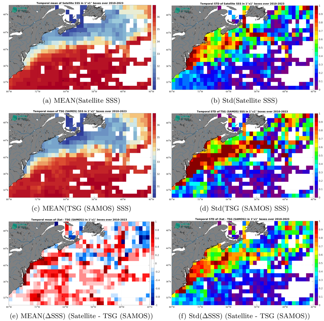
Figure 6: Temporal mean (left) and Std (right) of SSS from SMOS SSS L3 v9 - 9 Days (CATDS-CEC-LOCEAN) (top), TSG (SAMOS) (middle), and of \Delta SSS (Satellite - TSG (SAMOS)). Only match-up pairs are used to generate these maps.
