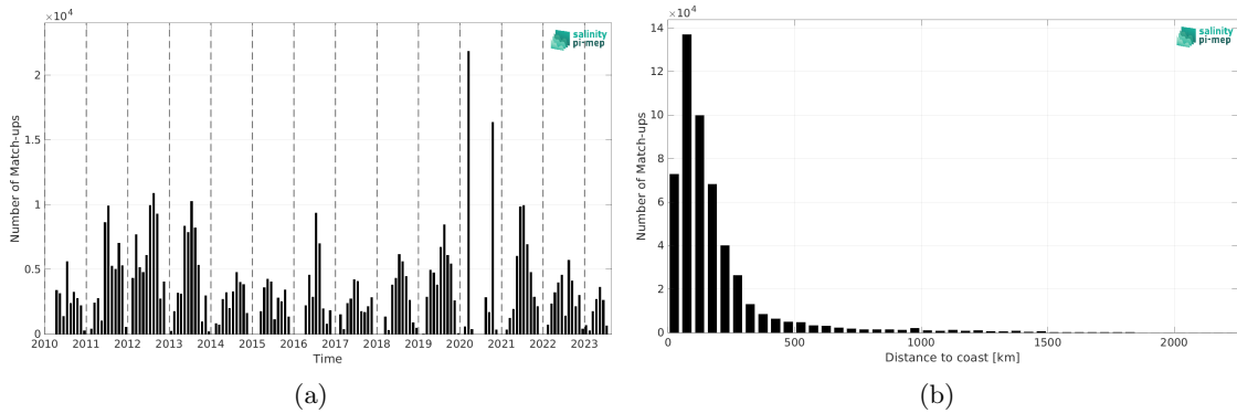
Figure 1: Number of match-ups between TSG (SAMOS) and SMOS SSS L3 v9 - 9 Days (CATDS-CEC-LOCEAN) SSS as a function of time (a) and as function of the distance to coast (b) over the Gulf Stream Pi-MEP region and for the full satellite product period.
