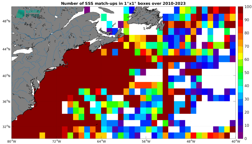
Figure 4: Number of SSS match-ups between TSG (SAMOS) SSS and the SMOS SSS L3 v9 - 9 Days (CATDS-CEC-LOCEAN) SSS product for the Gulf Stream Pi-MEP region over 1^\circ \times 1^\circ boxes and for the full satellite product period.
