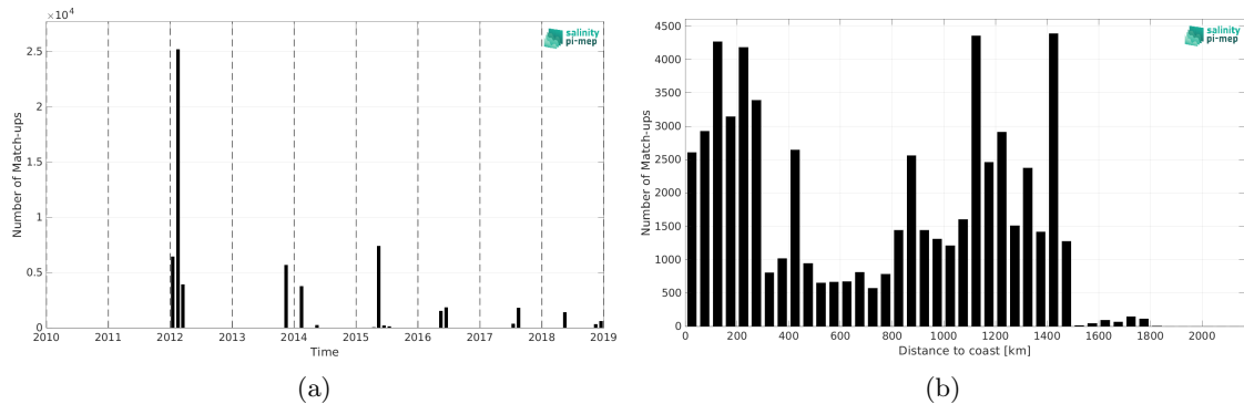
Figure 2: Number of match-ups between TSG (GOSUD-Sailing-ship) and SMOS SSS L3 v9 - 9 Days (CATDS-CEC-LOCEAN) SSS as a function of time (a) and as function of the distance to coast (b) over the Gulf Stream Pi-MEP region and for the full satellite product period.
