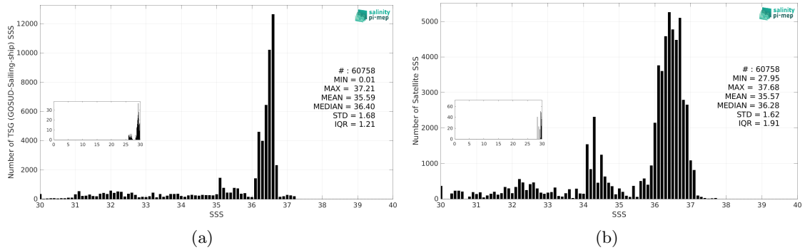
Figure 3: Histograms of SSS from TSG (GOSUD-Sailing-ship) (a) and SMOS SSS L3 v9 - 9 Days (CATDS-CEC-LOCEAN) (b) considering all match-up pairs per bins of 0.1 over the Gulf Stream Pi-MEP region and for the full satellite product period.
