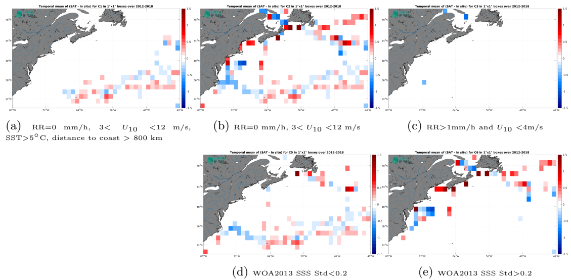
Figure 14: Temporal mean gridded over spatial boxes of size 1^\circ \times 1^\circ of \Delta SSS (SMOS SSS L3 v9 - 9 Days (CATDS-CEC-LOCEAN) - TSG (GOSUD-Sailing-ship)) for 5 different subdatasets corresponding to: RR=0 mm/h, 3 < U_{10} < 12 m/s, SST>5°C, distance to coast > 800 km (a), RR=0 mm/h, 3 < U_{10} < 12 m/s (b), RR>1mm/h and U_{10} < 4 m/s (c), WOA2013 SSS Std<0.2 (d), WOA2013 SSS Std>0.2 (e).
