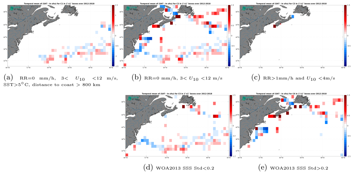
Figure 12: Temporal mean gridded over spatial boxes of size 1^{\circ}\times 1^{\circ} of \Delta SSS (SMOS SSS L3 v9 - 9 Days (CATDS-CEC-LOCEAN) - TSG (GOSUD-Sailing-ship)) for 5 different subdatasets corresponding to:RR=0 mm/h, 3 < U_{10} < 12 m/s, SST > 5^{\circ}\text{C} , distance to coast > 800 km (a), RR=0 mm/h, 3 < U_{10} < 12 m/s (b), RR > 1 mm/h and U_{10} < 4 m/s (c), WOA2013 SSS Std < 0.2 (d), WOA2013 SSS Std > 0.2 (e).
