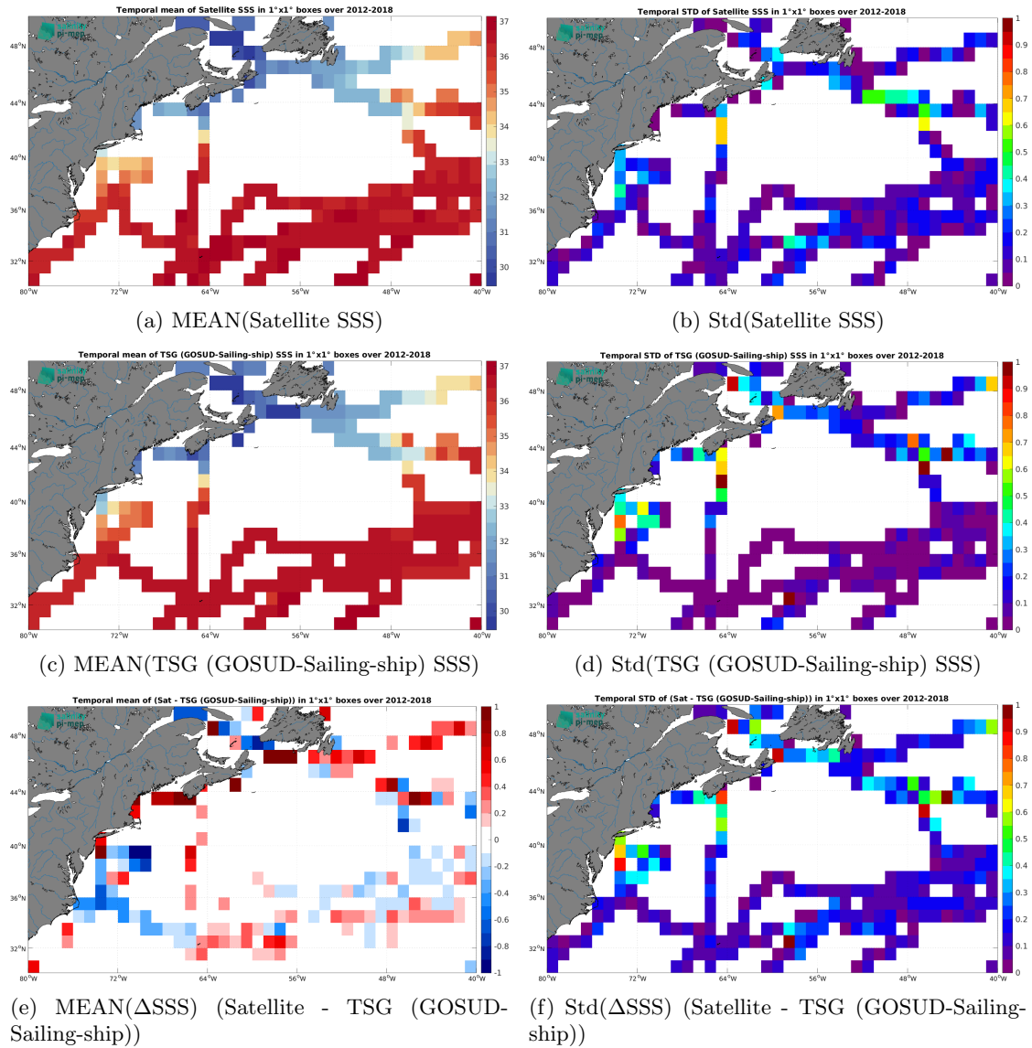
Figure 6: Temporal mean (left) and Std (right) of SSS from SMOS SSS L3 v9 - 9 Days (CATDS-CEC-LOCEAN) (top), TSG (GOSUD-Sailing-ship) (middle), and of \Delta SSS (Satellite - TSG (GOSUD-Sailing-ship)). Only match-up pairs are used to generate these maps.
