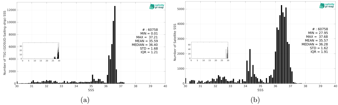
Figure 2: Histograms of SSS from TSG (GOSUD-Sailing-ship) (a) and SMOS SSS L3 v9 - 9 Days (CATDS-CEC-LOCEAN) (b) considering all match-up pairs per bins of 0.1 over the Gulf Stream Pi-MEP region and for the full satellite product period.
