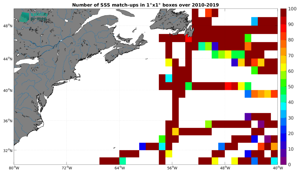
Figure 4: Number of SSS match-ups between TSG (GOSUD-Research-vessel) SSS and the SMOS SSS L3 v9 - 9 Days (CATDS-CEC-LOCEAN) SSS product for the Gulf Stream Pi-MEP region over 1^\circ \times 1^\circ boxes and for the full satellite product period.
