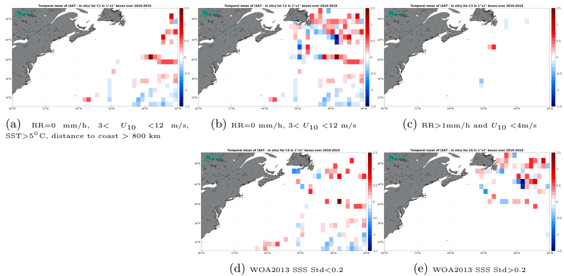
Figure 12: Temporal mean gridded over spatial boxes of size 1^{\circ}\times 1^{\circ} of \Delta SSS (SMOS SSS L3 v9 - 9 Days (CATDS-CEC-LOCEAN) - TSG (GOSUD-Research-vessel)) for 5 different subdatasets corresponding to:RR=0 mm/h, 3 < U_{10} < 12 m/s, SST > 5^{\circ}\text{C} , distance to coast > 800 km (a), RR=0 mm/h, 3 < U_{10} < 12 m/s (b), RR > 1 mm/h and U_{10} < 4 m/s (c), WOA2013 SSS Std < 0.2 (d), WOA2013 SSS Std > 0.2 (e).
