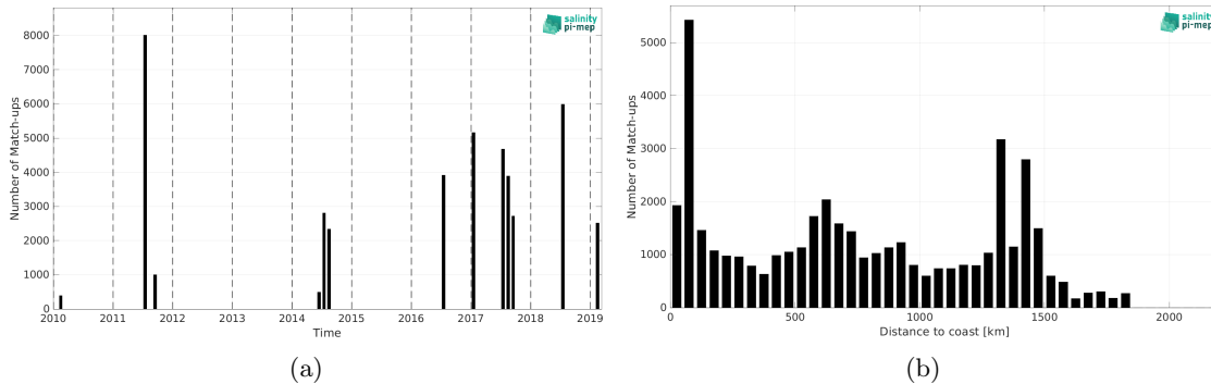
Figure 1: Number of match-ups between TSG (GOSUD-Research-vessel) and SMOS SSS L3 v9 - 9 Days (CATDS-CEC-LOCEAN) SSS as a function of time (a) and as function of the distance to coast (b) over the Gulf Stream Pi-MEP region and for the full satellite product period.
