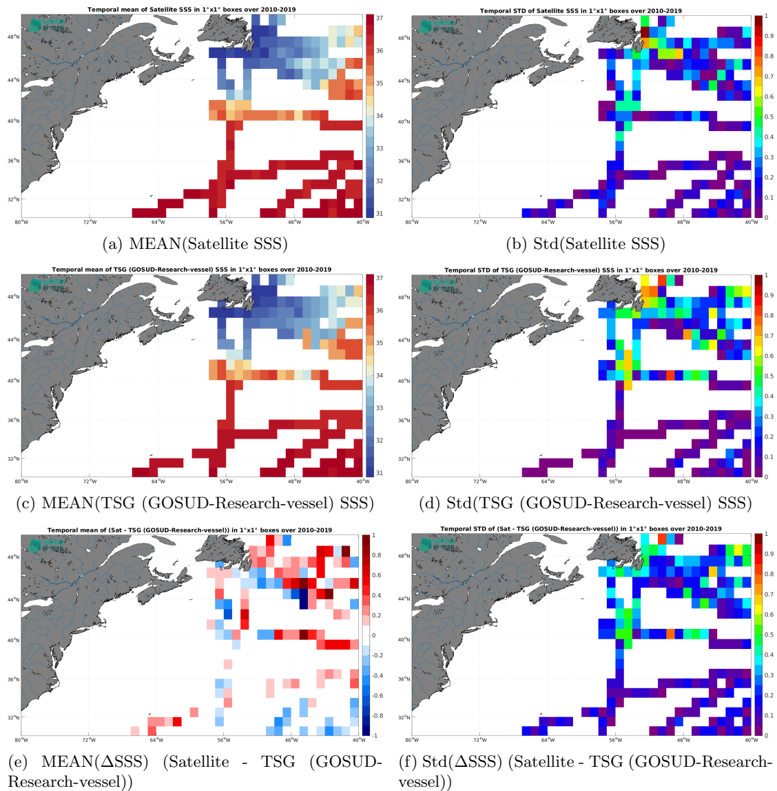
Figure 6: Temporal mean (left) and Std (right) of SSS from SMOS SSS L3 v9 - 9 Days (CATDS-CEC-LOCEAN) (top), TSG (GOSUD-Research-vessel) (middle), and of \Delta SSS (Satellite - TSG (GOSUD-Research-vessel)). Only match-up pairs are used to generate these maps.
