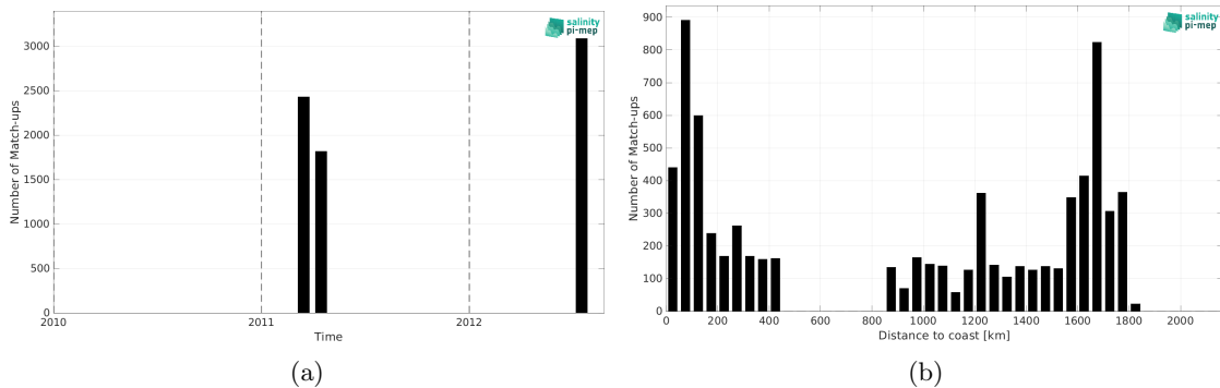
Figure 2: Number of match-ups between TSG (CSIC-UTM) and SMOS SSS L3 v9 - 9 Days (CATDS-CEC-LOCEAN) SSS as a function of time (a) and as function of the distance to coast (b) over the Gulf Stream Pi-MEP region and for the full satellite product period.
