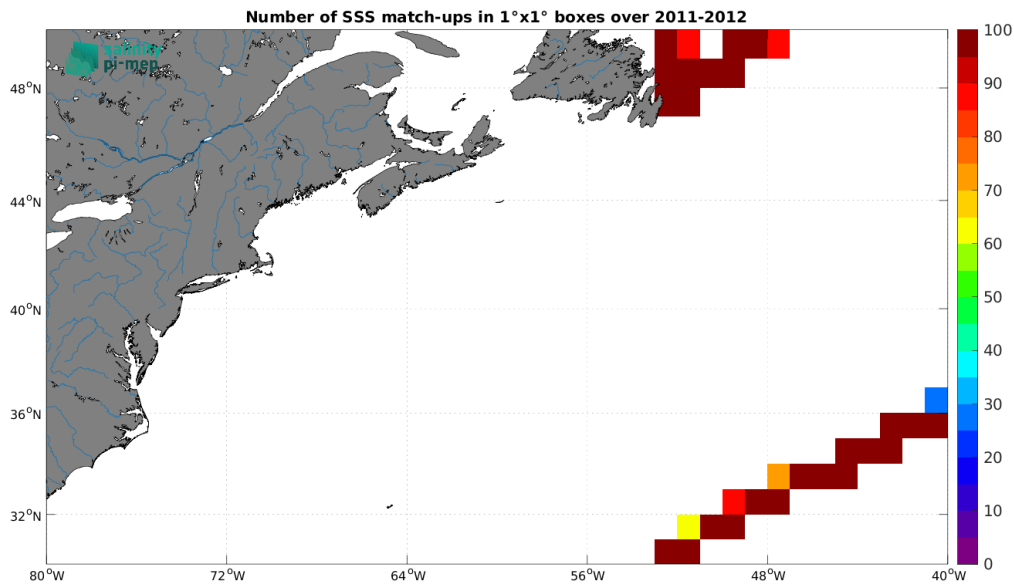
Figure 5: Number of SSS match-ups between TSG (CSIC-UTM) SSS and the SMOS SSS L3 v9 - 9 Days (CATDS-CEC-LOCEAN) SSS product for the Gulf Stream Pi-MEP region over 1^\circ \times 1^\circ boxes and for the full satellite product period.
