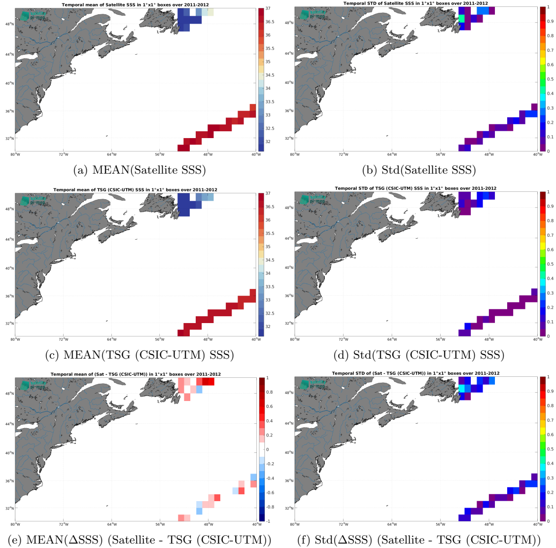
Figure 7: Temporal mean (left) and Std (right) of SSS from SMOS SSS L3 v9 - 9 Days (CATDS-CEC-LOCEAN) (top), TSG (CSIC-UTM) (middle), and of \Delta SSS (Satellite - TSG (CSIC-UTM)). Only match-up pairs are used to generate these maps.
