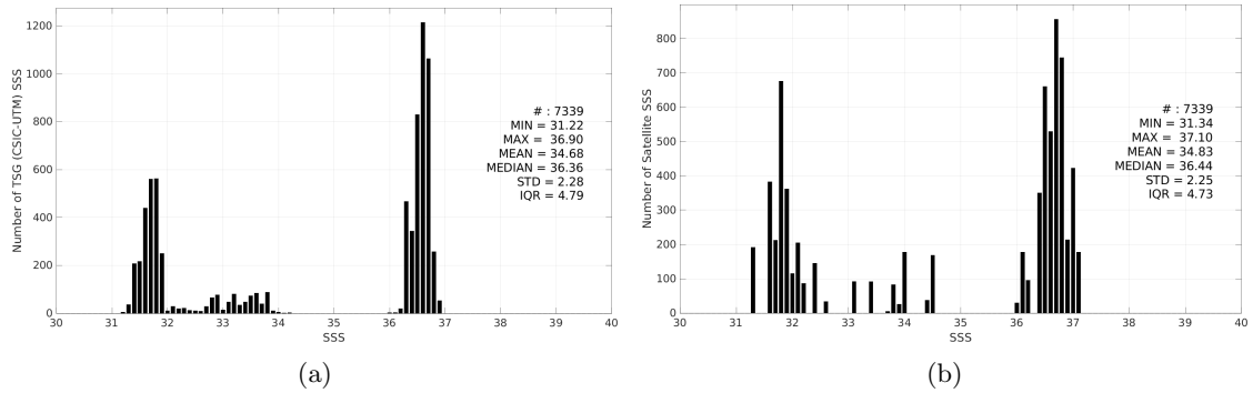
Figure 3: Histograms of SSS from TSG (CSIC-UTM) (a) and SMOS SSS L3 v9 - 9 Days (CATDS-CEC-LOCEAN) (b) considering all match-up pairs per bins of 0.1 over the Gulf Stream Pi-MEP region and for the full satellite product period.
