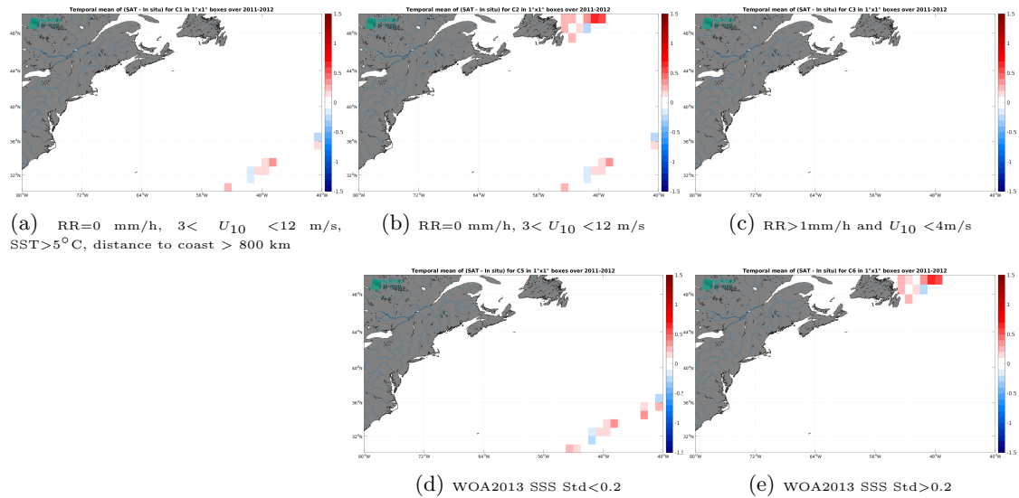
Figure 12: Temporal mean gridded over spatial boxes of size 1^{\circ}\times 1^{\circ} of \Delta\text{SSS} (SMOS SSS L3 v9 - 9 Days (CATDS-CEC-LOCEAN) - TSG (CSIC-UTM)) for 5 different subdatasets corresponding to:RR=0 mm/h, 3 < U_{10} < 12 m/s, SST >5^{\circ}\text{C} , distance to coast > 800 km (a), RR=0 mm/h, 3 < U_{10} < 12 m/s (b), RR >1 mm/h and U_{10} < 4 m/s (c), WOA2013 SSS Std <0.2 (d), WOA2013 SSS Std >0.2 (e).
