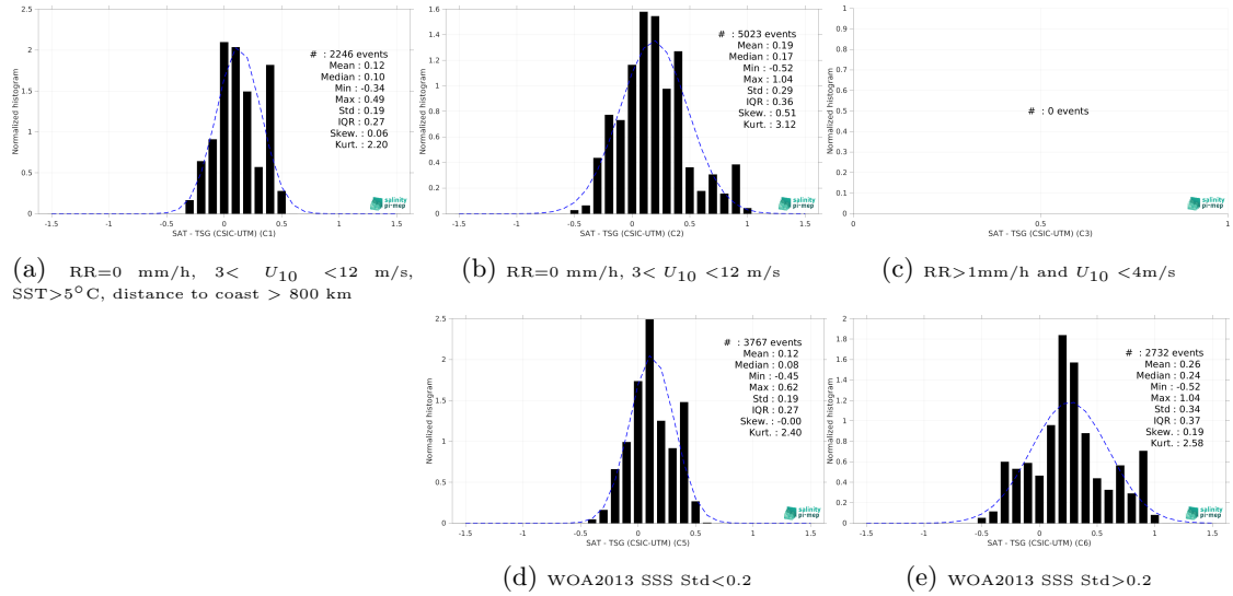
Figure 13: Normalized histogram of \Delta SSS (SMOS SSS L3 v9 - 9 Days (CATDS-CEC-LOCEAN) - TSG (CSIC-UTM)) for 5 different subdatasets corresponding to: RR=0 mm/h, 3 < U_{10} < 12 m/s, SST > 5°C, distance to coast > 800 km (a), RR=0 mm/h, 3 < U_{10} < 12 m/s (b), RR > 1mm/h and U_{10} < 4 m/s (c), WOA2013 SSS Std < 0.2 (d), WOA2013 SSS Std > 0.2 (e).
