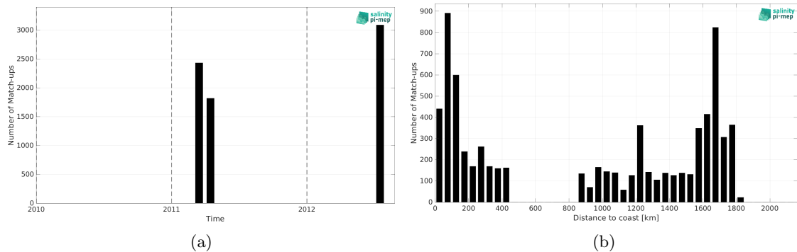
Figure 1: Number of match-ups between TSG (CSIC-UTM) and SMOS SSS L3 v9 - 9 Days (CATDS-CEC-LOCEAN) SSS as a function of time (a) and as function of the distance to coast (b) over the Gulf Stream Pi-MEP region and for the full satellite product period.
