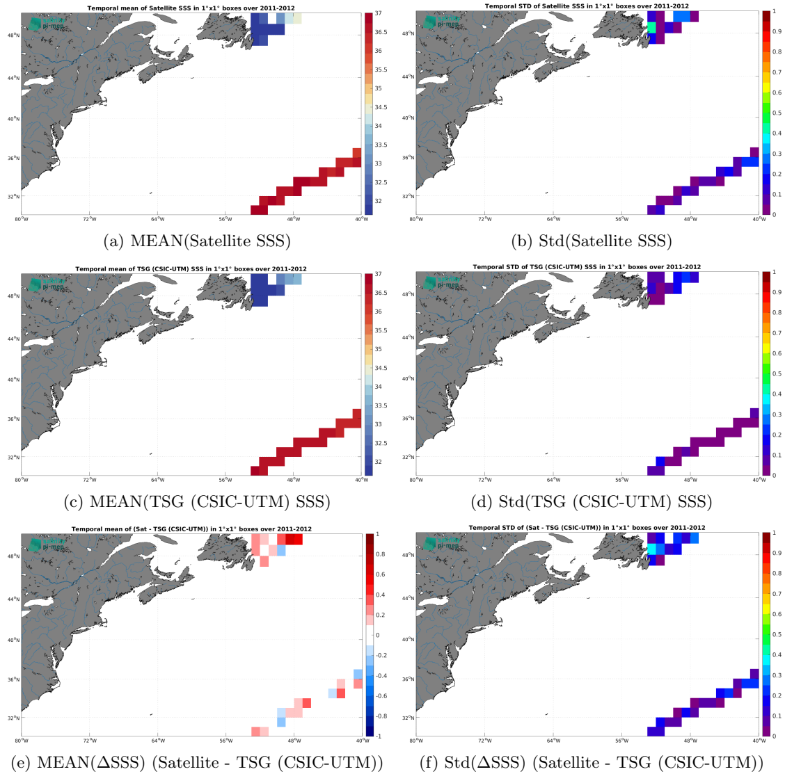
Figure 6: Temporal mean (left) and Std (right) of SSS from SMOS SSS L3 v9 - 9 Days (CATDS-CEC-LOCEAN) (top), TSG (CSIC-UTM) (middle), and of \Delta SSS (Satellite - TSG (CSIC-UTM)). Only match-up pairs are used to generate these maps.
