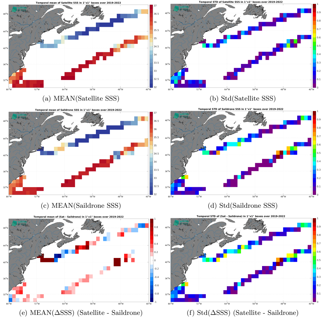
Figure 6: Temporal mean (left) and Std (right) of SSS from SMOS SSS L3 v9 - 9 Days (CATDS-CEC-LOCEAN) (top), Saildrone (middle), and of \Delta SSS (Satellite - Saildrone). Only match-up pairs are used to generate these maps.
