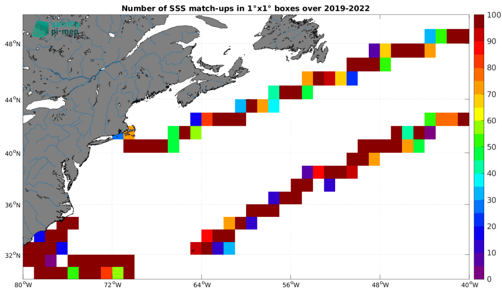
Figure 4: Number of SSS match-ups between Saildrone SSS and the SMOS SSS L3 v9 - 9 Days (CATDS-CEC-LOCEAN) SSS product for the Gulf Stream Pi-MEP region over 1^{\circ} \times 1^{\circ} boxes and for the full satellite product period.
