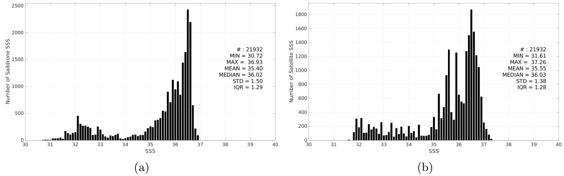
Figure 2: Histograms of SSS from Sairdrone (a) and SMOS SSS L3 v9 - 9 Days (CATDS-CEC-LOCEAN) (b) considering all match-up pairs per bins of 0.1 over the Gulf Stream Pi-MEP region and for the full satellite product period.
