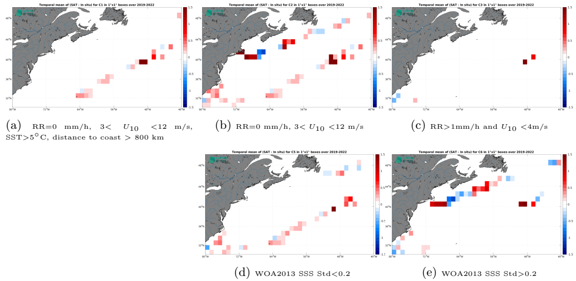
Figure 12: Temporal mean gridded over spatial boxes of size 1^\circ \times 1^\circ of \Delta SSS (SMOS SSS L3 v9 - 9 Days (CATDS-CEC-LOCEAN) - Saildrone) for 5 different subdatasets corresponding to:RR=0 mm/h, 3 < U_{10} < 12 m/s, SST >5^\circ C, distance to coast > 800 km (a), RR=0 mm/h, 3 < U_{10} < 12 m/s (b), RR >1 mm/h and U_{10} < 4 m/s (c), WOA2013 SSS Std <0.2 (d), WOA2013 SSS Std >0.2 (e).
