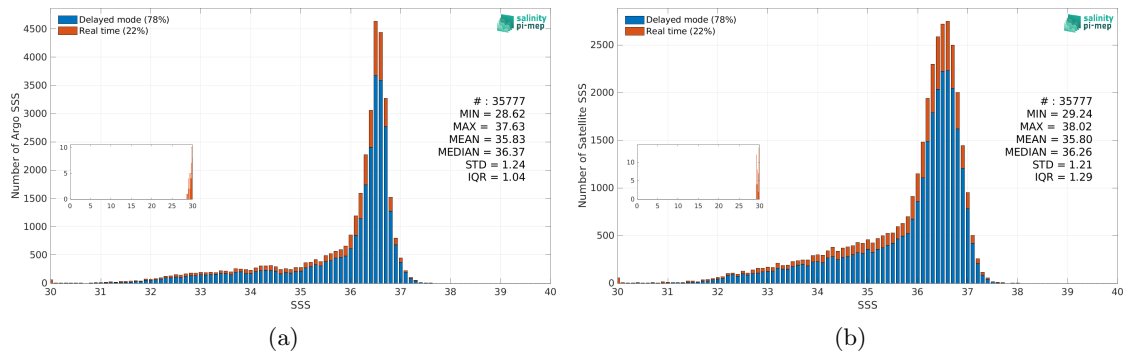
Figure 2: Histograms of SSS from Argo (a) and SMOS SSS L3 v9 - 9 Days (CATDS-CEC-LOCEAN) (b) considering all match-up pairs per bins of 0.1 over the Gulf Stream Pi-MEP region and for the full satellite product period.
