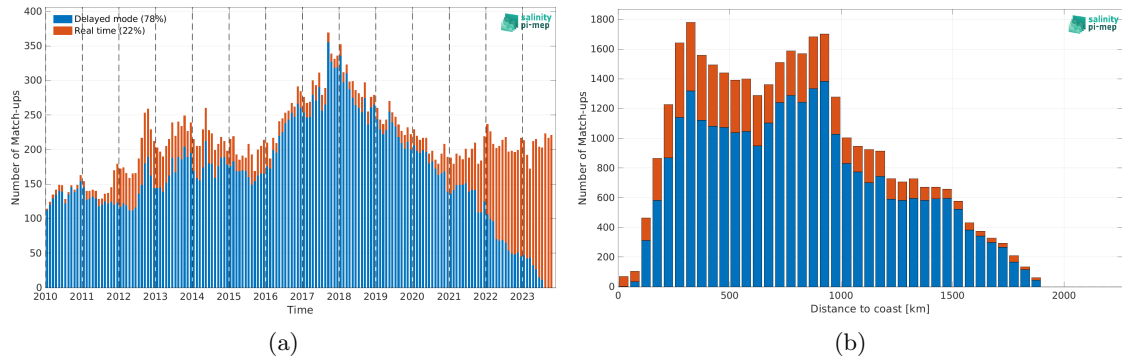
Figure 1: Number of match-ups between Argo and SMOS SSS L3 v9 - 9 Days (CATDS-CEC-LOCEAN) SSS as a function of time (a) and as function of the distance to coast (b) over the Gulf Stream Pi-MEP region and for the full satellite product period.
