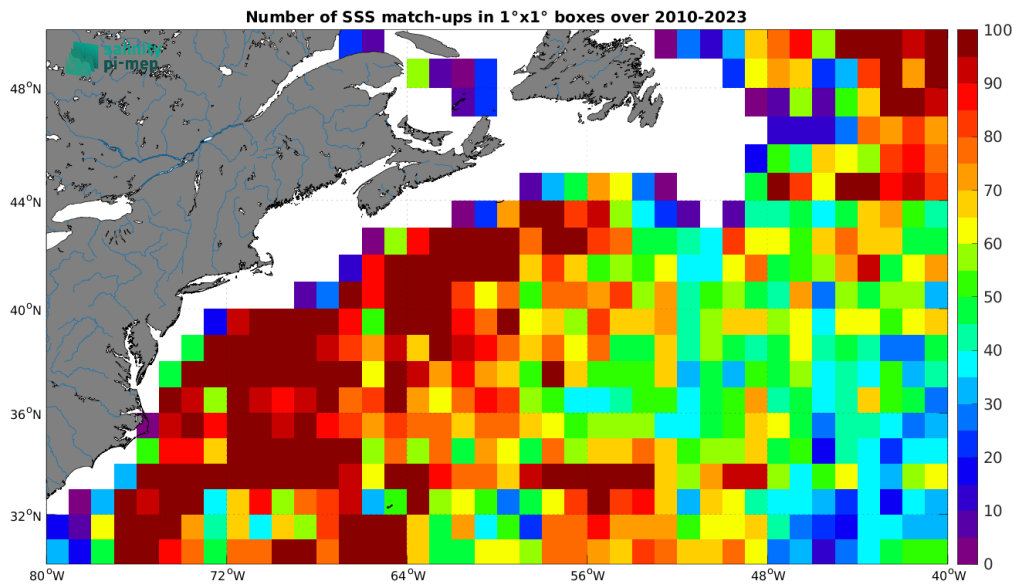
Figure 4: Number of SSS match-ups between Argo SSS and the SMOS SSS L3 v9 - 9 Days (CATDS-CEC-LOCEAN) SSS product for the Gulf Stream Pi-MEP region over 1^\circ \times 1^\circ boxes and for the full satellite product period.
