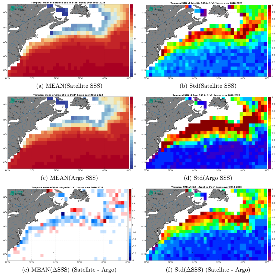
Figure 6: Temporal mean (left) and Std (right) of SSS from SMOS SSS L3 v9 - 9 Days (CATDS-CEC-LOCEAN) (top), Argo (middle), and of \Delta SSS (Satellite - Argo). Only match-up pairs are used to generate these maps.
