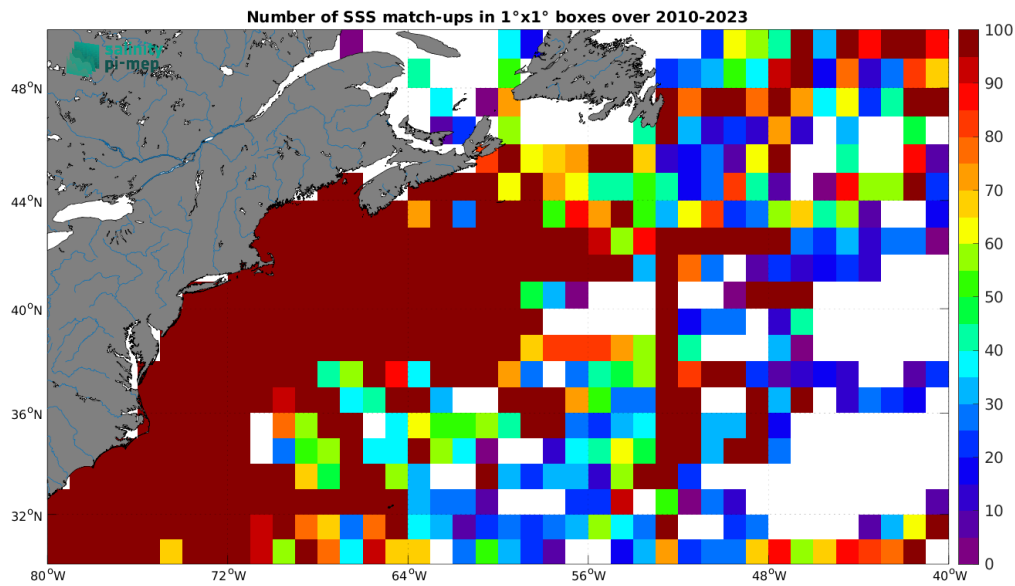
Figure 5: Number of SSS match-ups between TSG (SAMOS) SSS and the SMOS SSS L3 v9 - 18 Days (CATDS-CEC-LOCEAN) SSS product for the Gulf Stream Pi-MEP region over 1^\circ \times 1^\circ boxes and for the full satellite product period.
