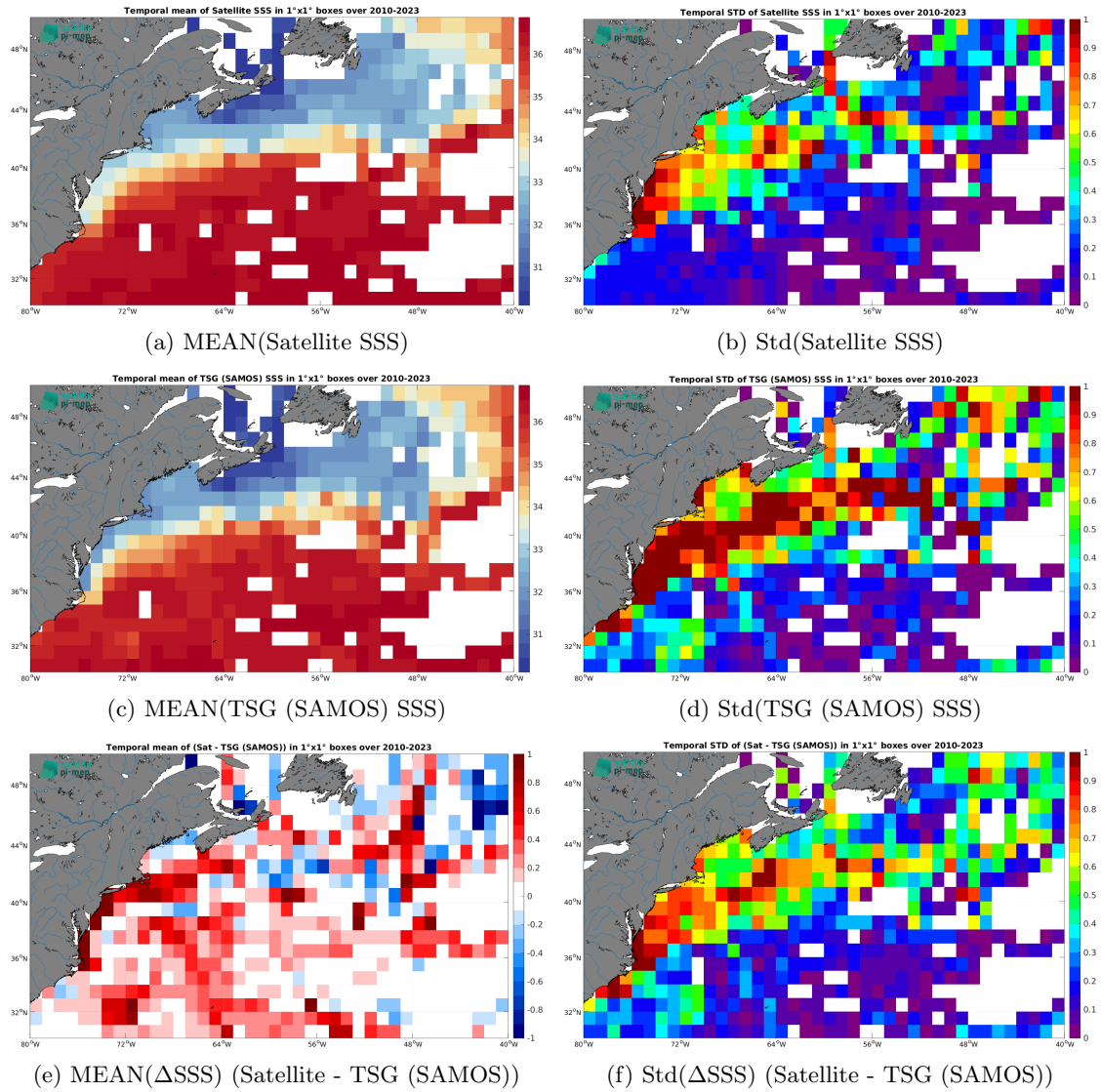
Figure 7: Temporal mean (left) and Std (right) of SSS from SMOS SSS L3 v9 - 18 Days (CATDS-CEC-LOCEAN) (top), TSG (SAMOS) (middle), and of \Delta SSS (Satellite - TSG (SAMOS)). Only match-up pairs are used to generate these maps.
