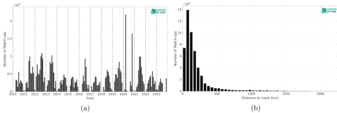
Figure 2: Number of match-ups between TSG (SAMOS) and SMOS SSS L3 v9 - 18 Days (CATDS-CEC-LOCEAN) SSS as a function of time (a) and as function of the distance to coast (b) over the Gulf Stream Pi-MEP region and for the full satellite product period.
