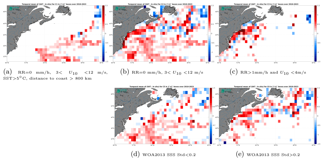
Figure 14: Temporal mean gridded over spatial boxes of size 1^\circ \times 1^\circ of \Delta SSS (SMOS SSS L3 v9 - 18 Days (CATDS-CEC-LOCEAN) - TSG (SAMOS)) for 5 different subdatasets corresponding to: RR=0 mm/h, 3 < U_{10} < 12 m/s, SST > 5°C, distance to coast > 800 km (a), RR=0 mm/h, 3 < U_{10} < 12 m/s (b), RR > 1mm/h and U_{10} < 4 m/s (c), WOA2013 SSS Std < 0.2 (d), WOA2013 SSS Std > 0.2 (e).
