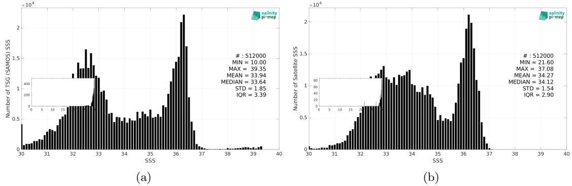
Figure 3: Histograms of SSS from TSG (SAMOS) (a) and SMOS SSS L3 v9 - 18 Days (CATDS-CEC-LOCEAN) (b) considering all match-up pairs per bins of 0.1 over the Gulf Stream Pi-MEP region and for the full satellite product period.
