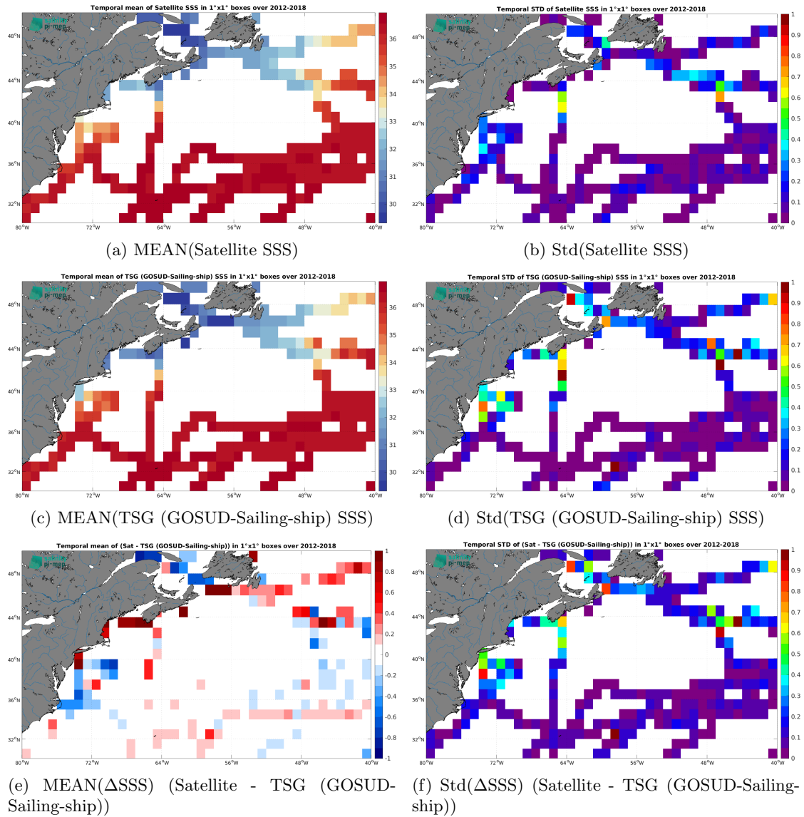
Figure 6: Temporal mean (left) and Std (right) of SSS from SMOS SSS L3 v9 - 18 Days (CATDS-CEC-LOCEAN) (top), TSG (GOSUD-Sailing-ship) (middle), and of \Delta SSS (Satellite - TSG (GOSUD-Sailing-ship)). Only match-up pairs are used to generate these maps.
