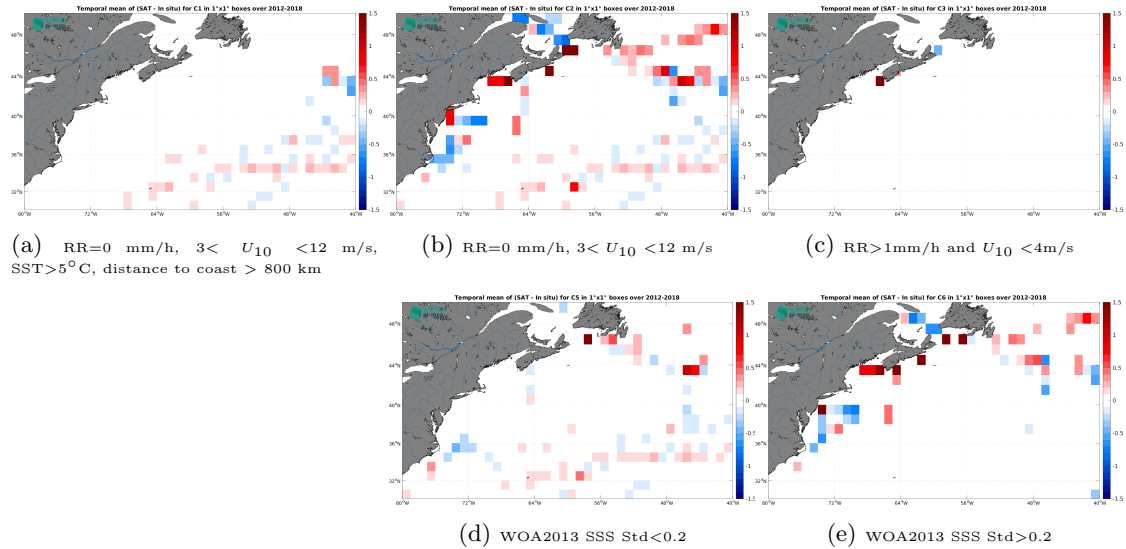
Figure 12: Temporal mean gridded over spatial boxes of size 1^{\circ}\times 1^{\circ} of \Delta SSS (SMOS SSS L3 v9 - 18 Days (CATDS-CEC-LOCEAN) - TSG (GOSUD-Sailing-ship)) for 5 different subdatasets corresponding to:RR=0 mm/h, 3 < U_{10} < 12 m/s, SST > 5^{\circ}\text{C} , distance to coast > 800 km (a), RR=0 mm/h, 3 < U_{10} < 12 m/s (b), RR > 1 mm/h and U_{10} < 4 m/s (c), WOA2013 SSS Std < 0.2 (d), WOA2013 SSS Std > 0.2 (e).
