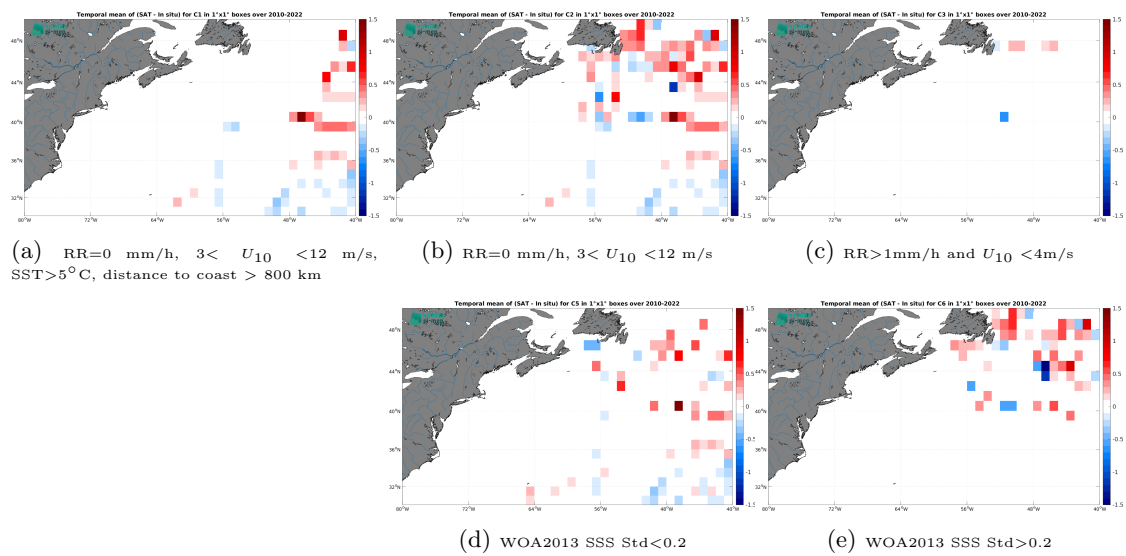
Figure 14: Temporal mean gridded over spatial boxes of size 1^\circ \times 1^\circ of \Delta\text{SSS} (SMOS SSS L3 v9 - 18 Days (CATDS-CEC-LOCEAN) - TSG (GOSUD-Research-vessel)) for 5 different subdatasets corresponding to:RR=0 mm/h, 3 < U_{10} < 12 m/s, SST >5^\circ\text{C} , distance to coast > 800 km (a), RR=0 mm/h, 3 < U_{10} < 12 m/s (b), RR >1 mm/h and U_{10} < 4 m/s (c), WOA2013 SSS Std <0.2 (d), WOA2013 SSS Std >0.2 (e).
